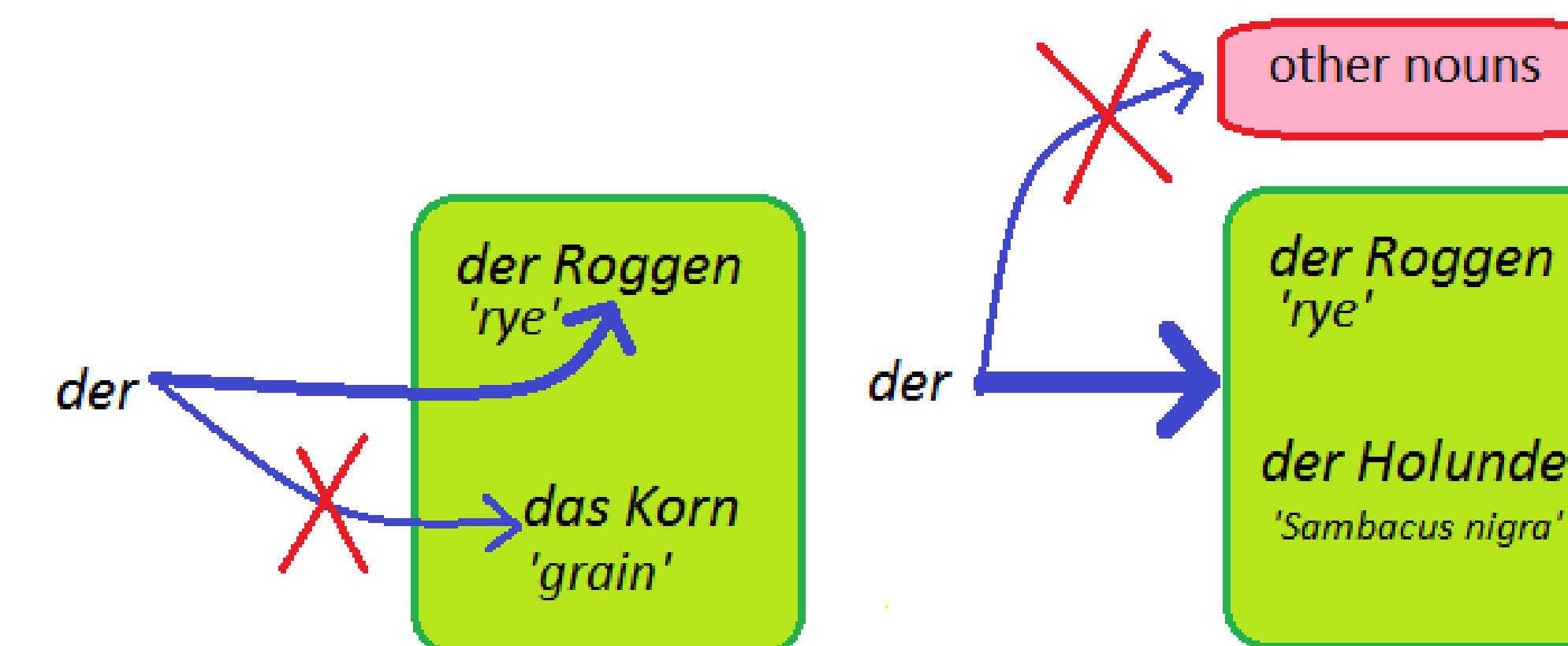
Figure 5. Gender may either discriminate between semantically similar nouns, or provide a cue for a semantic neighborhood.
