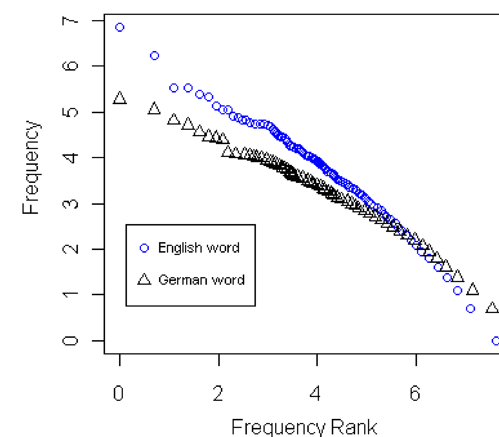
Figure 4. Frequency distribution of English and German lemmas in the context D-N.
