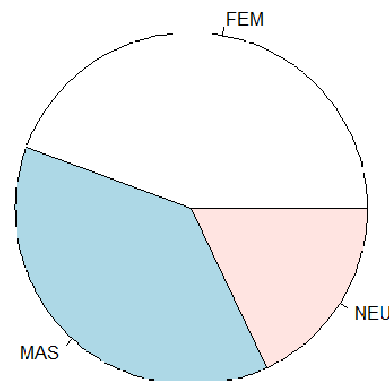
Figure 2. The distribution of the three genders by type in the German noun lexicon. For any two nouns, the baseline P(\text{Same gender}) = 0.36 .
