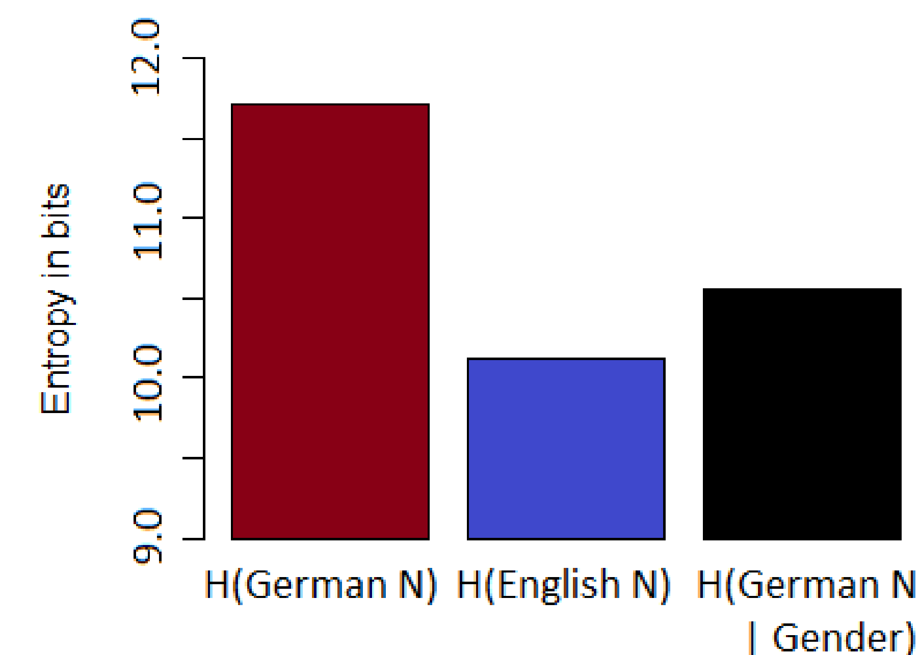
Figure 3. Entropy of German and English nouns after definite articles.
