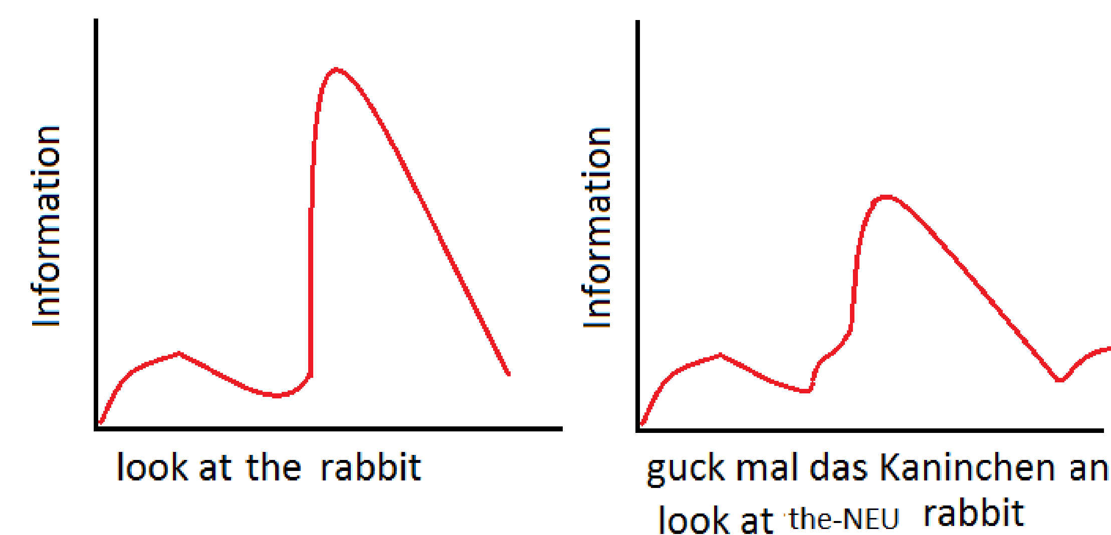
Figure 1. Hypothetical entropy rate without gender marking (English) and with it (German).
