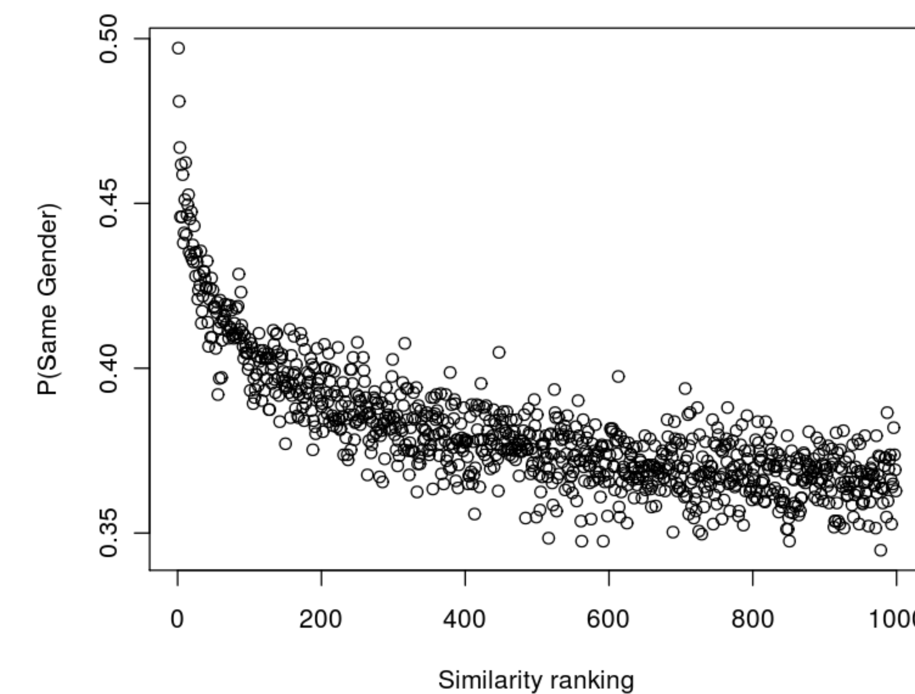
Figure 6. Probability that two nouns will share a gender based on their similarity ranking. The closest semantic neighbors (rank = 1) have just a 50% chance of sharing a gender.
