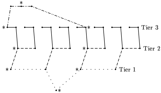
Figure 2.5: Parity-check tree
