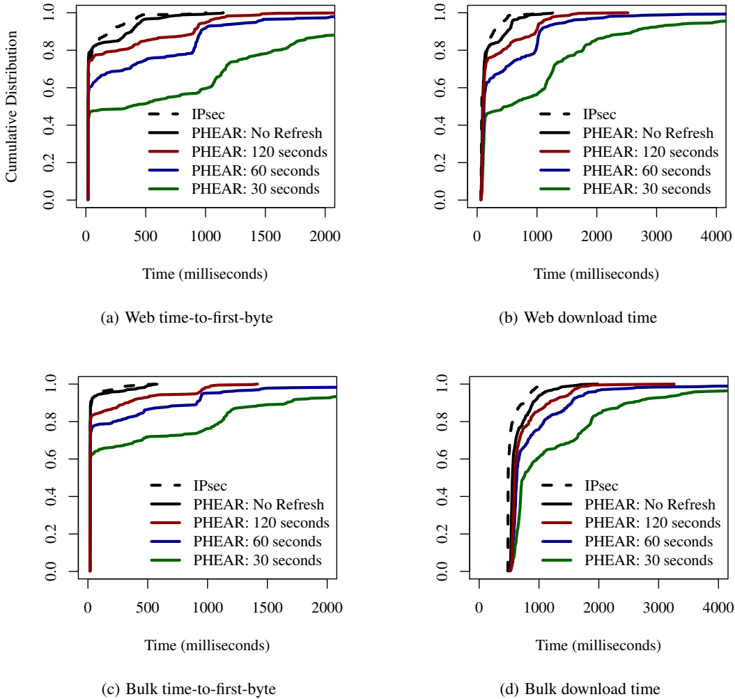
Figure 8: Whole-network performance results for the emulated web and bulk clients.
