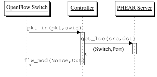
Figure 5: Nonce Lookup
