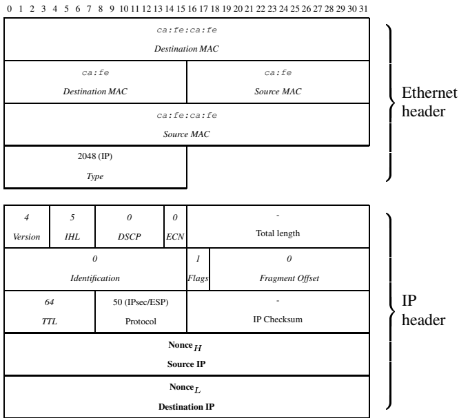
Figure 3: PHEAR Header
