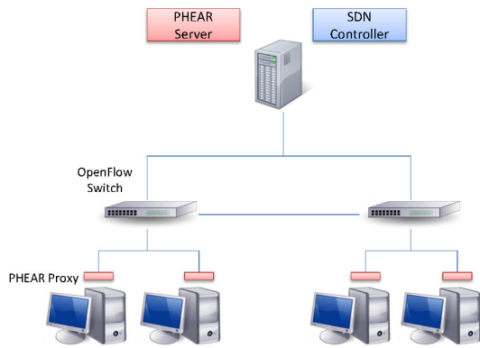
Figure 2: Packet Header Randomization Architecture
