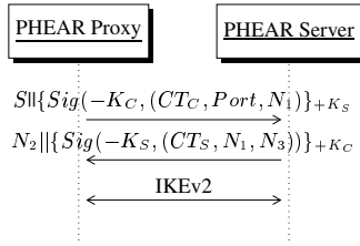
Figure 4: Client Registration
