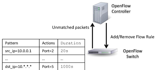
Figure 1: OpenFlow Architecture
