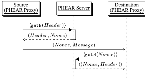
Figure 6: PHEAR Session Initiation
