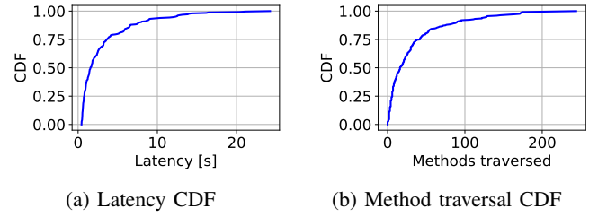
Fig. 7: Component analysis performance results.
