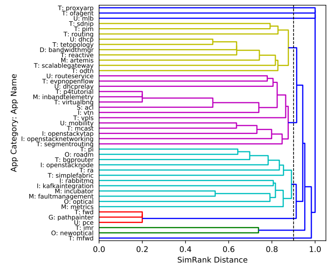
Fig. 5: Dendrogram representation of ONOS network event type similarity among apps, based on the SimRank distance metric. The dashed vertical line represents a threshold \tau = 0.90 with a partitioning of 9 clusters.
