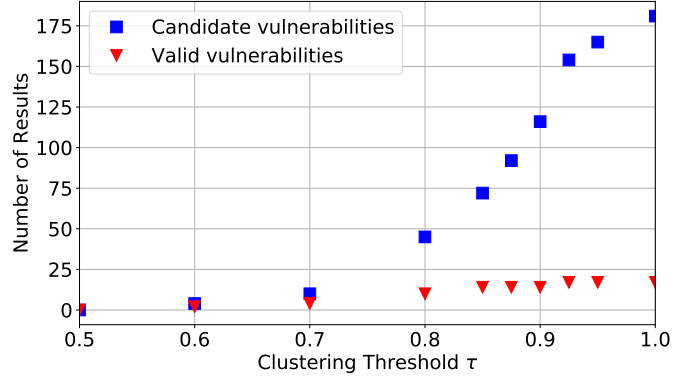
Fig. 12: ONOS apps' candidate and valid vulnerabilities as a function of clustering threshold \tau (using SimRank [24]).
