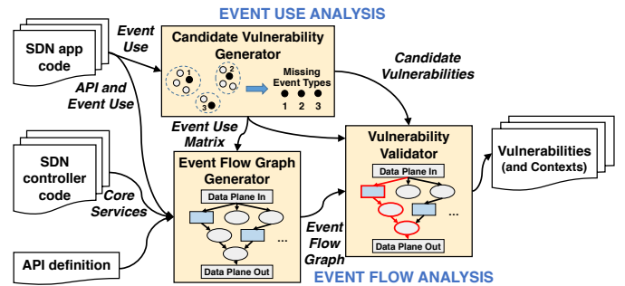
Fig. 3: EVENTSCOPE architecture overview.
