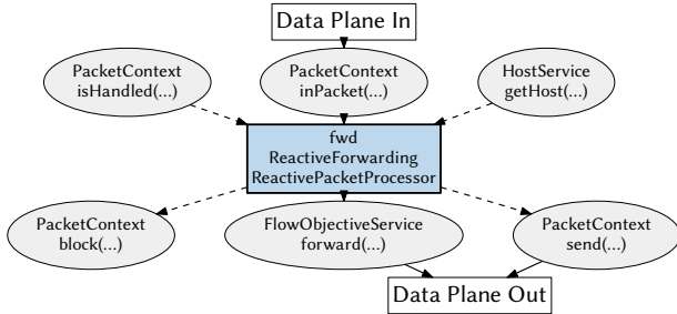
Fig. 6: Event flow graph of fwd 's packet processor. Blue rectangles represent event listeners and packet processors, gray ellipses represent API methods, and dashed edges represent API calls.
