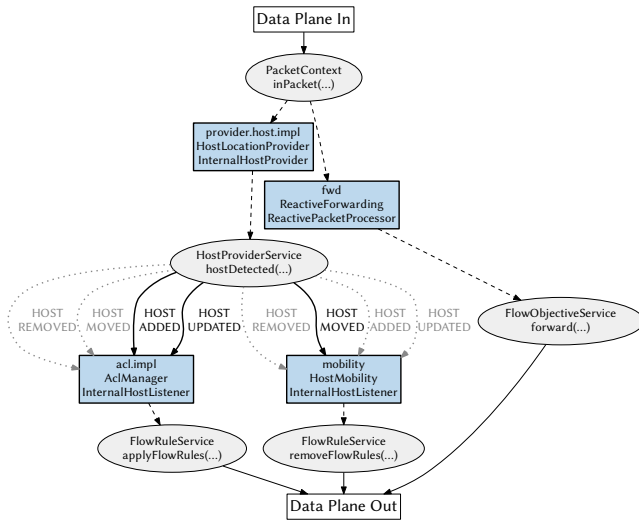
Fig. 9: Partial event flow graph showing vulnerable code paths used in CVE-2019-11189. Blue rectangles represent event listeners and packet processors, gray ellipses represent API methods, bold edges represent event dispatches, and dashed edges represent API calls. (Dotted gray edges represent unhandled event types, which are shown for reference.)
