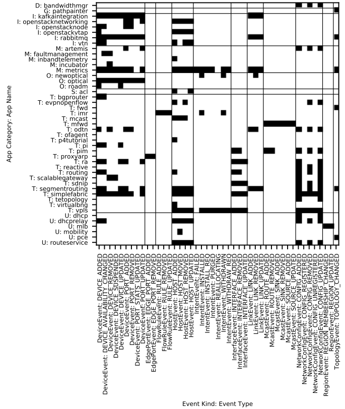
Fig. 4: ONOS event use matrix, M . Black cells represent event types that are handled by event() methods. Horizontal dividers represent app categories, and vertical dividers represent event kinds. (App category key: D = default, G = GUI, I = integration, M = monitoring, O = optical, S = security, T = traffic engineering, and U = utility.)
