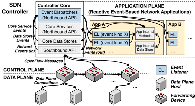
Fig. 1: SDN architecture overview. Apps subscribe to event dispatchers and implement event listeners. Network, data store, and service updates generate events.
