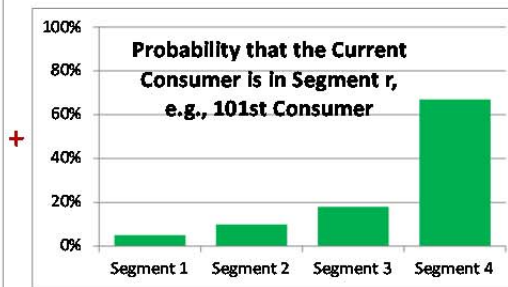
Posterior Probability that Current Consumer Belongs to Latent Segment r
