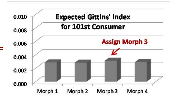
Expected Gittins' Index by Morph
