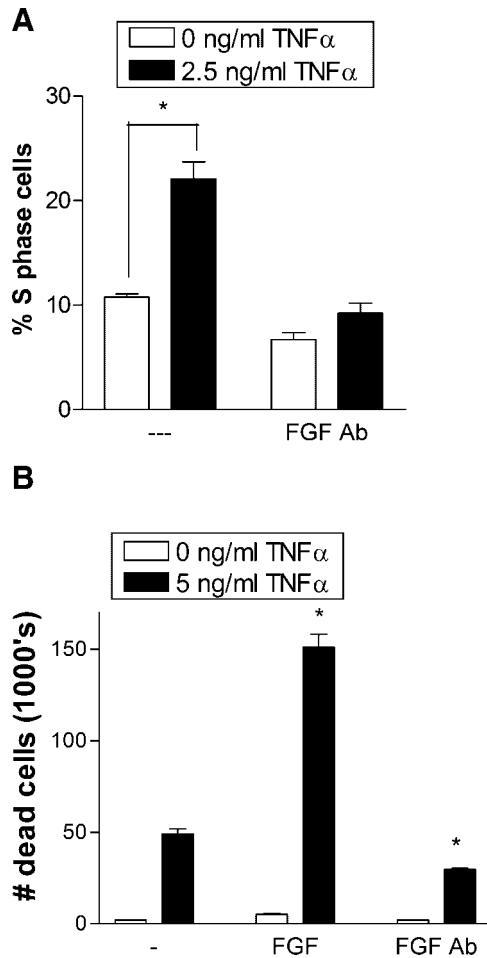
Fig. 5. An FGF-2 neutralizing antibody blocked TNF \alpha induced cell entry into S phase and decreases TNF \alpha apoptosis. A: Endothelial cells cultured in 5 mM glucose media with 0.5% FBS were given 2.5 ng/ml TNF \alpha . After 24 h, conditioned media was collected from these cells, concentrated by centrifugation, and 50 \mu l added to subconfluent, starved endothelial cells for 24 h. Cells were then harvested and prepared for cell cycle flow cytometry. B: Endothelial cells cultured in 5 mM glucose were given 10 ng/ml FGF-2 or 1 \mu g/ml neutralizing FGF-2 antibody. After 48 h, cells were given 5 ng/ml TNF \alpha . Floating dead cells were counted 24 h after TNF \alpha addition. Data shown is one representative experiment of three, n = 3 . * P < 0.01 .
