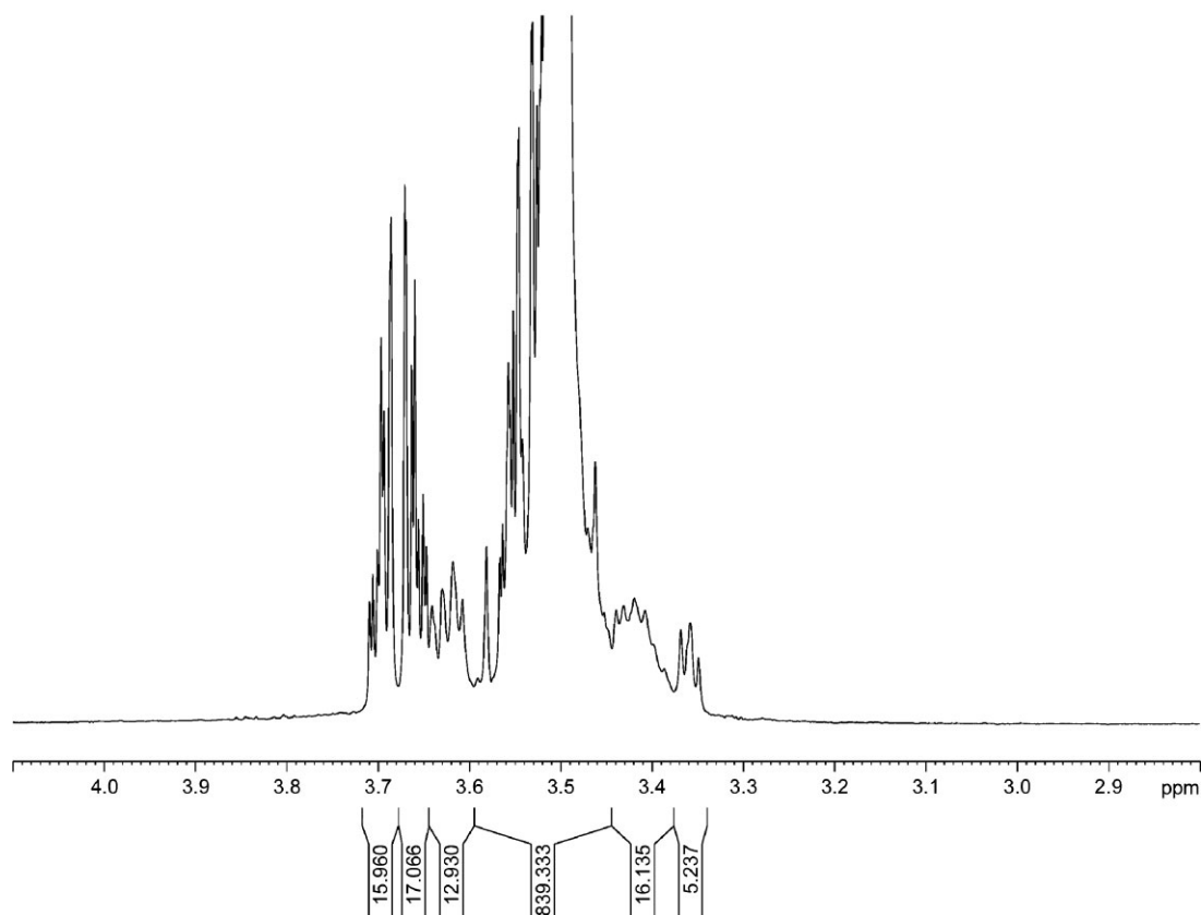
■ Figure A1. 1 H NMR of PEG chloride showing a peak at \delta = 3.72\text{--}3.68 (m, 2H, CH 2 Cl).
