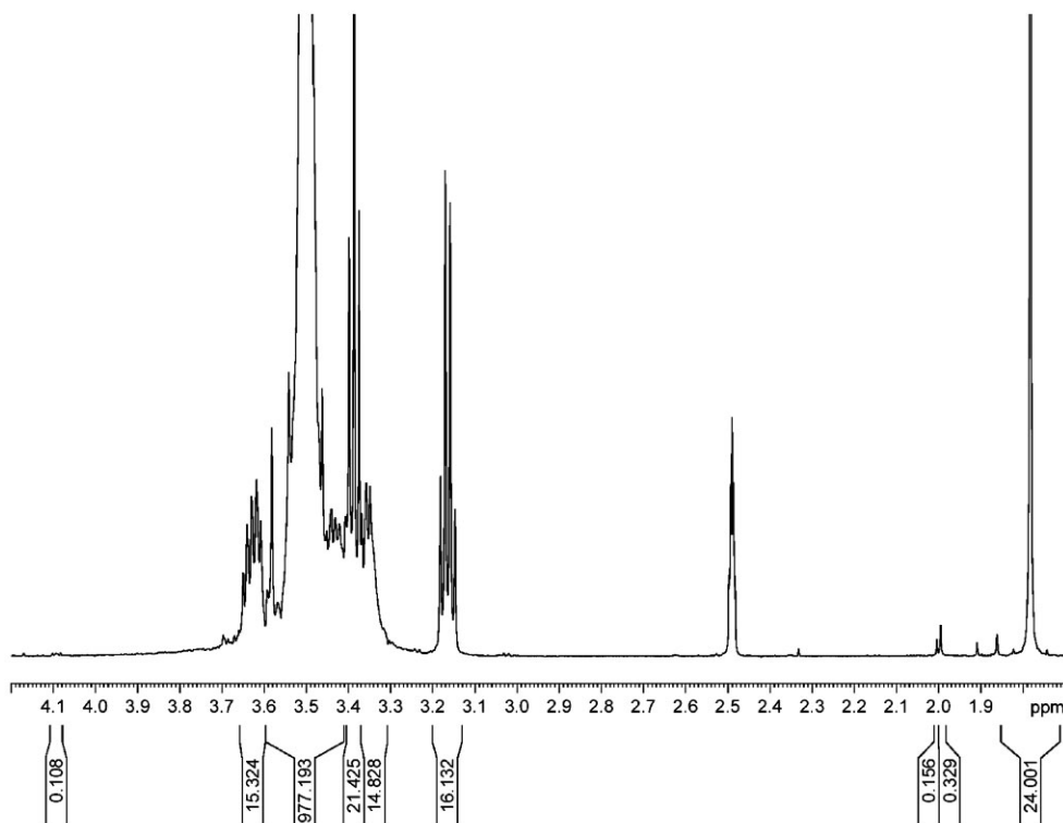
Figure A4. ^1\text{H} NMR of acetylated PEG amine showing peaks at \delta = 4.09 (t, J = 4.7 Hz, 2H, \text{CH}_2\text{OAc} ), 3.16 (q, J = 5.8 Hz, 2H, \text{CH}_2\text{N} ), \delta = 2.00 (s, 3H, AcO) and 1.78 (s, 3H, AcN).
