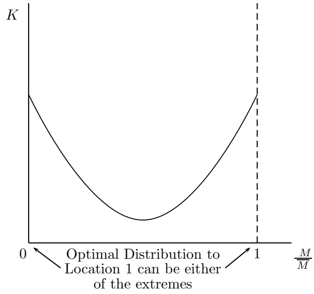
Figure 4: Optimal Distribution ( \beta_3 > 0 )
