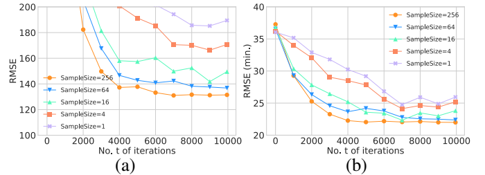
Fig. 4. Graphs of RMSEs of VBPC+ vs. number t of iterations with varying sampling sizes for computing its predictive mean for the (a) TWITTER and (b) AIRLINE datasets.
