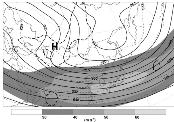
FIG. 6. As in Fig. 3, but for the Siberian composite.
