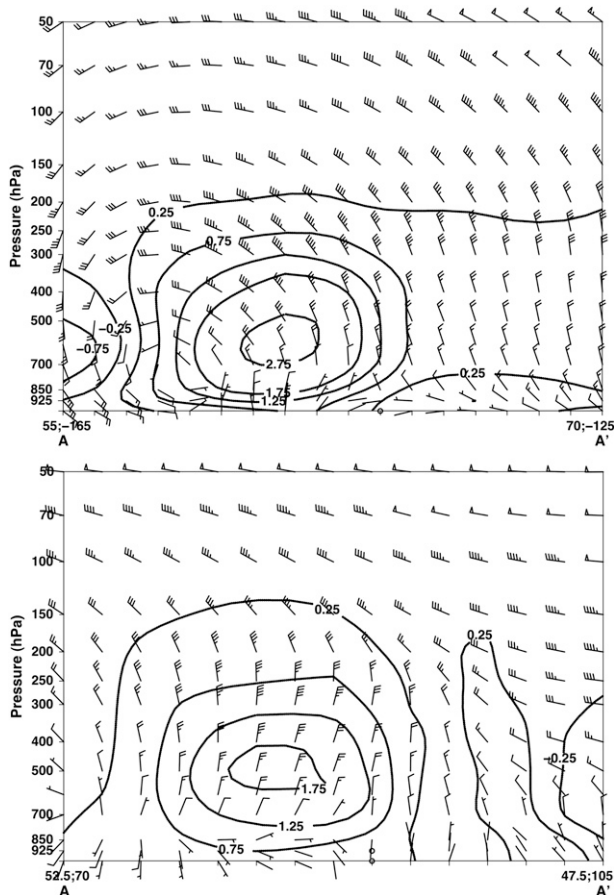
FIG. 10. Vertical cross sections of \omega (solid contours, \times 10^{-3} hPa s ^{-1} ) and winds (m s ^{-1} ) at t = -1 day for the (top) Alaskan composite and (bottom) Siberian composite.
