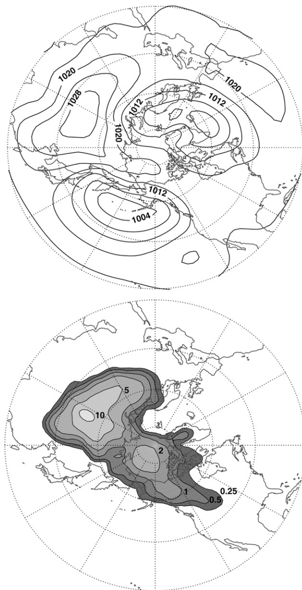
FIG. 1. (top) Mean November–March SLP for the period 1957–2002 and (bottom) annual frequency of observed SLP values greater than or equal to 1050 hPa.
