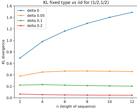
Fig. 3. This plot demonstrates the consequences of Theorem 2. We numerically compute D(P_{\hat{Y}^n} \| P_{Y^n}) when P = (1/2, 1/2) and P_{Y|X} is given as in (4) for different values of \delta . When \delta = 0 , we see that the KL divergence is trending towards infinity (specifically it grows as \frac{1}{2} \log n ). When any noise is added ( \delta is positive), this growth to infinity completely disappears. The quantity D(P_{\hat{Y}^n} \| P_{Y^n}) becomes constant in n , as Theorem 2 states.
