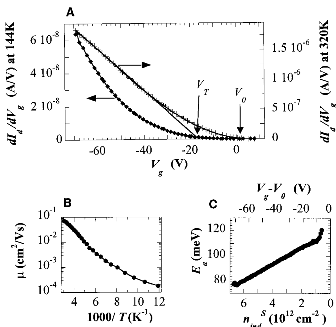
Fig. 4. (A) Transconductance dI_d/dV_g in the saturation regime ( L = 75 \mu\text{m} , W = 1500 \mu\text{m} , V_{\text{sd}} = -70 V) at 320 K (crosses) and 144 K (squares). (B) Field-effect mobility at n_{\text{ind}}^s = 6 \times 10^{12} \text{cm}^{-2} as a function of temperature between 330 and 84 K. (C) Activation energy E_a of the mobility extracted between 300 and 160 K as a function of n_{\text{ind}}^s \approx C_i/e(V_g - V_0) .
