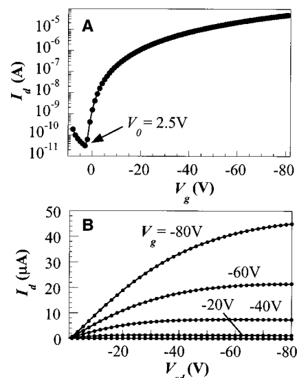
Fig. 3. (A) Transfer characteristics in the saturation regime ( v_{sd} = -80 V) and (B) output characteristics of a typical P3HT FET ( L = 75 \mu\text{m} , W = 1500 \mu\text{m} ).
