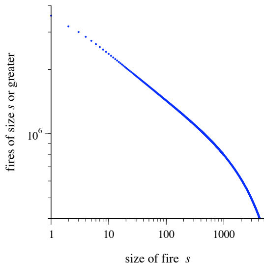
FIG. 16 Cumulative distribution of the sizes of “fires” in a simulation of the forest fire model of Drossel and Schwabl [59] for a square lattice of size 5000 \times 5000 .
