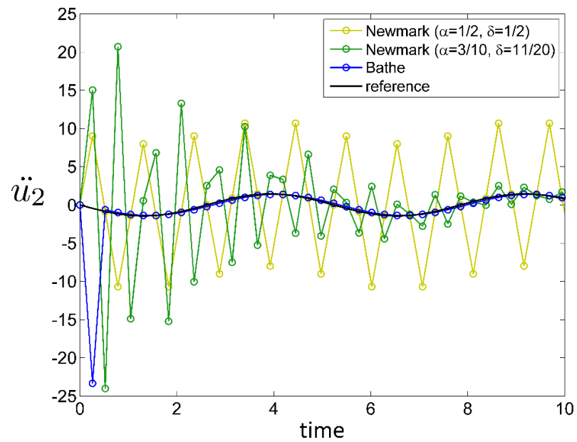
(f) Acceleration of node 2 for various methods, not using the Trapezoidal Rule. For the first step in the Bathe method, the overshoot is eliminated with good results throughout if we use only for the first sub-step of the first time step, \alpha = 1 ; \delta = 3/4 .
