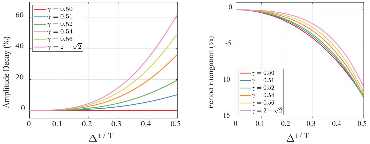
Fig. 4.2 Percentage amplitude decay and period elongation of Noh-Bathe explicit time integration.
