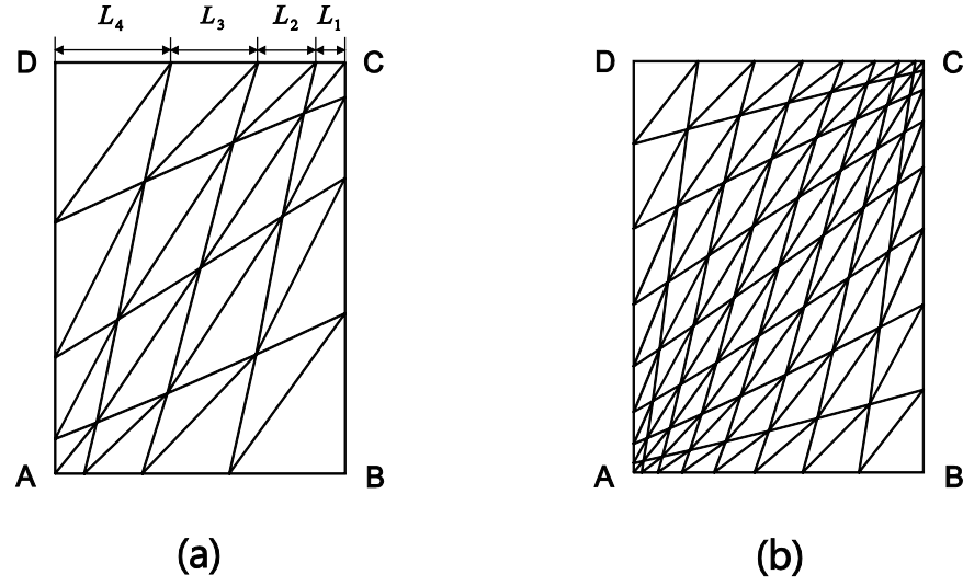
Fig. 2.25. Distorted mesh patterns (a) for N = 4 and (b) for N = 8 .
