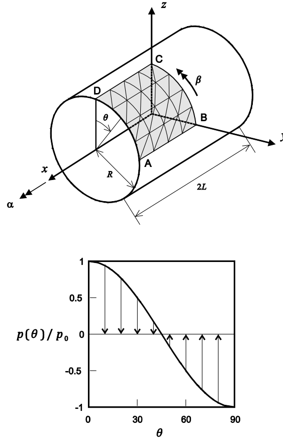
Fig. 2.22. Cylindrical shell problem ( 4 \times 4 mesh, L = R = 1.0 , E = 2.0 \times 10^5 , \nu = 1/3 and p_0 = 1.0 )
