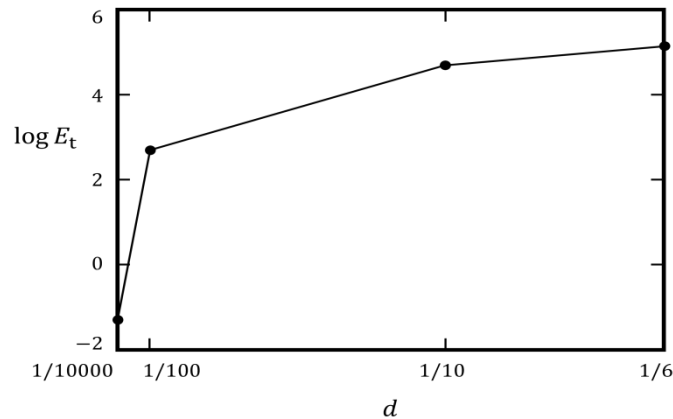
Fig. 2.19 Strain energy in twisting mode as a function of distance d in Fig. 2.1.
