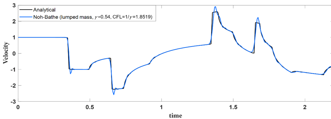
(a) using the Noh-Bathe method, \gamma = 0.54 , \text{CFL} = 1.8519
