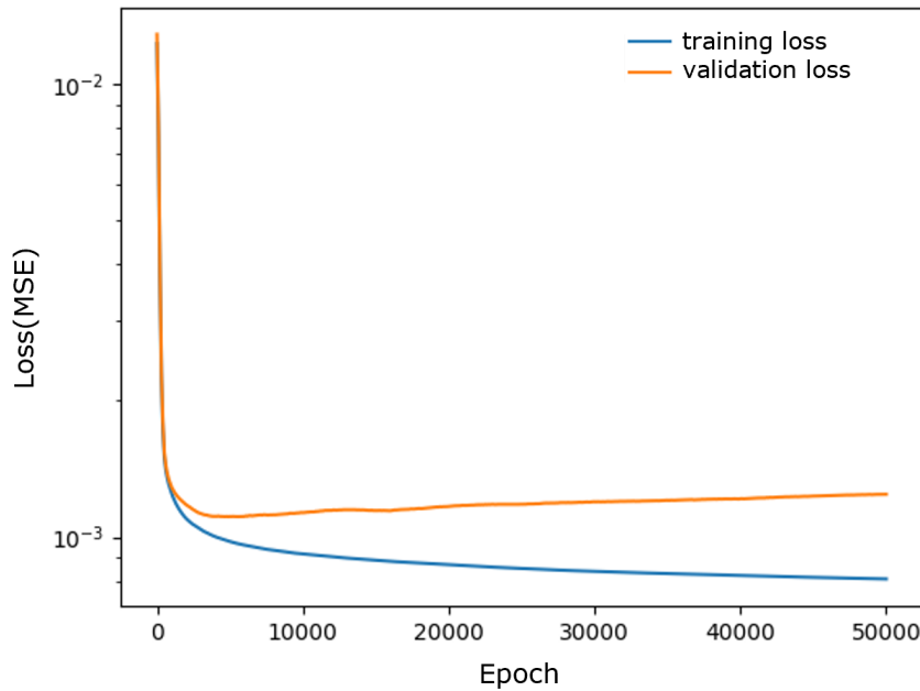
Fig. 6.10 Loss in training and validation of the example considered
