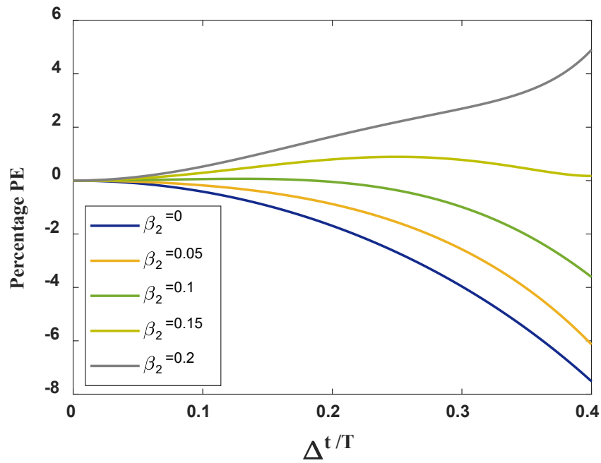
(b) Period elongation of the explicit \beta_1/\beta_2 -Bathe method second-order scheme, \beta_1 = 0.5 , with \xi = 0.0
