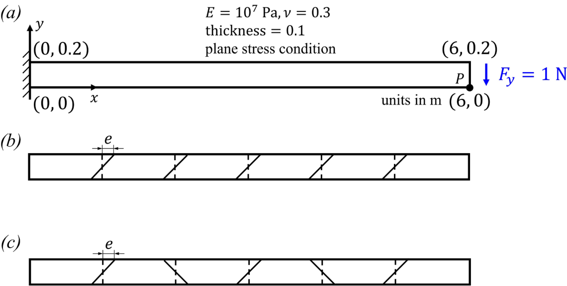
Fig. 3.9 Thin beam problem; (a) Description of the bending problem; total applied force is 1 N; (b) Parallelogram mesh used; (c) Trapezoidal mesh used.
