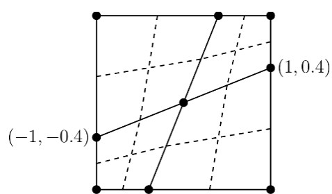
c) Distorted mesh
