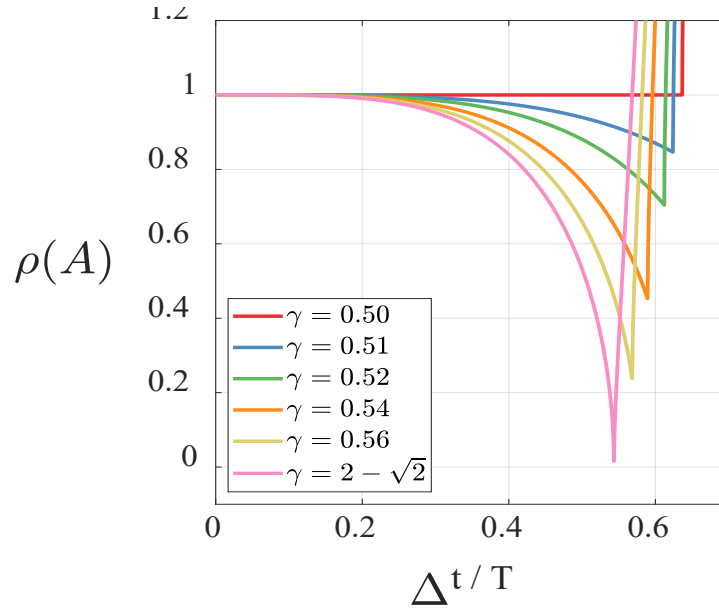
Fig. 4.1 Spectral radius of Noh-Bathe explicit time integration scheme, with \xi = 0.0 , G. Noh and K.J. Bathe [A].
