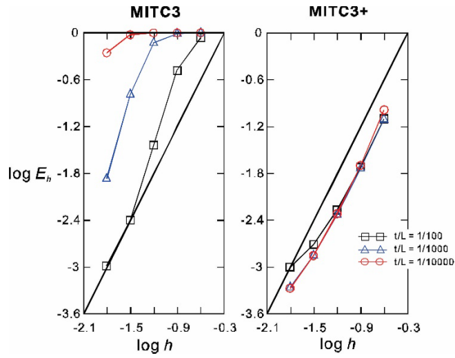
Fig. 2.30 Convergence curves for the free hyperboloid shell problem using non-distorted meshes.
