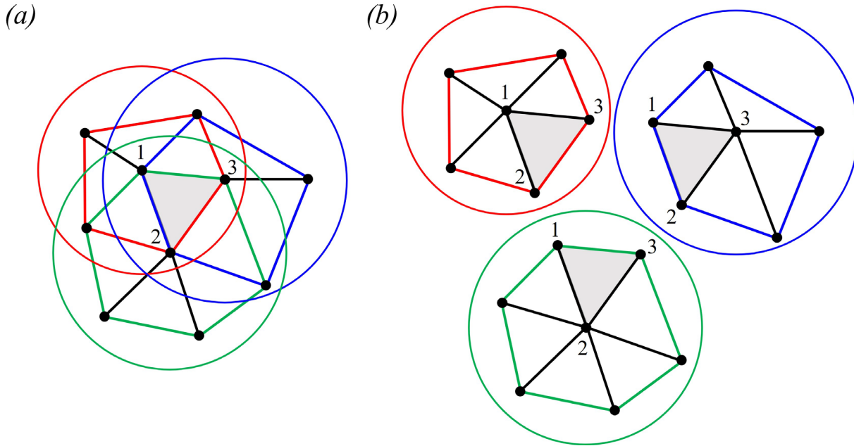
Fig. 3.1 (a) A triangular overlapping finite element with nodes 1, 2, and 3; (b) the overlapping finite element corresponds to the overlapped region of the three polygonal elements with center nodes 1, 2, and 3; the circles indicate the corresponding finite disks for the overlapping finite element. Regarding Figs. 3.1 to 3.3 and more discussion, see S. Lee and K.J. Bathe [A].
