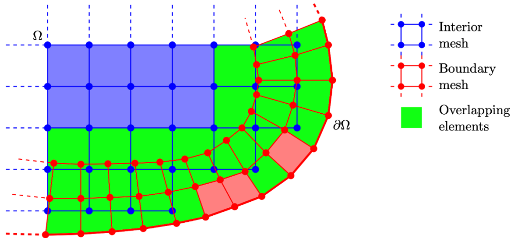
Fig. 3.33 Illustration of two overlapping meshes. Regarding Figs. 3.33 to 3.38 and a further discussion, see J. Huang and K.J. Bathe [B].
