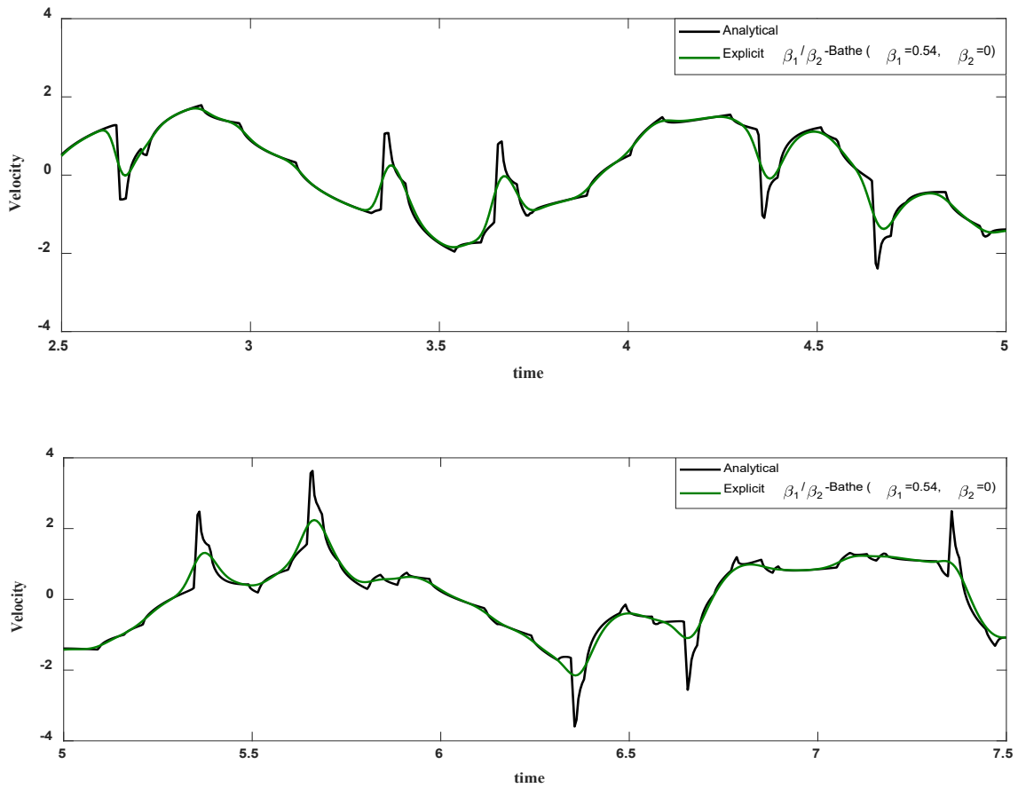
Fig. 4.17 Predicted longtime velocity using the explicit \beta_1/\beta_2 -Bathe method with CFL = 1.925.
