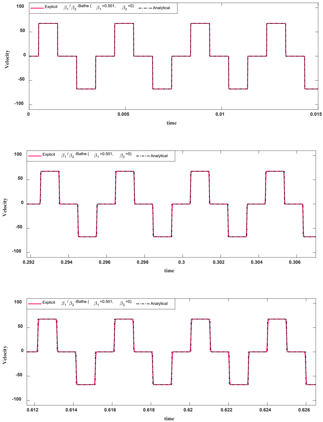
Fig. 4.11 Predicted velocity at the mid-point of the bar, CFL = 1.998
