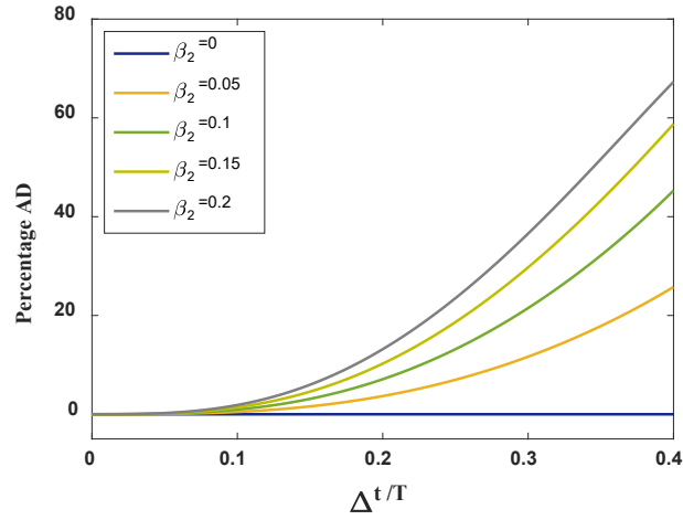
(a) Amplitude decay of the explicit \beta_1/\beta_2 -Bathe method; second-order scheme \beta_1 = 0.5 , with \xi = 0.0
