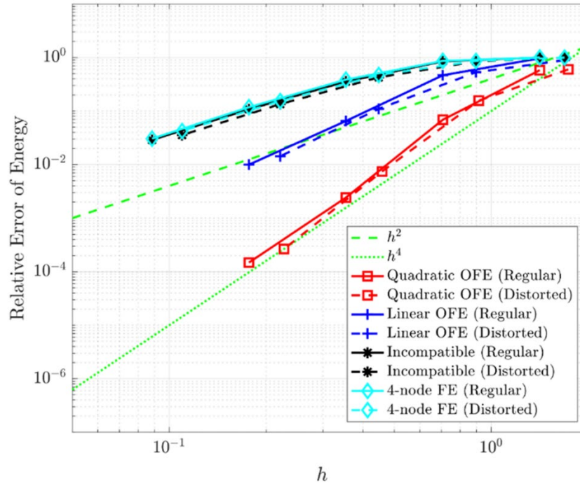
Fig. 3.11 The convergence rates for the ad-hoc example problem
