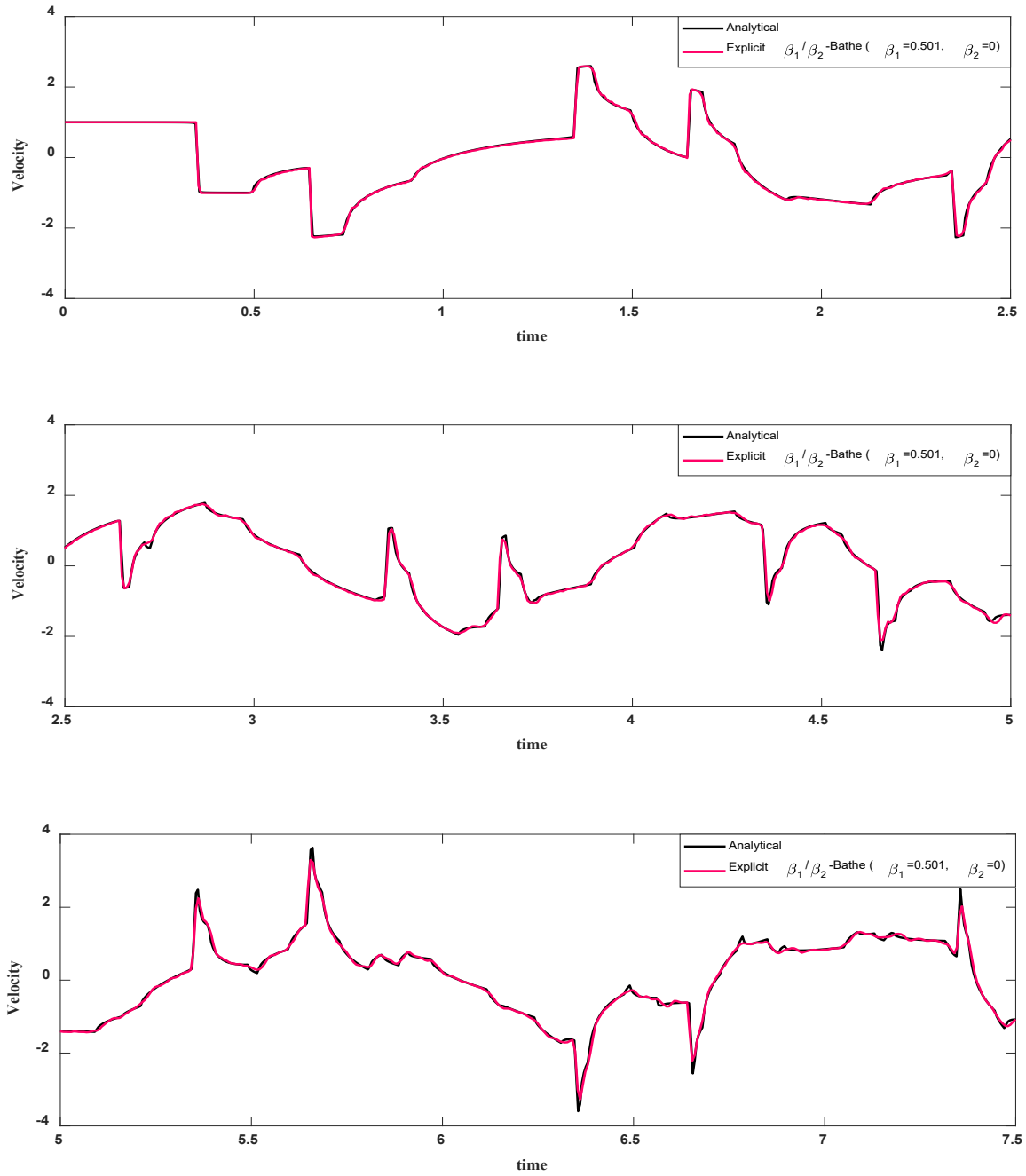
Fig.4.18 Predicted longtime velocity using the explicit \beta_1/\beta_2 -Bathe method, CFL = 1.998
