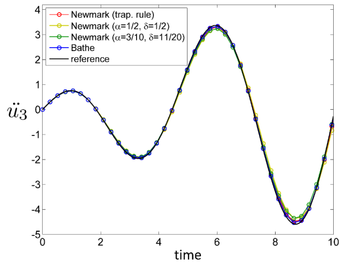
(g) Acceleration of node 3 for various methods.
