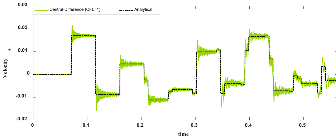
Fig. 4.13 Solution using the central difference method with CFL = 1
