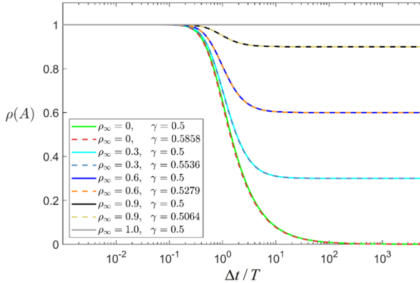
(a) Spectral radius
