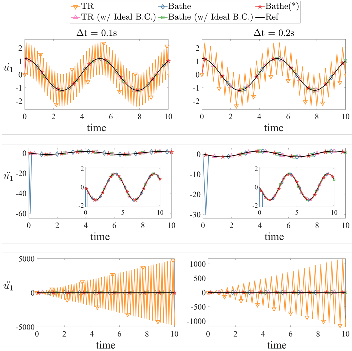
Fig. 4.24 Predictions of velocity and acceleration at node 1; “Bathe(*)” uses \alpha=1 and \delta=3/4 only for the first step, and \alpha=1/4 and \delta=1/2 otherwise; the results of the computed acceleration for “TR” are shown separately due to the different scale.
