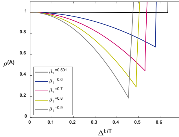
Fig. 4.4 Spectral radius of the explicit \beta_1/\beta_2 -Bathe method; first-order scheme, \beta_2 = 0 , with \xi = 0.0 . Regarding Figs. 4.4 to 4.8 and more information, see M.M. Malakiyeh, S. Shojaee, S. Hamzehei-Javaran and K.J.Bathe [A] and M. M. Malakiyeh, Z. Anjomshoe, S. Shojaee, S.Hamzehei-Javaran and K.J. Bathe [A].
