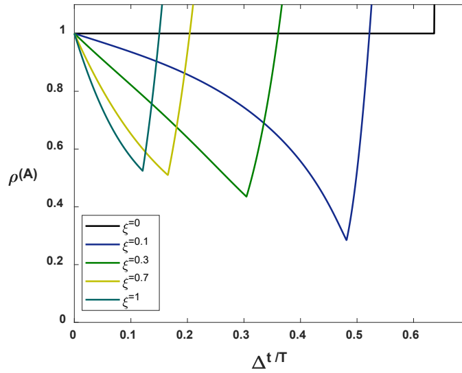
Fig. 4.8 Spectral radius of the explicit \beta_1/\beta_2 -Bathe method in the presence of physical damping ( \xi \geq 0.0 ) for \beta_1 = 0.5 and \beta_2 = 0
