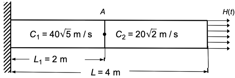
Fig. 3.14 An elastic bi-material bar impacted by a unit step axial pressure. Regarding Figs. 3.14 to 3.20 and further information, see K.T. Kim and K.J. Bathe [B].
