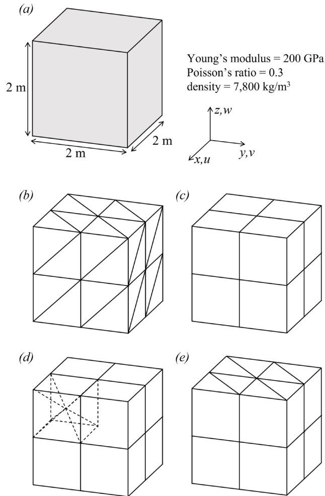
Fig. 3.12 Free vibration analysis of an unsupported cube; (a) Description of the analysis domain; (b) Mesh using tetrahedral elements; (c) using brick elements; (d) using pyramid elements; as shown, a set of six pyramid elements forms a sub-hexahedral domain; (e) Mesh using prism elements; All shown meshes correspond to N = 2 where N is the number of elements per side of the analysis domain.
