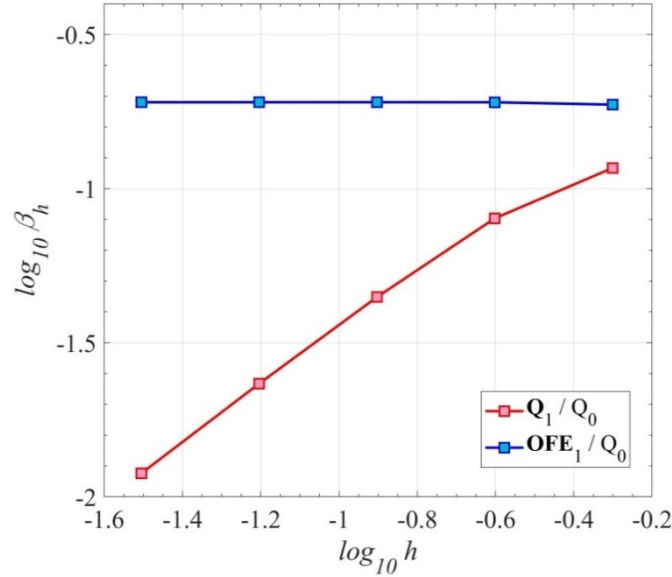
Fig. 3.24 Inf-sup test results for the traditional Q_1/Q_0 element and the OFE_1/Q_0 element when the meshes are undistorted.
