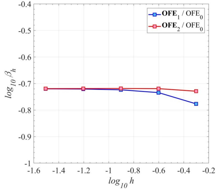
Fig. 3.25 Inf-sup test results for the OFE_1/OFE_0 and OFE_2/OFE_0 elements, when the meshes are undistorted.
