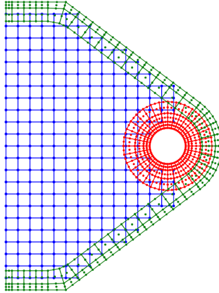
(c) Overlapping finite element meshes
