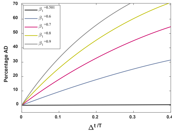
(a) Amplitude decay of the explicit \beta_1/\beta_2 -Bathe method; first-order scheme, \beta_2 = 0 , with \xi = 0.0
