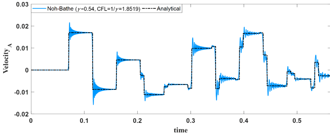
Fig. 4.14 (a) Solution using the Noh-Bathe method with CFL = 1.8519
