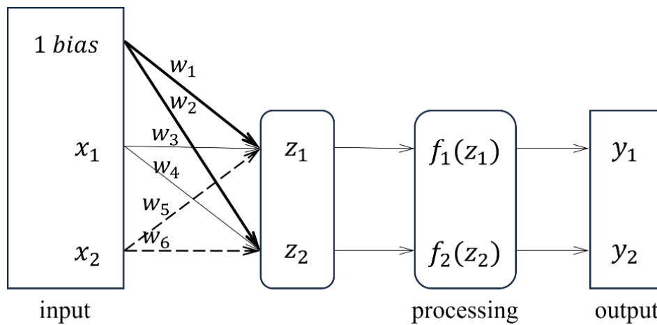
Fig. 6.2 A simple NN with an input layer of x_1 , x_2 and the bias b = 1.0 , with two nodes in the processing layer
