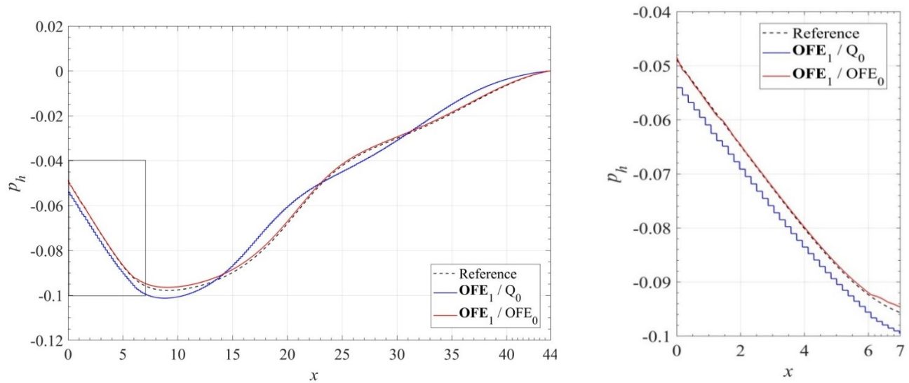
Fig. 3.32 Predicted pressure along the top wall of the channel; on the right, the solutions in the box indicated in the left figure are enlarged.
