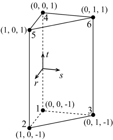
Fig. 3.6 Reference element for the geometry interpolation of the prism overlapping element.
