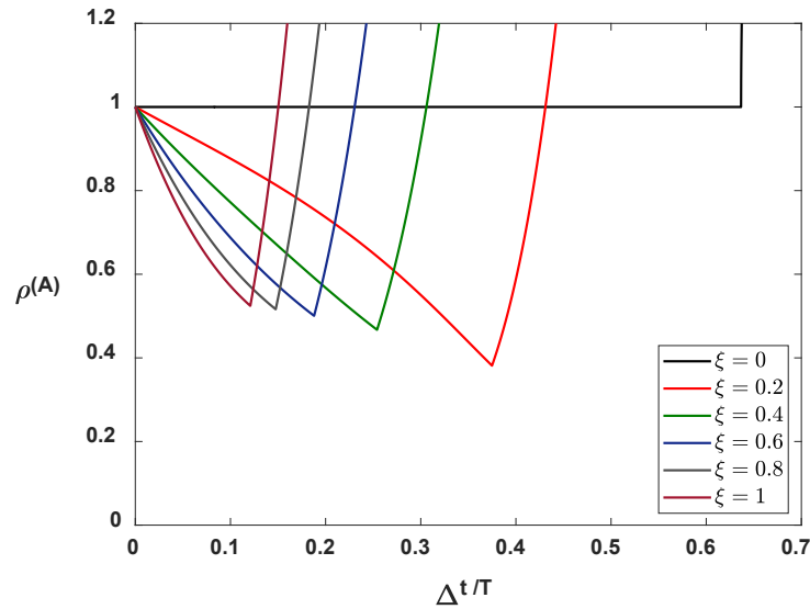
Fig. 4.3 The effect of physical damping ( \xi \geq 0.0 ) on the spectral radius when \gamma = 0.5 .
