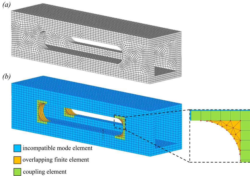
Fig. 3.43 For the tool jig; (a) The traditional mesh using the incompatible mode element; (b) The AMORE mesh using the 6-node prism overlapping element with the linear basis and \beta = 0.01 ; the 8-node coupling element is used.
