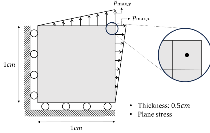
Fig. 6.5 Two-dimensional specimen used to generate the training, validation and test data
