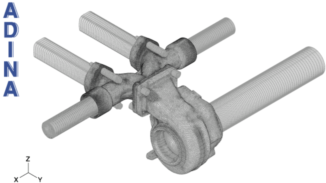
Fig. 5.5 The model of the manifold exhaust solved for its lowest (nonzero) frequencies
