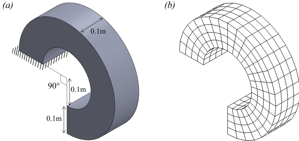
Fig. 3.13 A three-dimensional slender ring; Young's modulus = 200 GPa, Poisson's ratio = 0.3, density = 7,800 kg/m 3 ; (a) The ring (b) The mesh using m = 4 , S. Lee and K.J. Bathe [B].
