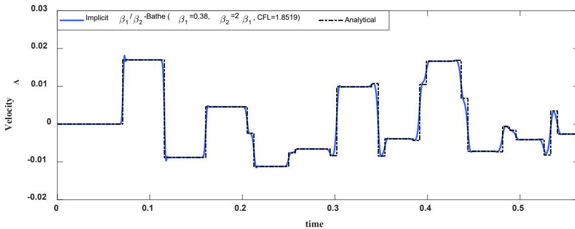
Fig. 4.27 Predicted velocity using the implicit \beta_1 / \beta_2 -Bathe method at point A in the rod (see Fig. 4.7), M.M. Malakiyeh, S. Shojaee, S. Hamzehei-Javaran and K.J.Bathe [A].
