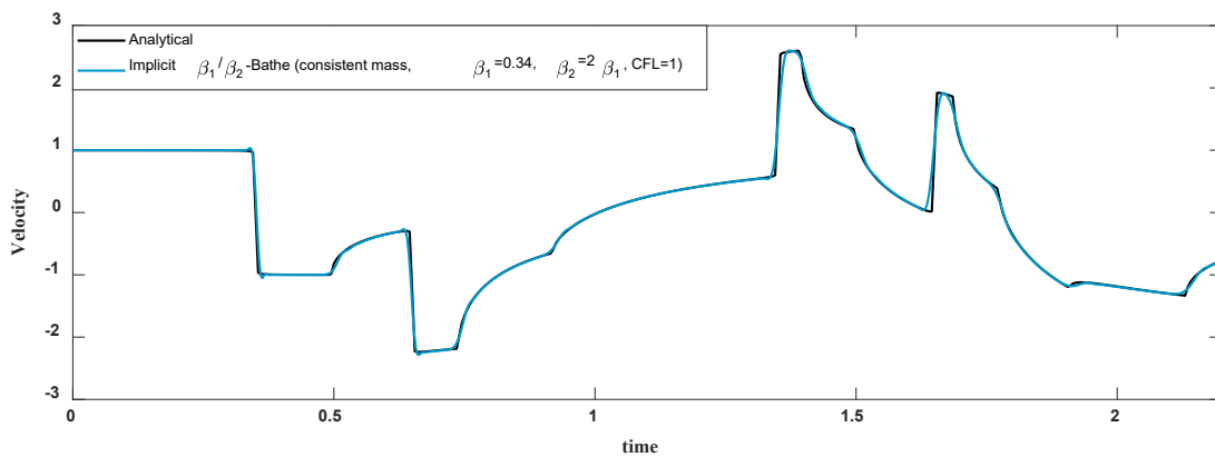
Fig. 4.28 Predicted velocity at center point using the implicit \beta_1/\beta_2 -Bathe method, consistent mass matrix, CFL = 1, \gamma = 0.5 , M.M. Malakiyeh, S. Shojaee, S. Hamzehei-Javaran and K.J. Bathe [A].
