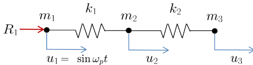
Fig. 4.20 Model problem of three degrees of freedom spring system,
