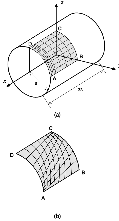
Fig. 2.35 Cylindrical shell for the inf-sup testing ( L = R = 1.0 , t = 1/10 , 1/100 , 1/1000 or 1/10000 , E = 1.0 and \nu = 0.0 ). (a) Problem description with the graded regular mesh ( 8 \times 8 elements). (b) A distorted mesh used ( 8 \times 8 elements). Regarding Figs.2.35 to 2.38 and more discussion, see Y. Ko and K.J. Bathe [B].
