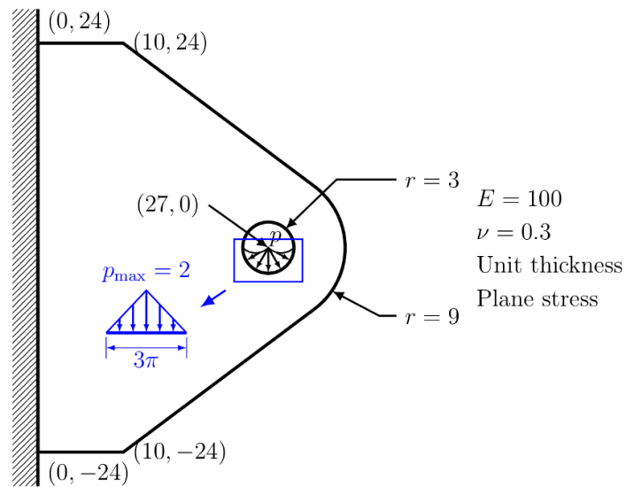
Fig. 3.39 The bracket problem, K.J. Bathe [D]
