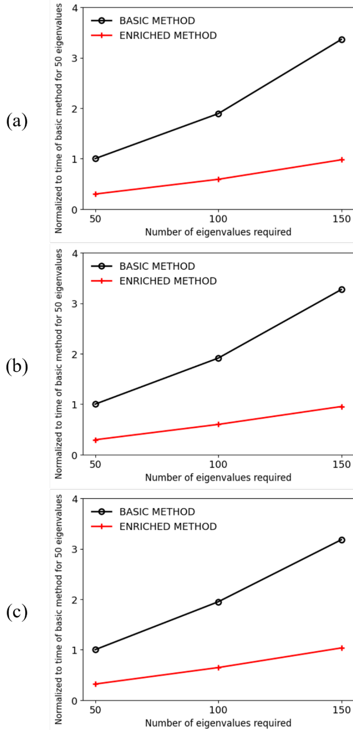
Fig. 5.4 Solution times solving the ring problem of Fig. 5.3, all times are normalized to the time used for the problem for p=50 ; (a) n = 216,000, m = 675 ; (b) n = 389,880, m = 1,083 ; (c) n = 603,060, m = 1,587
