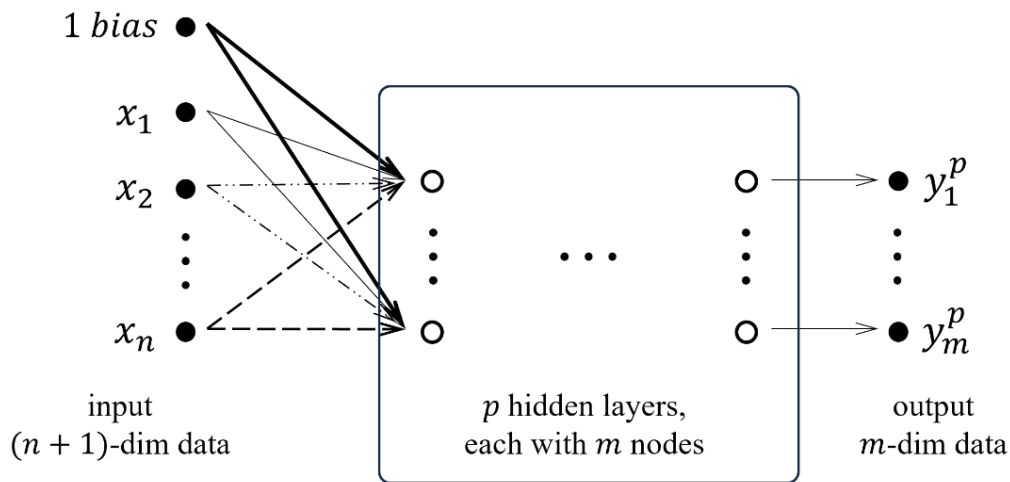
Fig. 6.3 A deep NN with p hidden layers, each layer has m nodes, but different numbers of nodes in the layers may also be used
