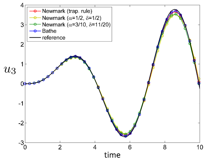
(b) Displacement of node 3 for various methods
