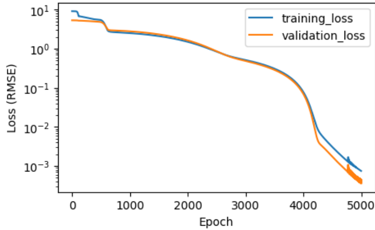
Fig. 6.7 Training and validation loss in the evaluation of the material behavior of the specimen of Fig. 6.5
