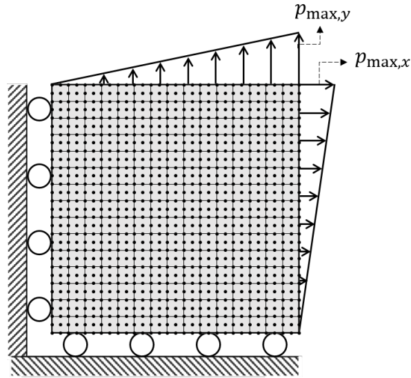
(a) The specimen in its original configuration with the displacement boundary conditions and (b) the loading in the x- and y-directions
