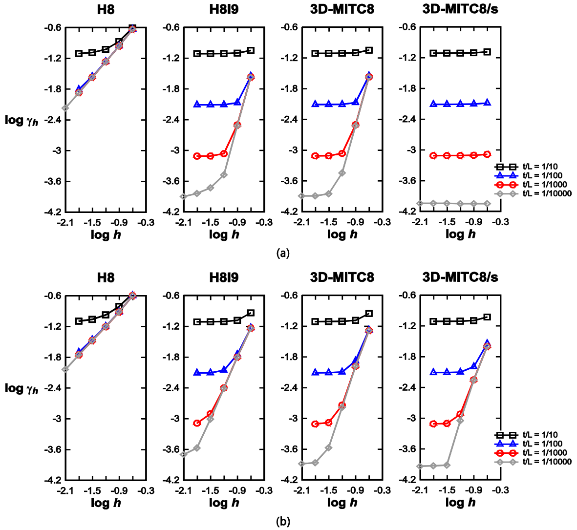
Fig. 2.36 Inf-sup convergence curves for the cylindrical shell using (a) regular and (b) distorted meshes.
