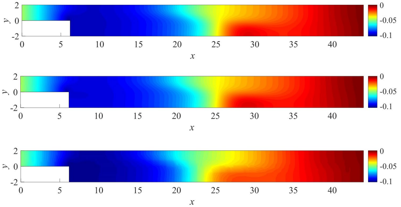
Fig. 3.30 Predicted pressure at Re = 250 ; top: reference solution using the Q_2/Q_1 element; middle: solution using the OFE_1/OFE_0 element; bottom: solution using the OFE_1/Q_0 element.
