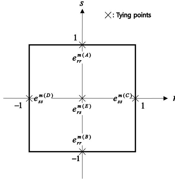
Fig. 2.4. Tying positions (A), (B), (C), (D) and (E) for the assumed mid-surface membrane strains. Note that in comparison to Fig. 2.2, the position (E) is also used.
