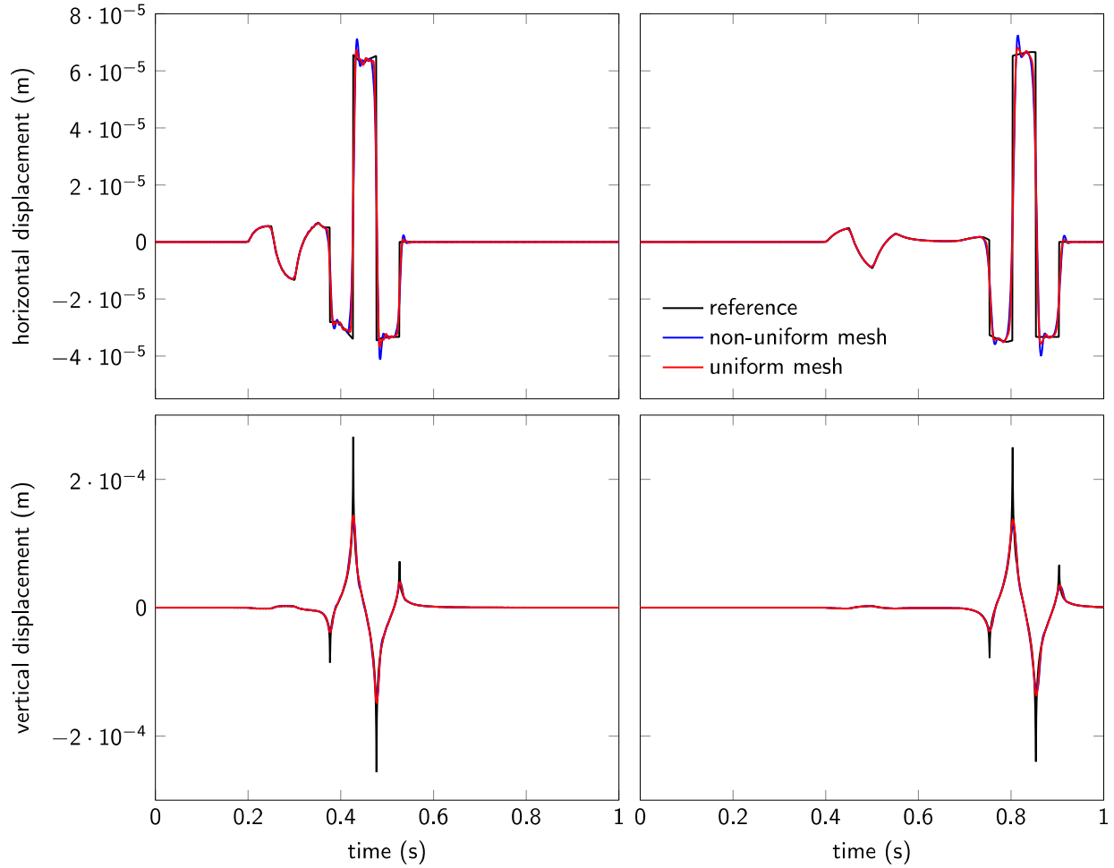
Fig. 3.17 Horizontal and vertical displacements of the elastic medium subjected to the step loading on the free surface. The time histories of the displacements at \mathbf{x} = (640,0) (left) and at \mathbf{x} = (1280,0) (right) are shown. The OFE-TRI2 with uniform and non-uniform meshes (51,200 elements and 30,446 elements, respectively) and the \beta_1/\beta_2 -Bathe method ( \gamma = 0.5 and \beta_1 = 0.35 with \beta_2 = 2\beta_1 ) with CFL=0.125 are used. The analytical reference solution is based on the work in J. Miklowitz [A].
