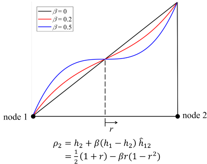
Fig. 3.2 Interpolation function for node 2 of overlapping 2-node element
