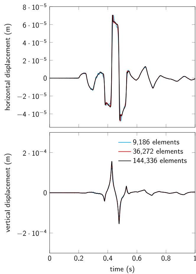
Fig. 3.19 Horizontal and vertical displacements of the two-layered elastic medium with a crack
