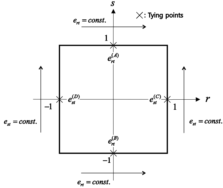
Fig. 2.2 The tying positions (A), (B), (C) and (D) for the assumed transverse shear strain field of the MITC4 and MITC4+ shell elements. The constant transverse shear strain conditions are imposed along the element edges, K.J. Bathe [A]
