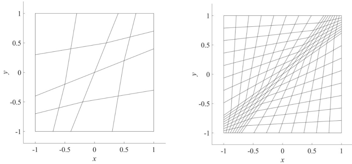
Fig 3.26 The original undistorted mesh, N=2 , and distorted N=2 and N=4 element meshes for \Delta=0.4 , and distorted N=16 element mesh for \Delta=0.7 . To reach the 4 \times 4 element mesh, that is, N=4 , the elements in the distorted 2 \times 2 element mesh are each subdivided into 4 elements. The finer meshes are similarly reached.
