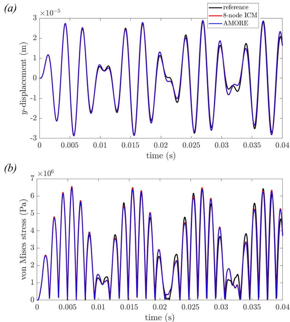
Fig. 3.44 Numerical predictions at point P , see Fig. 3.42; (a) the y -displacement; (b) the von Mises stress.
