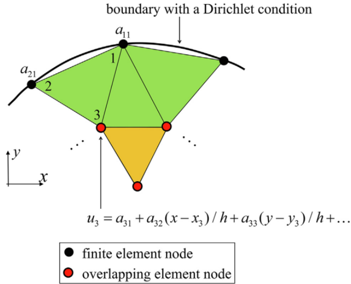
Fig. 3.8 Coupling element used to impose displacement boundary condition
