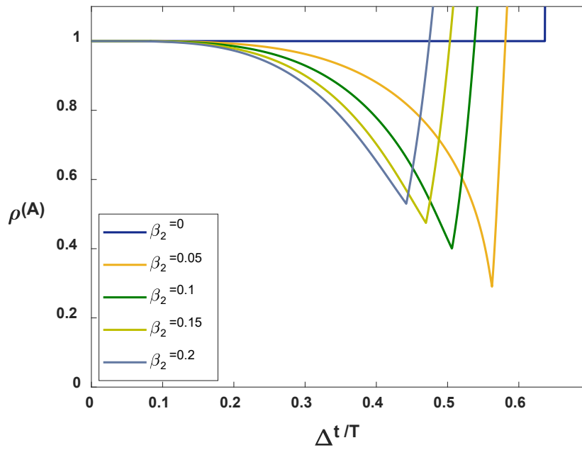
Fig. 4.6 Spectral radius of the explicit \beta_1/\beta_2 -Bathe method; second-order scheme, \beta_1 = 0.5 , with \xi = 0.0
