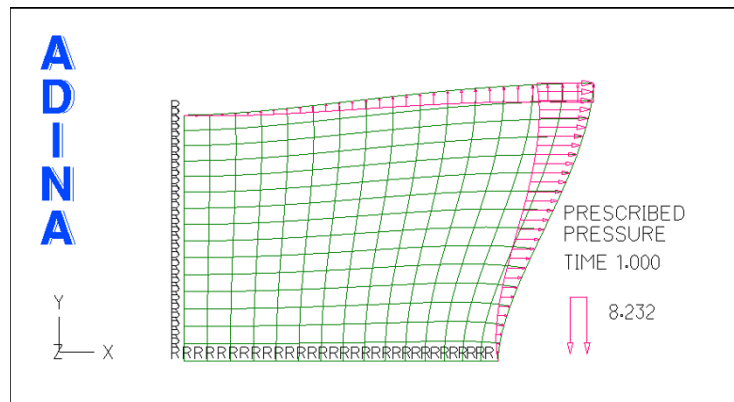
(b) A typical deformed configuration reached, notice that the applied horizontal pressure is larger than the vertical pressure; the roller supports are shown by the “R”
