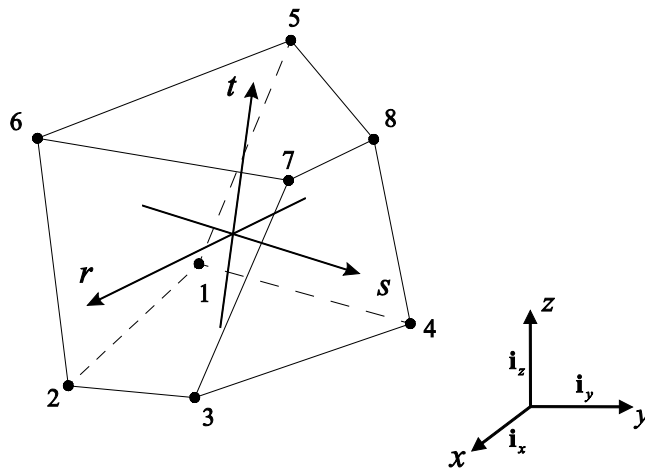
Fig. 2.33 A standard 8-node hexahedral three-dimensional solid element, Y. Ko and K.J. Bathe [A].
