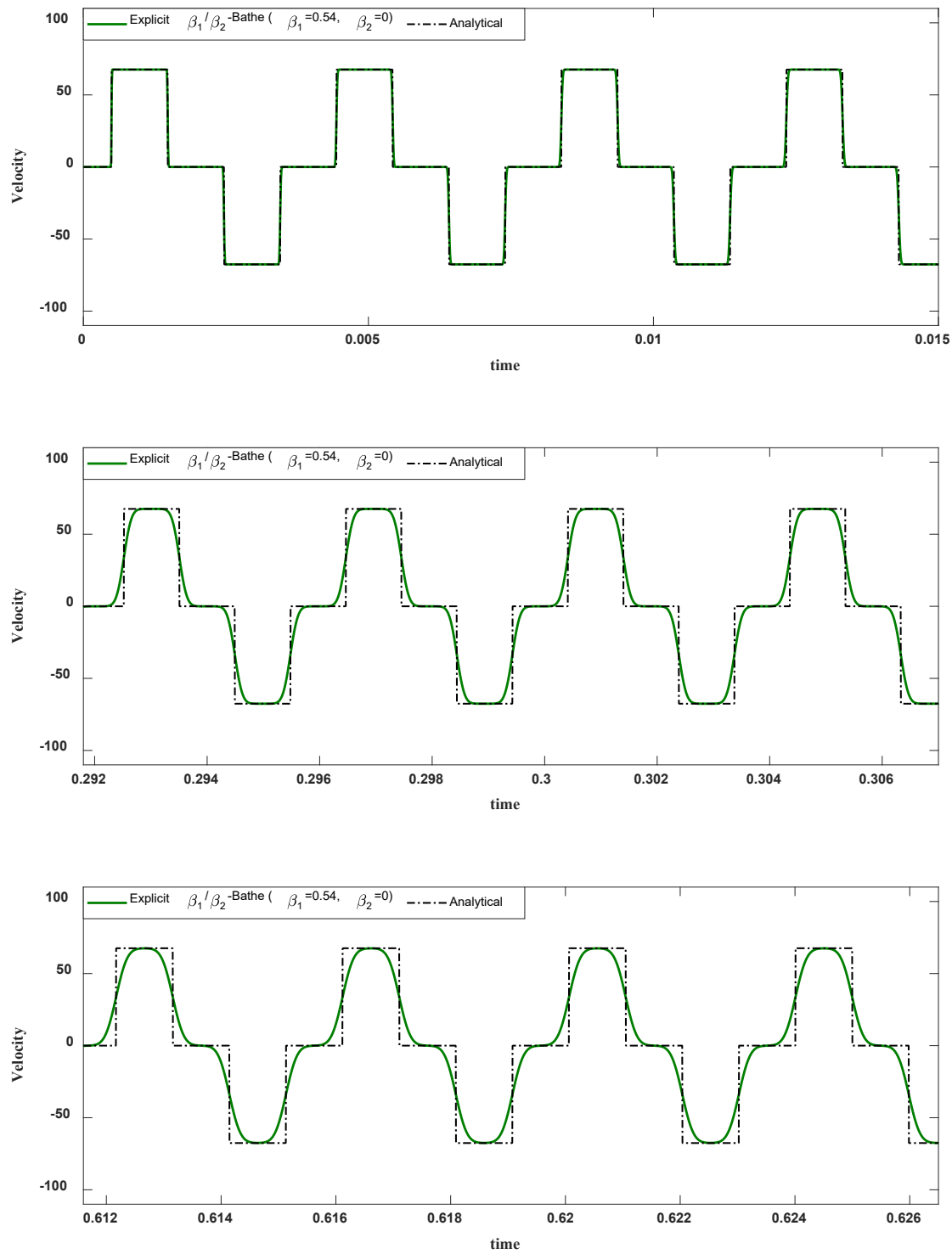
Fig.. 4.10 Predicted velocity at the mid-point of the bar, CFL = 1.925
