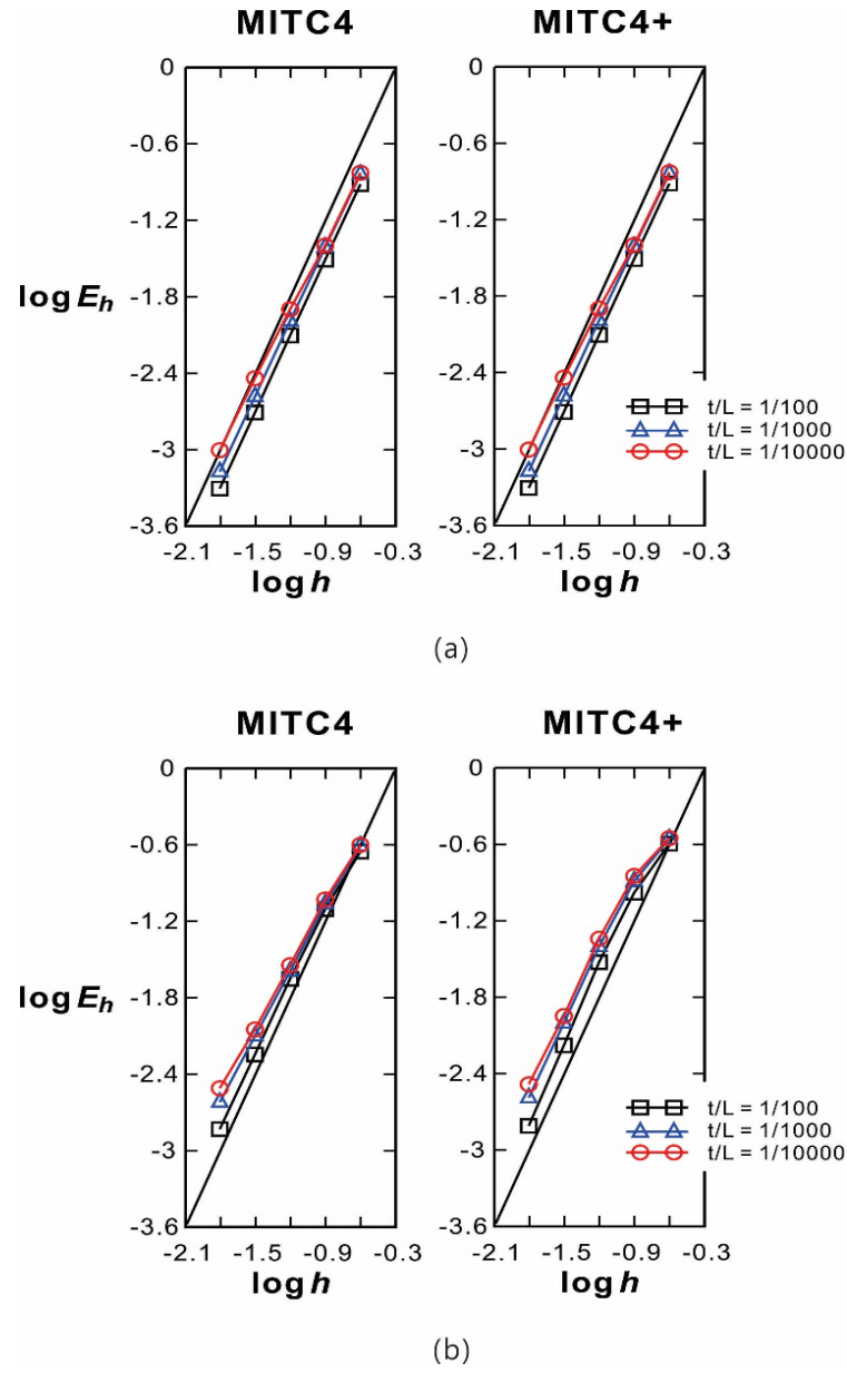
Fig. 2.10 Convergence curves for the clamped cylindrical shell problem with (a) the graded regular or (b) distorted meshes.
