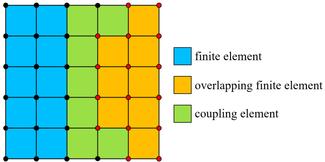
Fig. 3.7 Coupling elements for transitioning from traditional to overlapping elements
