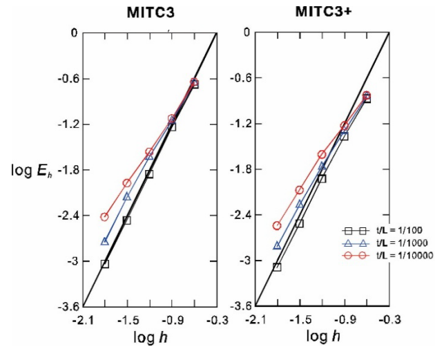
Fig. 2.23. Convergence curves for the clamped cylindrical shell problem using non-distorted meshes
