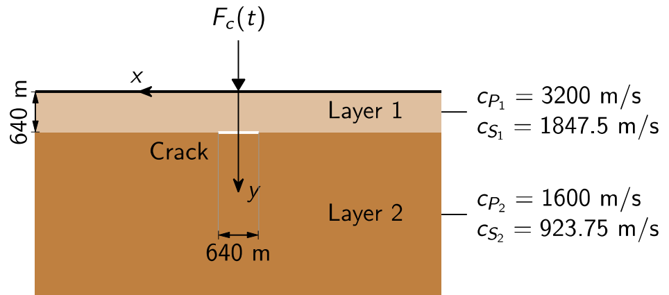
Fig. 3.18 A semi-infinite medium consisting of two elastic layers with a crack in plane strain conditions; a concentrated line load is applied on the free surface.
