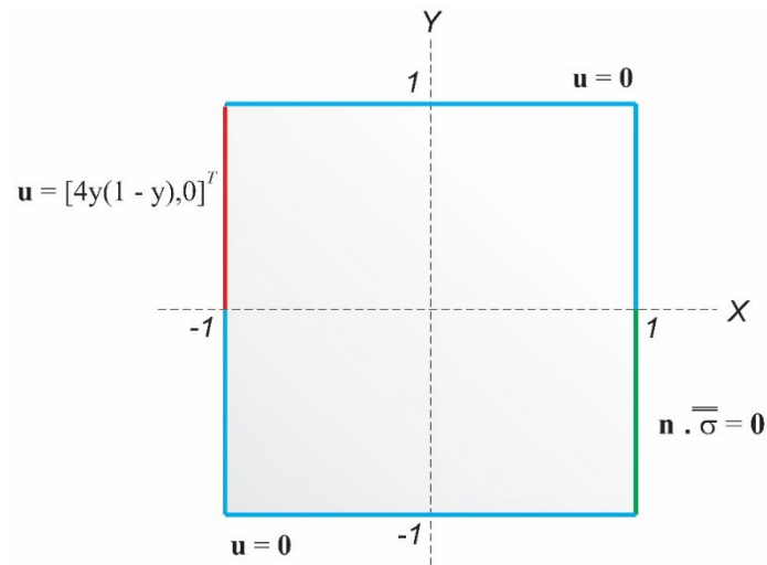
Fig. 3.21 Fluid flow problem with in-flow condition on the boundary marked red, out-flow condition on boundary marked green and the no-slip condition on the boundary marked blue.
