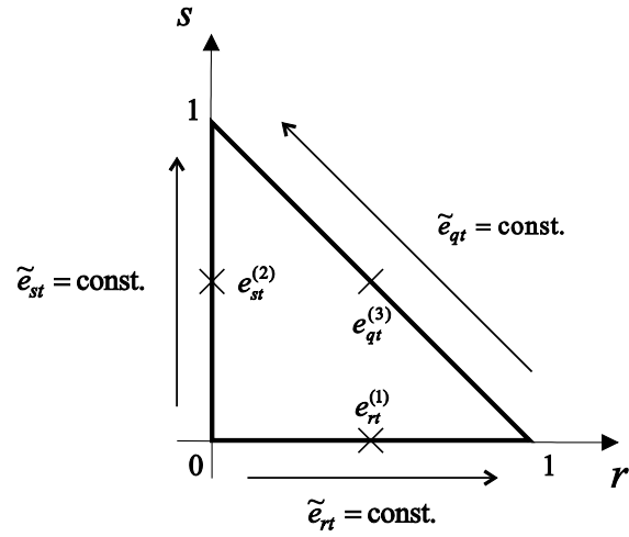
Fig. 2.16 Tying positions for the assumed transverse shear strain field of the MITC3 shell element. Along the edges, constant transverse shear strain conditions are imposed, P.S. Lee and K.J. Bathe [D].
