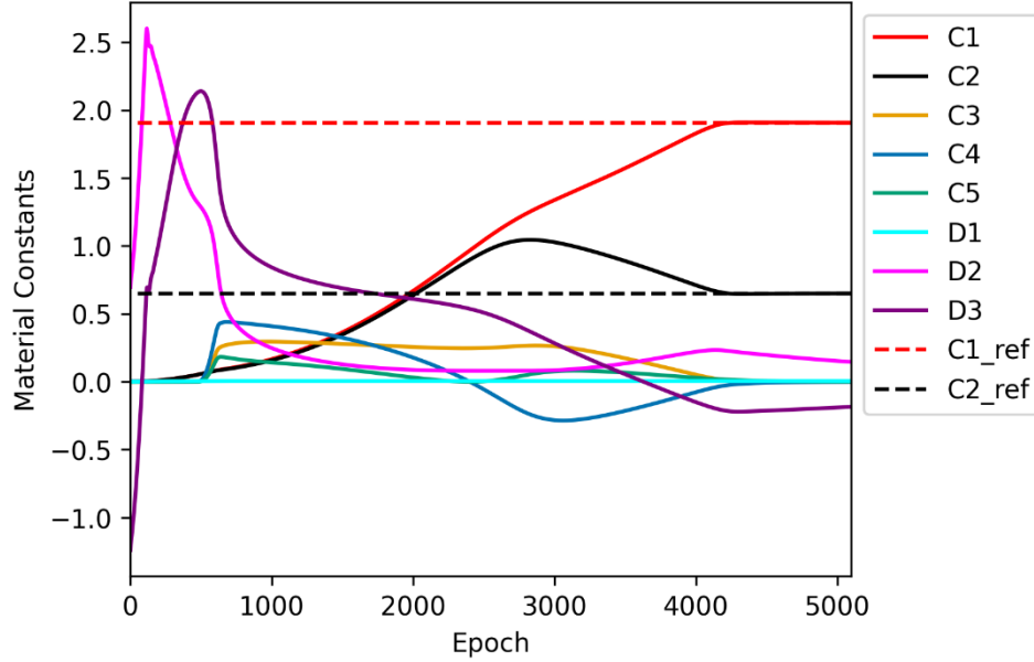
Fig. 6.8 Calculated material constants as a function of completed epochs using Eq. ( 6.15)
