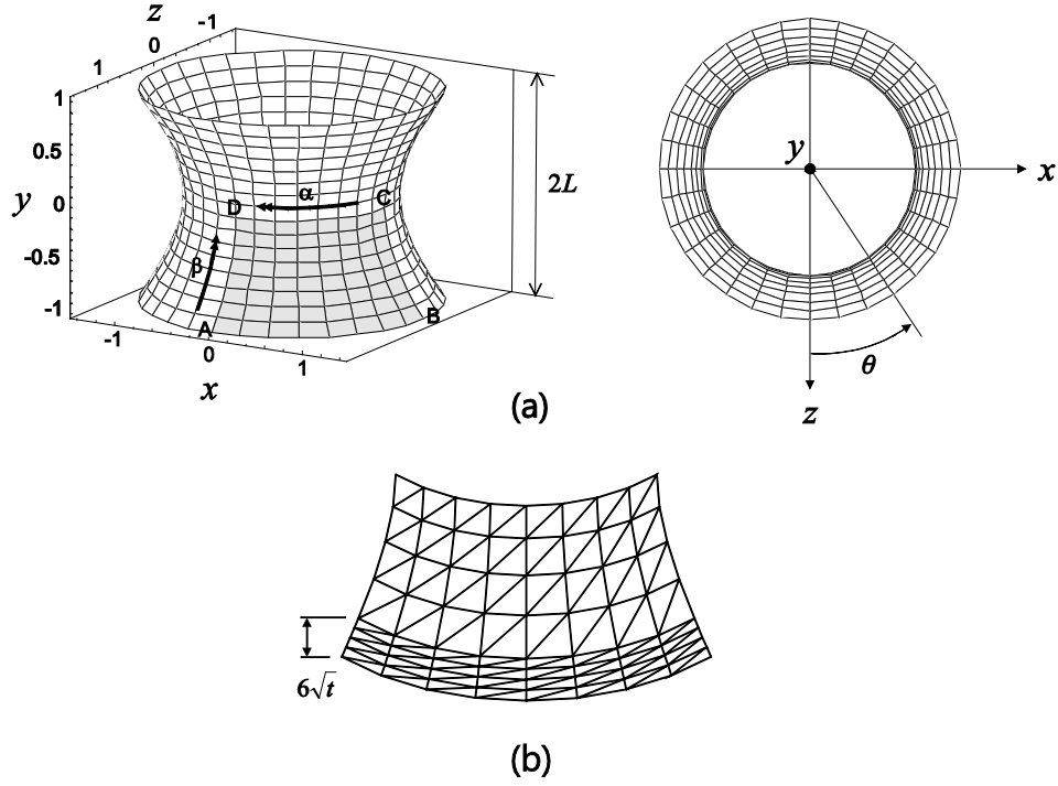
Fig. 2.28. Hyperboloid shell problem ( E = 2.0 \times 10^{11} , \nu = 1/3 and p_0 = 1.0 ). (a) Problem description. (b) Graded mesh for the clamped case ( 8 \times 8 mesh).
