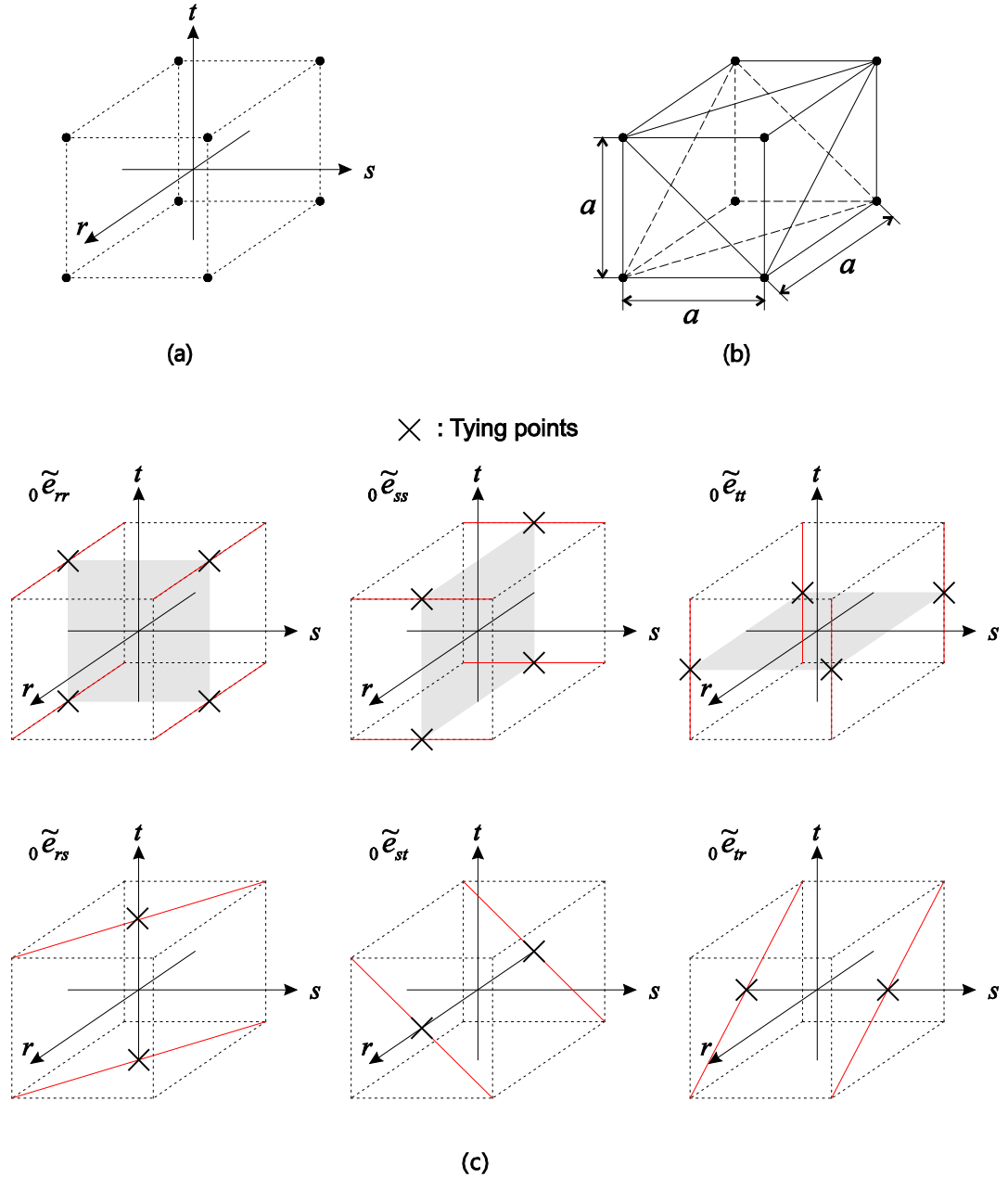
Fig. 2.34 Selection of tying strains and positions for the 3D-MITC8 element, Y. Ko and K.J. Bathe [A].
