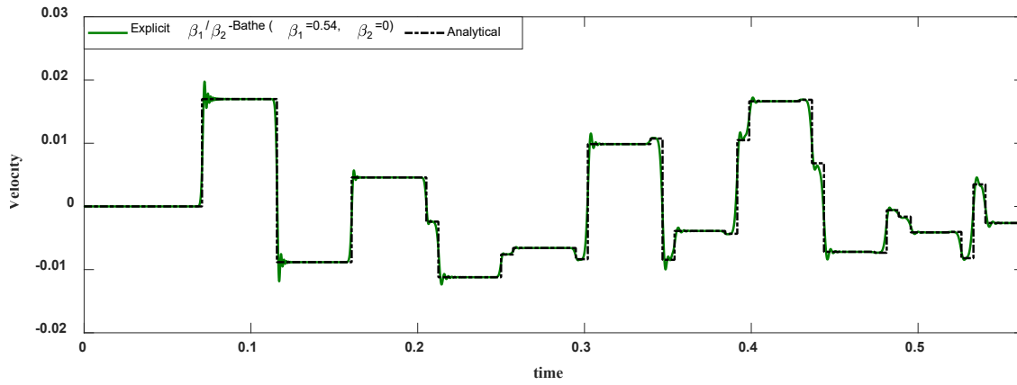
Fig. 4.14 (b) Solution using the \beta_1/\beta_2 -Bathe method with CFL = 1.925
