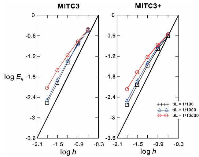
Fig. 2.29. Convergence curves for the clamped hyperboloid shell problem using non-distorted meshes
