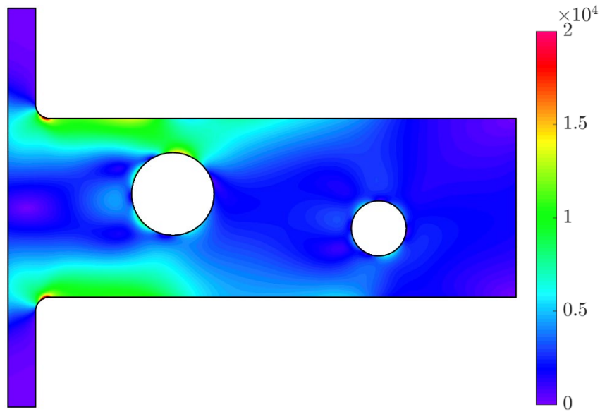
(b) Solutions of the effective stress \bar{\tau}
