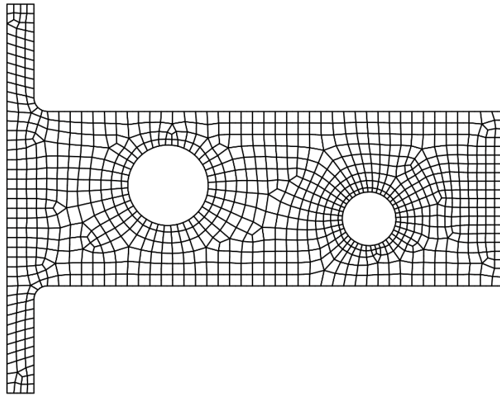
Fig. 3.37 A traditional 9-node finite element mesh
