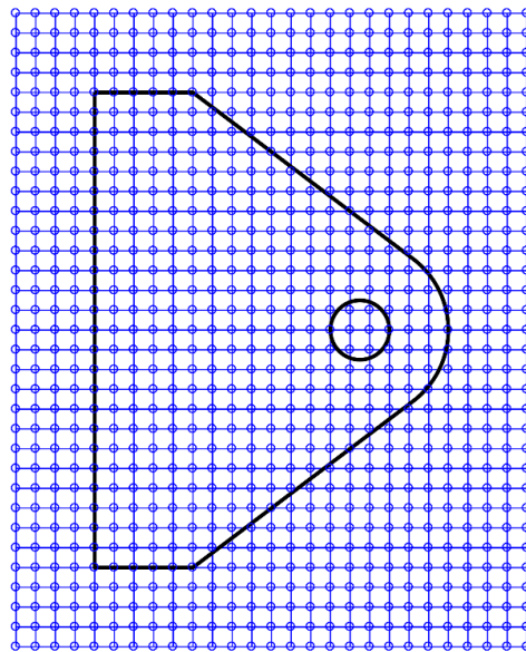
Fig. 3.39 The bracket problem, K.J. Bathe [D]
