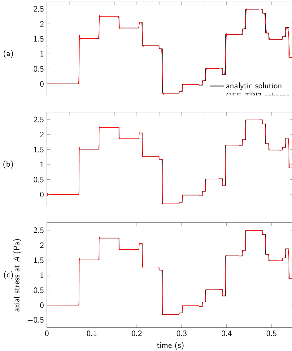
Fig.3.15 Predicted axial stress histories at the point A using the OFE-TRI3 with the \beta_1/\beta_2 -Bathe method ( \gamma 0.5 and \beta_1 = 0.35 with \beta_2 = 2\beta_1 ), A uniform mesh of N = 160 elements (80 elements in each material) is used and the time step size is set using (a) the wave speed of the second material (the smaller wave speed) and (b) that of the first material (the larger wave speed) both with CFL = 0.125 . (c) A non-uniform mesh of N = 160 elements (80 elements for each material) is used and the time step size is set using the larger wave speed with h = L / N and CFL = 0.125 . The non-uniform mesh is constructed by randomly distributing the nodes under the condition that the size of each element is 0 < \Delta x < 2L/N .
