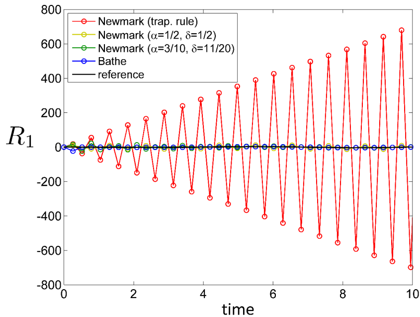
(a) Reaction force at node 1 for various methods
