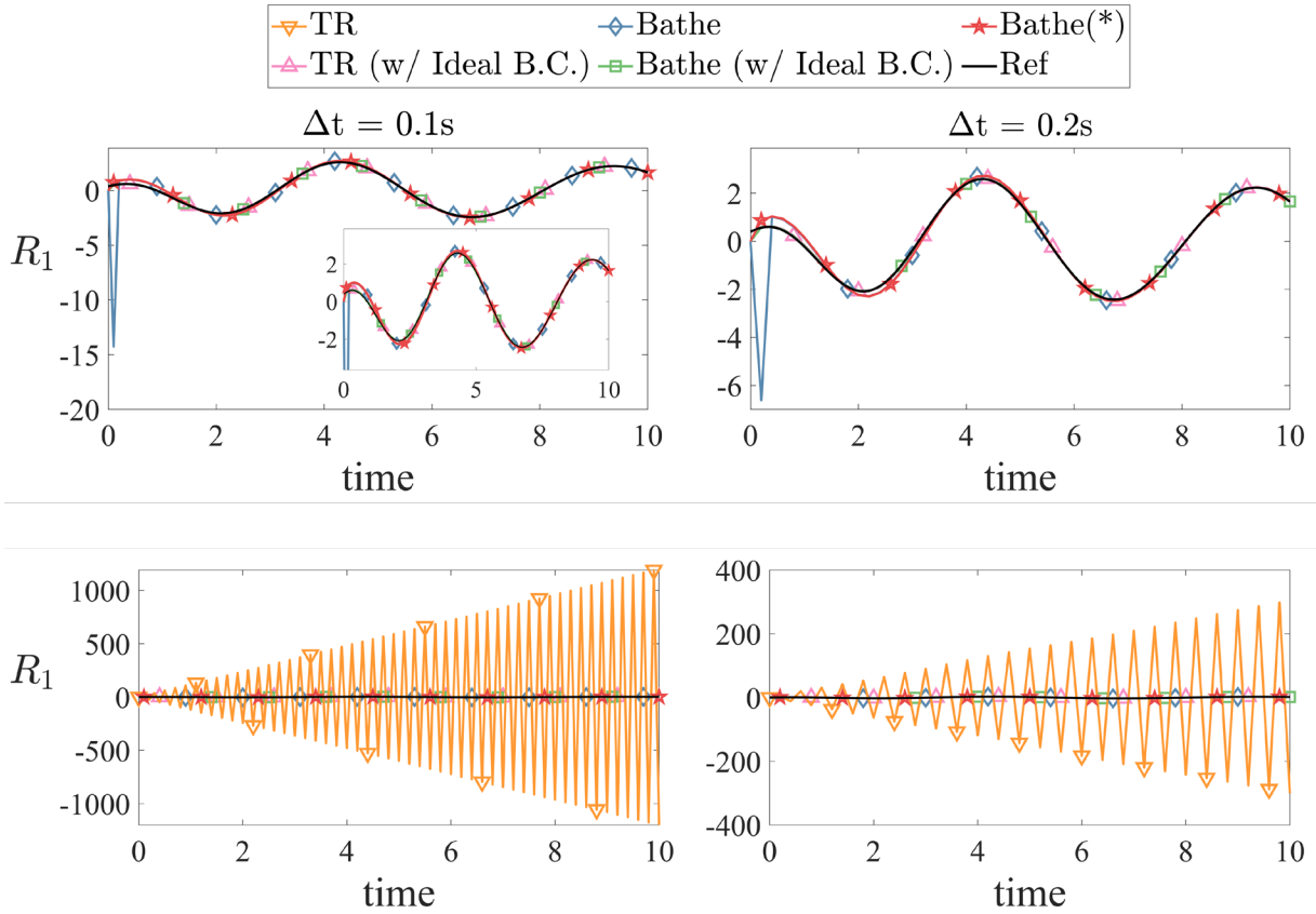
Fig. 4.26 Prediction of reaction force; “Bathe(*)” uses \alpha = 1 and \delta = 3/4 only for the first step, and \alpha = 1/4 and \delta = 1/2 otherwise; the results of the computed reaction for “TR” are shown separately due to the different scale.
