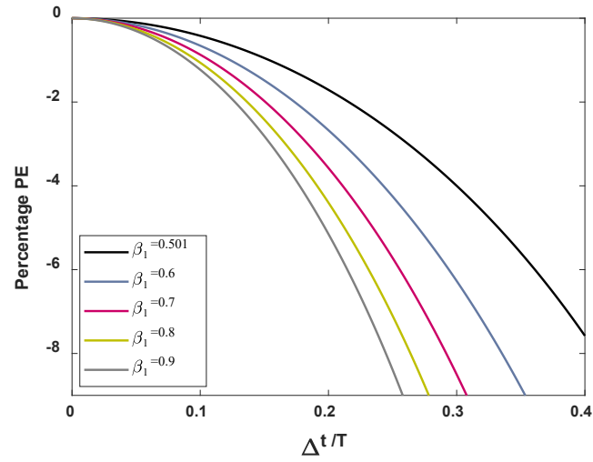
(b) Period elongation of the explicit \beta_1/\beta_2 -Bathe method; first-order scheme, \beta_2 = 0 , with \xi = 0.0
