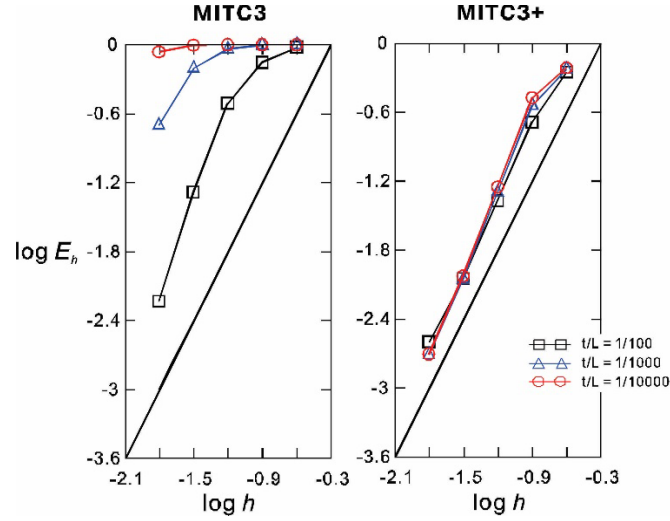
Fig. 2.32 Convergence curves for the free hyperboloid shell problem with the distorted meshes shown in Fig. 2.25.
