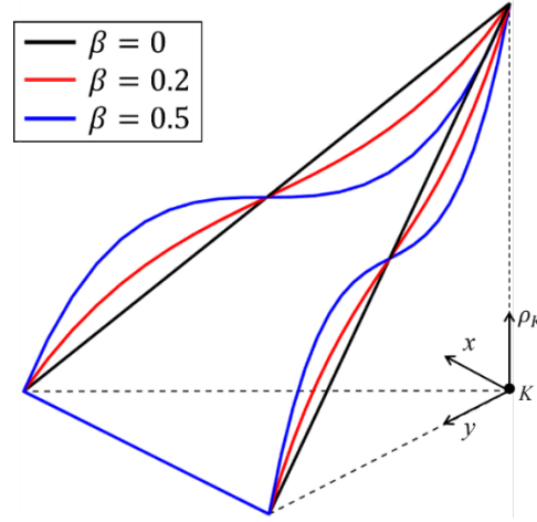
Fig. 3.3 Interpolation function \rho_K for a 3-node overlapping finite element
