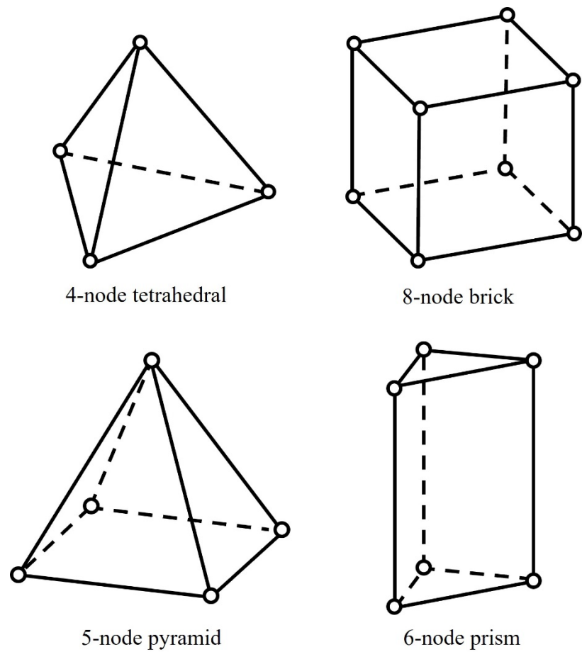
(b) Elements for three-dimensional analyses
