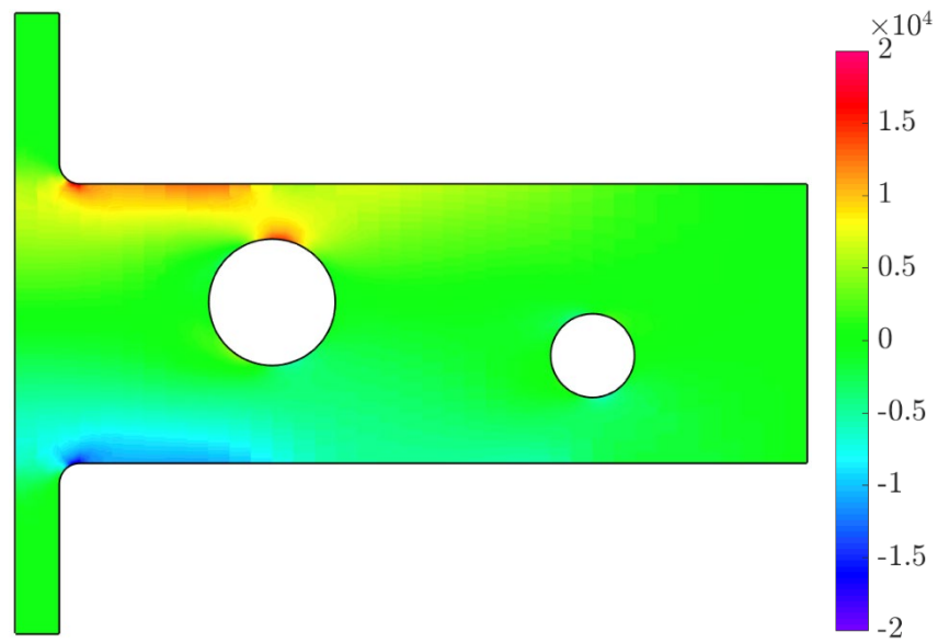
Solution using overlapping meshes
