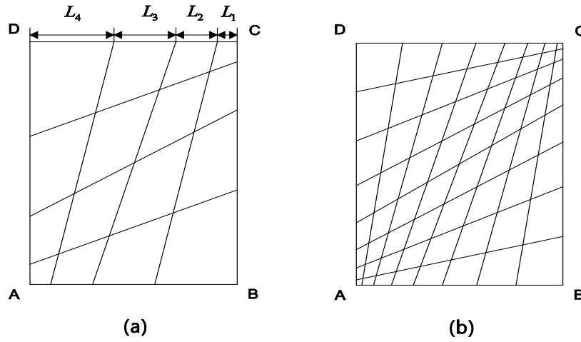
Fig. 2.7 Distorted mesh patterns for (a) N = 4 and (b) N = 8 .
