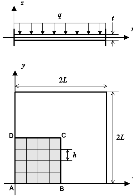
Fig. 2.6 Fully clamped square plate under uniform pressure ( L = 1.0 , E = 1.7472 \times 10^7 , q = 1.0 and \nu = 0.3 ).
