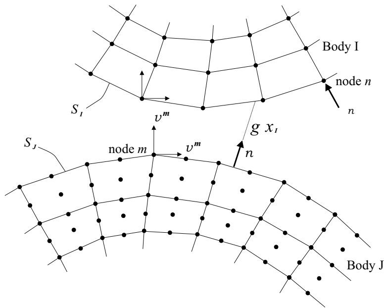
FIGURE 3. Discretizations of bodies in contact region; nodal-point displacements (and nodal Lagrange multiplier if used) are shown.
