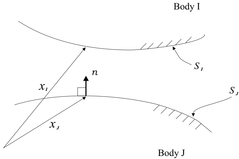
FIGURE 2. Geometry used to calculate the gap
