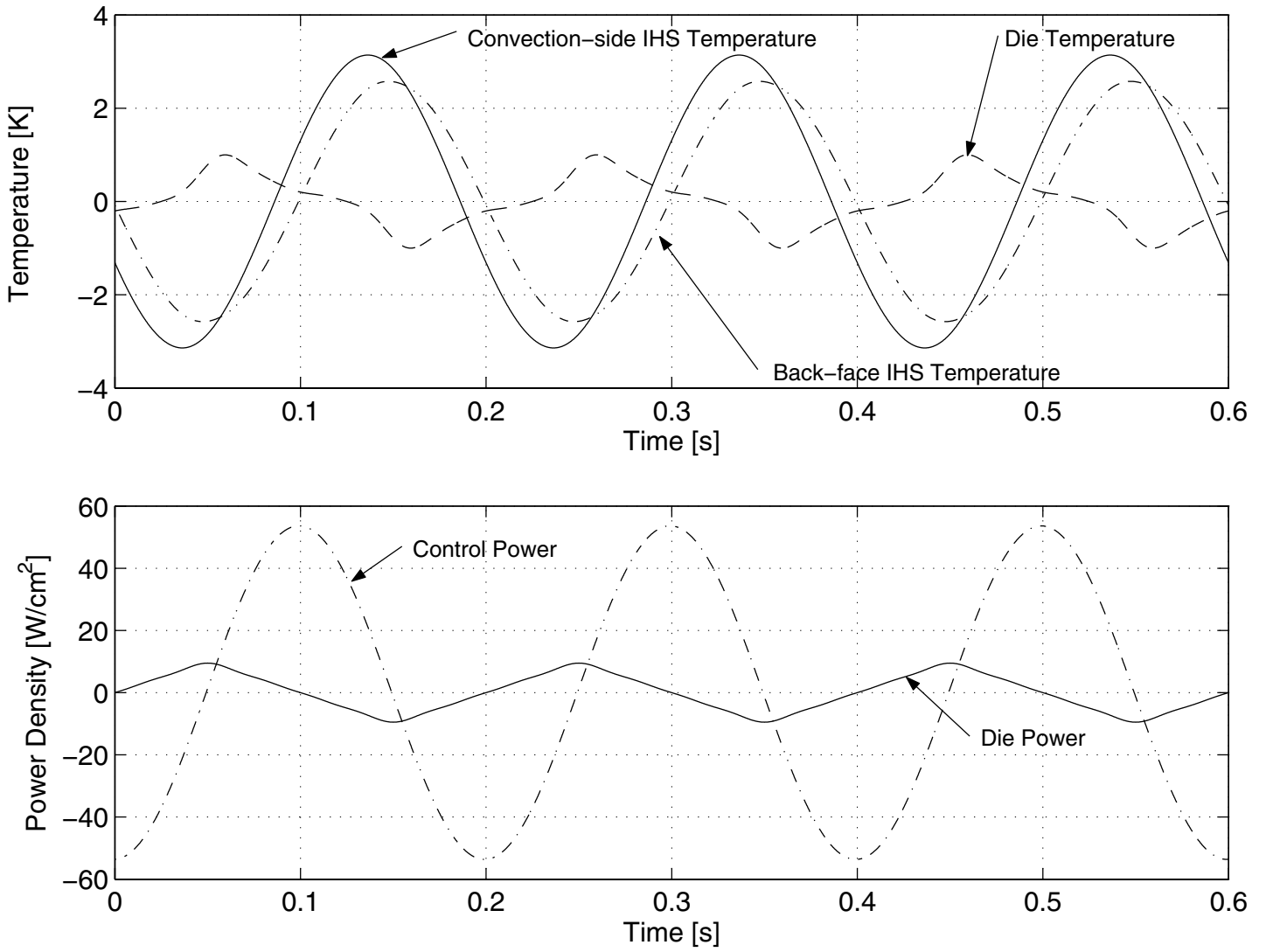
Figure 6. Temperature and power profiles for triangular wave die power profile and a prescribed temperature tolerance of \Delta T = 2 K. Properties are given in Table 1 and Table 2.
