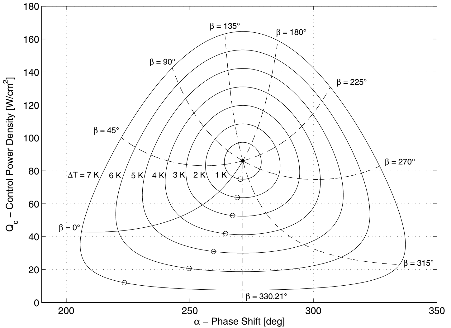
Figure 3. Control power densities and phase shifts for single frequency die power profile ( \omega = 5 Hz and Q_c = 10 W/cm 2 ) and multiple prescribed temperature tolerances \Delta T . The problem properties are given in Table 1 and Table 2. The circles \circ mark the points computed using the method given in Ref. [4].
