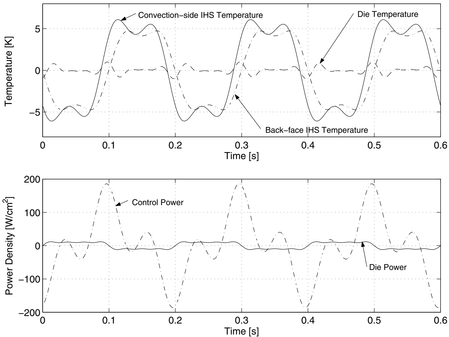
Figure 5. Temperature and power profiles for square wave die power profile and a prescribed temperature tolerance of \Delta T = 2 K. Properties are given in Table 1 and Table 2.
