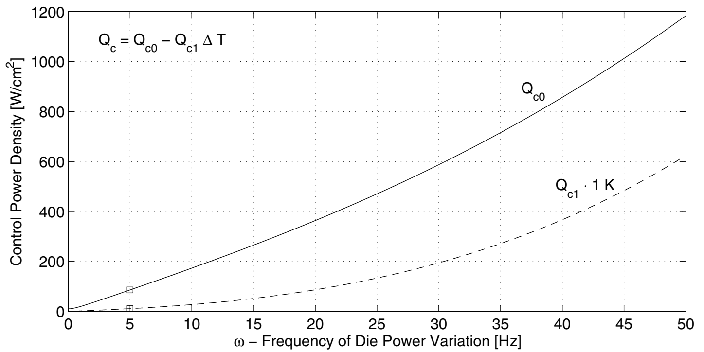
Figure 4. Control power density for optimal control of a single frequency die power profile with Q_d = 10 \text{ W/cm}^2 and frequencies from zero to 50 HZ.
