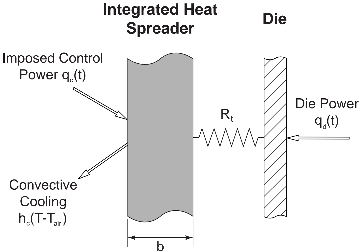
Figure 2. Schematic diagram of simplified device for transient analysis.
