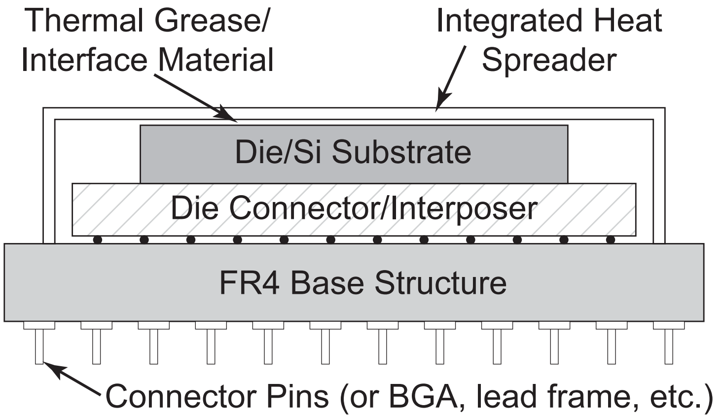
Figure 1. Typical cross-section of a high-power microprocessor device.
