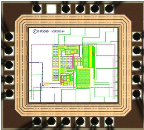
Fig. 9. Die micrograph overlaid by the layout.
