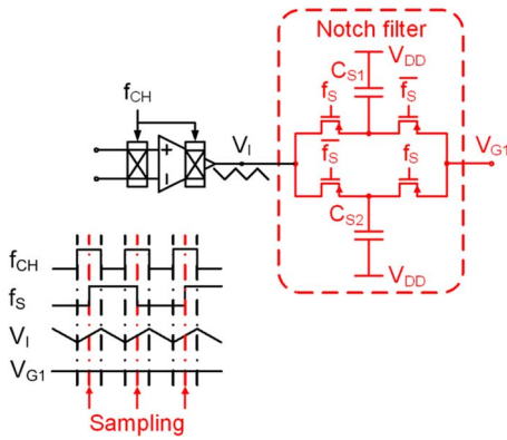
Fig. 7. Implementation of the notch filter.
