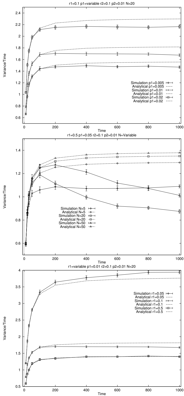
Figure 6-3: Variance of the output of a two-machine finite buffer size: analytical vs. simulation results
