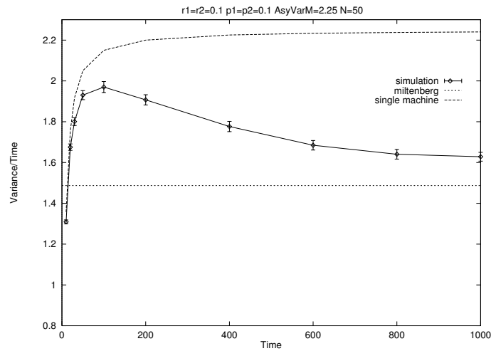
Figure 7-5: Same efficiency: Evolution of the variance as N \rightarrow \infty
