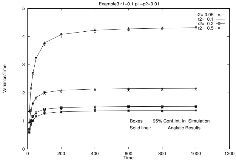
Figure 3-6: Variance of the output of a two-machine zero buffer system: analytical results vs. simulations
