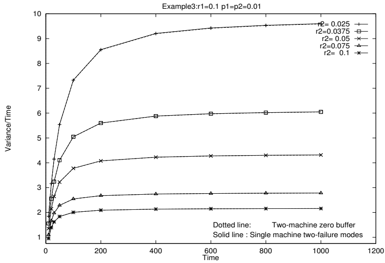
Figure 3-5: Variance of the output: original two-machine zero buffer system vs. simplified single machine with two failure modes
