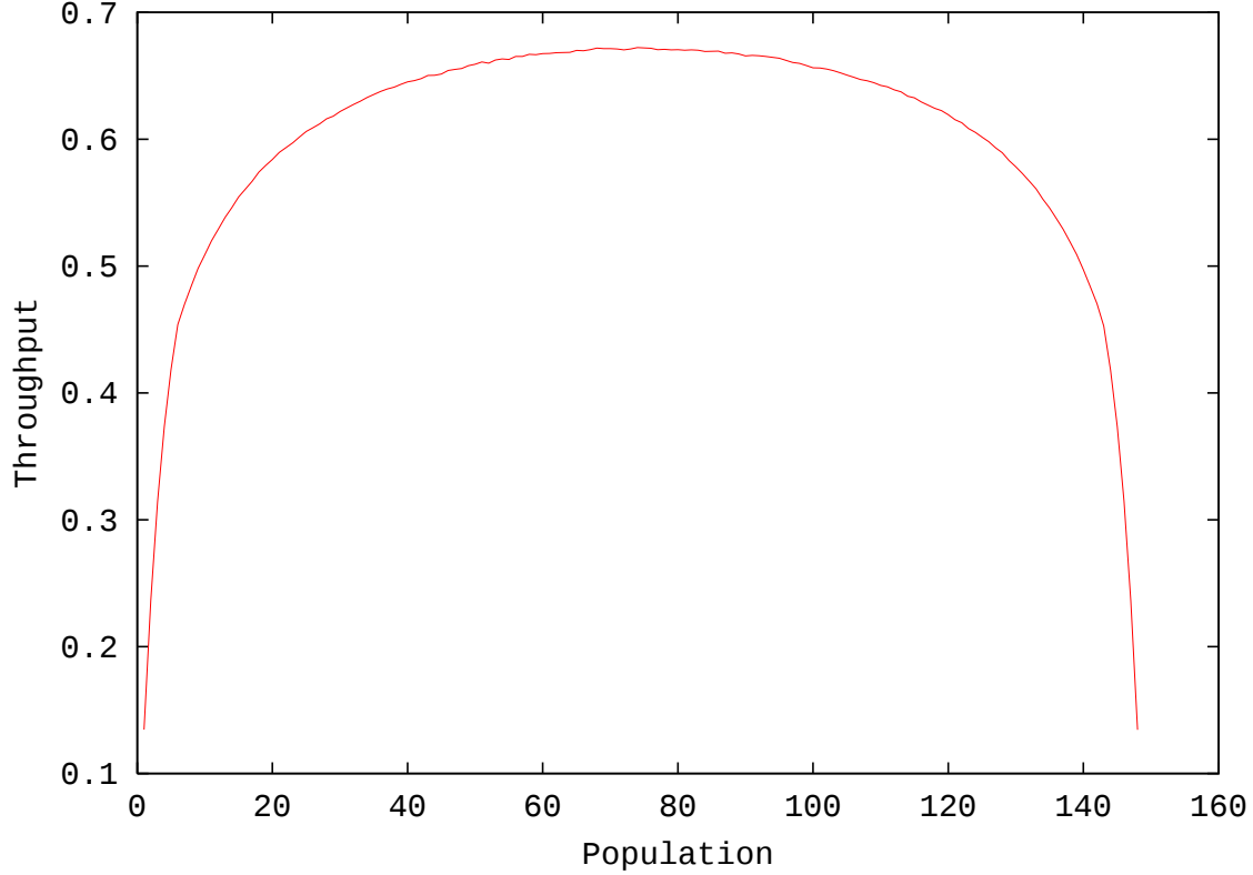
Figure 6-4: Loop 6.4 ( \sigma_{buffers} = 7.97 )
