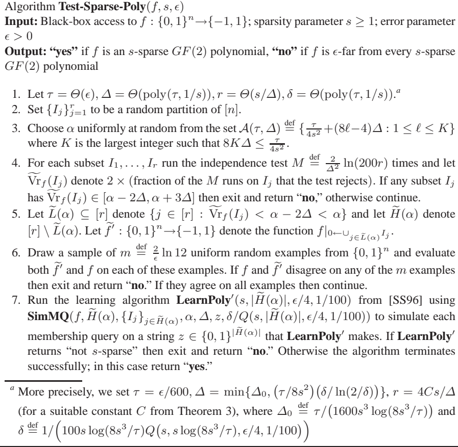
Fig. 1. The algorithm Test-Sparse-Poly .
