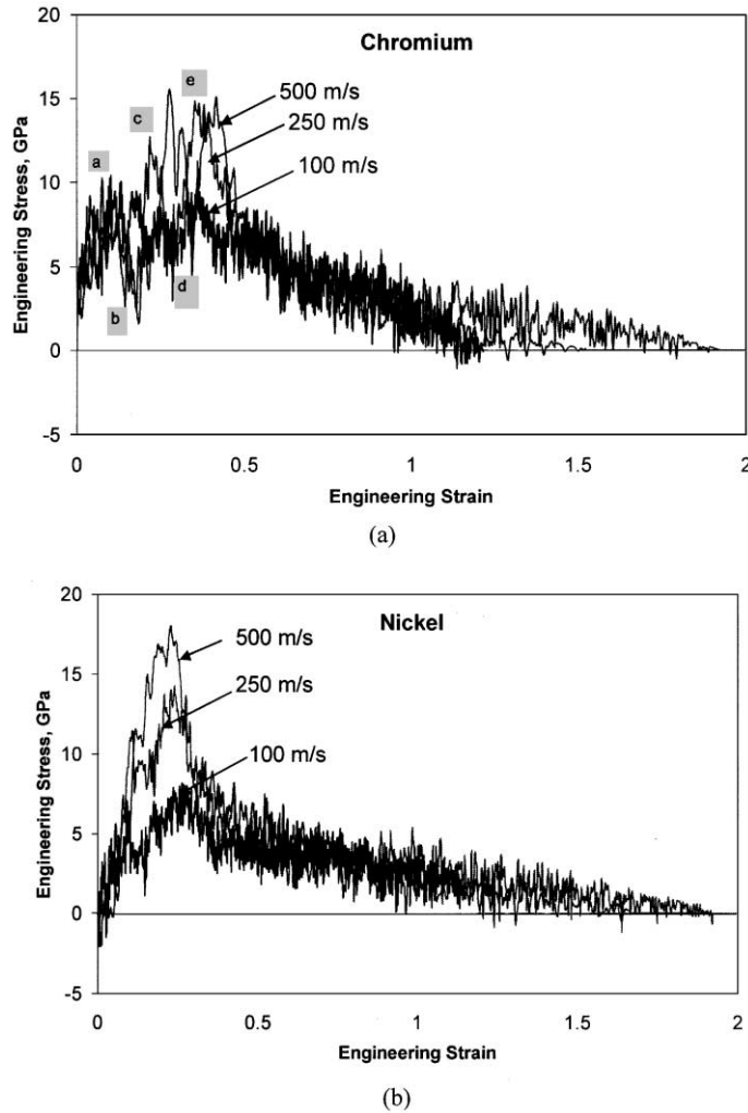
Fig. 12. Variation of the engineering stress with strain at different loading rates (500, 250, and 100 \text{m s}^{-1} ) for: (a) a BCC (Cr); and (b) an FCC material (Ni), respectively.
