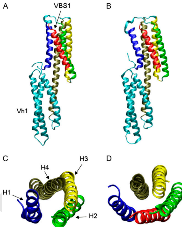
FIGURE 1 (A) Vh1 (PDB 1RKE) and VBS1 (PDB 1T01) unbound structures viewed from the front. VBS1 is translated by 12 Å from its corresponding position within the Vh1-VBS1 complex. (B) Vh1 and VBS1 bound complex (PDB 1T01) viewed from the front. (C) Vh1 and VBS1 unbound structures viewed from the top. Only the first four helices of Vh1 (a seven-helix bundle) are shown for clarity. (D) Vh1 and VBS1 bound complex viewed from the top.
