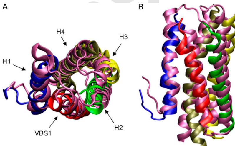
FIGURE 2 (A) RMSD of the equilibration simulation from the Vh1-VBS1 complex crystal structure ( red dashed line ) and RMSD of the Vh1 and VBS1 binding simulation from the Vh1-VBS1 complex crystal structure ( black solid line ). (B) One conformation from Vh1-VBS1 binding simulation (same coloring scheme as in Fig. 1) superimposed with a conformation from Vh1-VBS1 equilibration simulation ( purple ) viewed from the top and (C) viewed from the front.
