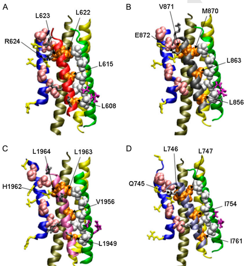
FIGURE 5 Crystal structures of Vh1 bound to various VBS. The backbones of helical sequences are shown in ribbon representation; polar and charged residues are shown in stick representation; and the hydrophobic residues are shown as spheres. (A) Vh1-VBS1 complex (PDB 1T01) with critical residues important in binding of the two molecules. VBS1 is shown as red ribbon. (B) Vh1-VBS2 complex (PDB 1U6H) and corresponding critical residues are labeled. VBS2 is shown as a gray ribbon. (C) Vh1-VBS3 complex (PDB 1RKC) and the corresponding critical residues are labeled. VBS3 is shown as a purple ribbon. (D) Vh1- \alpha VBS complex (PDB 1YDI) and the corresponding critical residues are labeled. \alpha VBS is shown as a silver ribbon.
