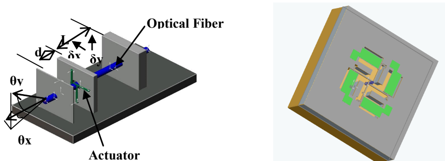
Fig. 14 Concept of DPBS and a 2D actuation device
