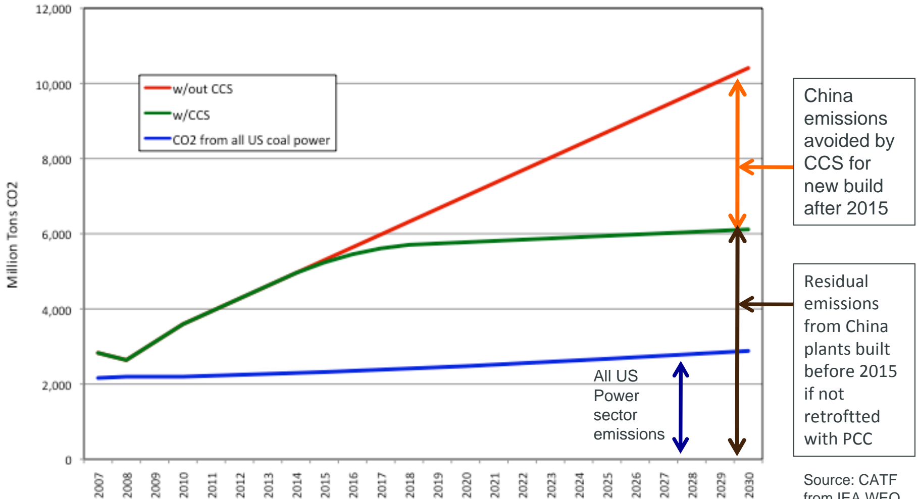
Annual CO2 Emissions From New Generating Capacity in China, 2007-2030 (with and without CCS phase-in for all new China plants starting 2015)
