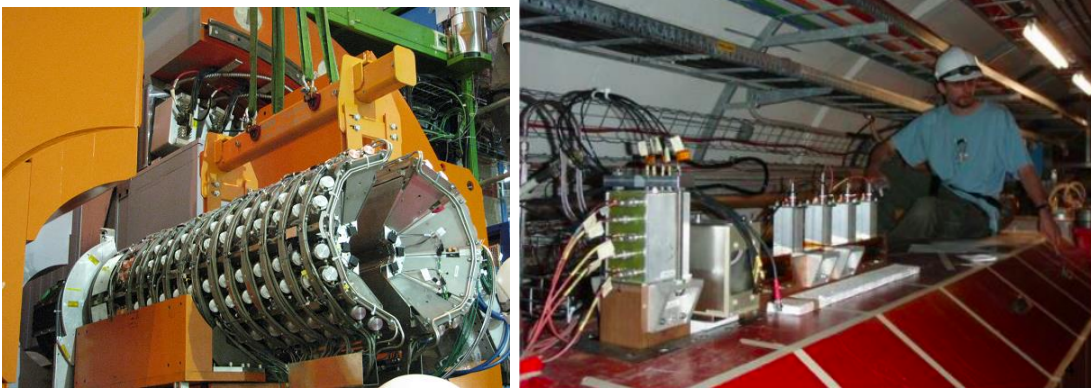
Figure 3-15: The picture of the CASTOR (left) at the CMS underground collision hall and ZDC (right) at 140 m away from the CMS beam interacting point are shown above.
