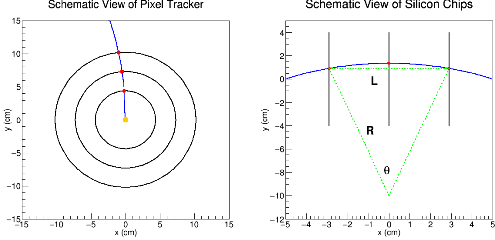
Figure 4-5: A track (blue) initiated from the beam spot (orange) passing through 3 layers of pixel detectors (black) leaving 3 clusters (red) is shown on the left and the circular fit to the 3 clusters with the definition of R , L , and \theta is shown on the right.
