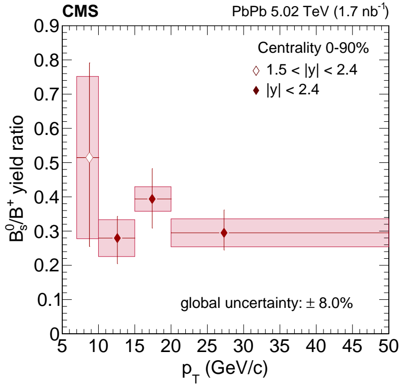
Figure 5-73: The measurement of B_s^0/B^+ as a function of p_T is shown above. The open markers from 7 - 10 GeV/c stand for the fiducial measurements in B-meson rapidity of 1.5 < |y| < 2.4 .
