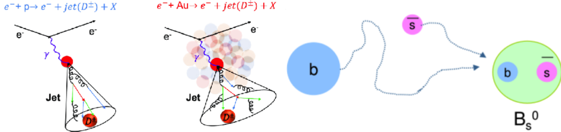
Figure 1-4: The fragmentation process of charms quarks hadronize into D^\pm (left) and the coalescence process of a beauty quark combining with a strange quark nearby to form a B_s^0 are shown above.
