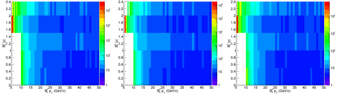
Figure 5-49: The finely binned 2D \frac{1}{\alpha \times \epsilon} vs B_s^0 p_T and B |y| in centrality 0 - 90% (top), 0 - 30% (middle), and 30% - 90% (bottom) are shown respectfully above.
