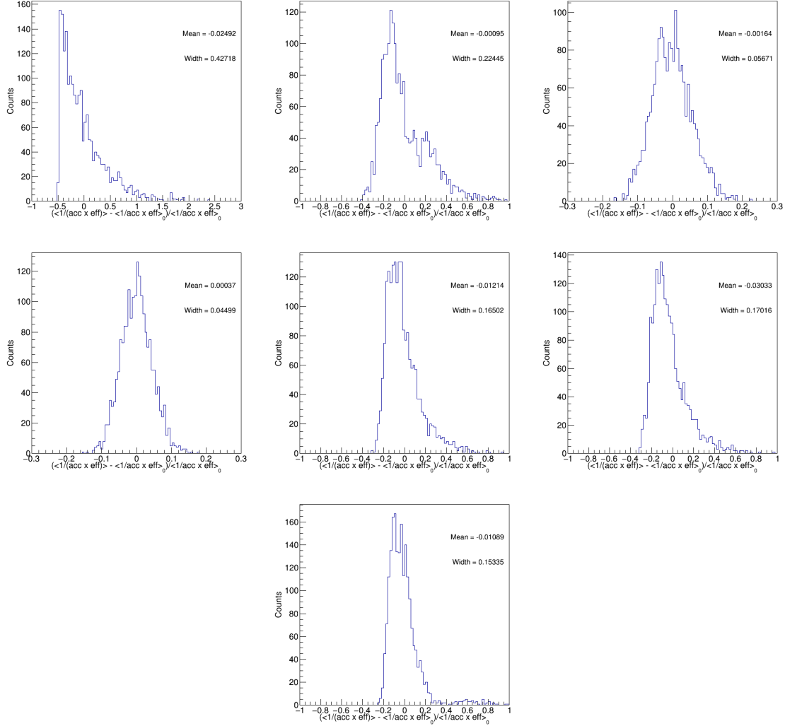
Figure 5-57: The percent deviation distributions of B_s^0 \langle \frac{1}{\alpha \times \epsilon} \rangle to RECO/GEN for the data-like randomly constructed MC samples in centrality 0 - 90% from 7 - 10, 10 - 15, 15 - 20, and 20 - 50 GeV/c as well as 0 - 90%, 0 - 30%, and 30 - 90% event centrality from 10 - 50 GeV/c are shown respectfully above.
