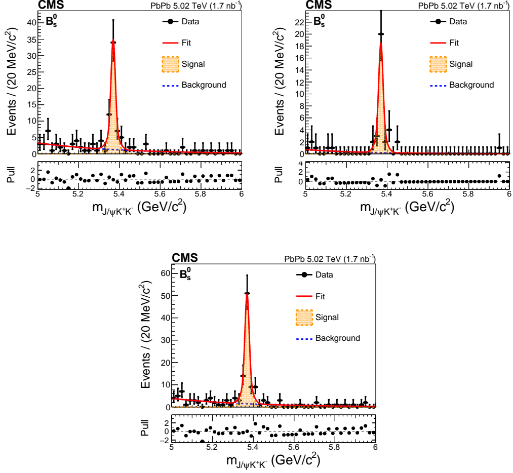
Figure 5-34: The B_s^0 invariant mass distributions as well as the fits to extract the signal raw yield N_S in centrality bins 0 - 30%, 30 - 90%, and 0 - 90% are shown above.
