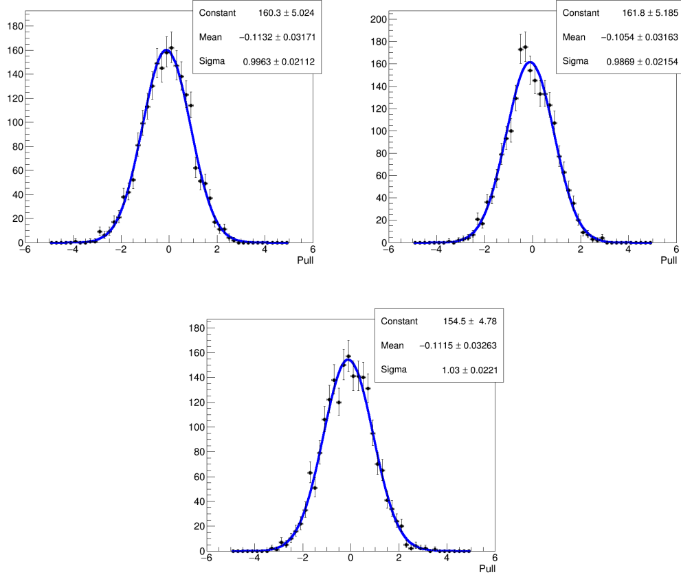
Figure 5-56: The B^+ pull distributions and the Gaussian fits for 0 - 30%, 30 - 90%, and 0 - 90% event centrality are shown respectfully above.
