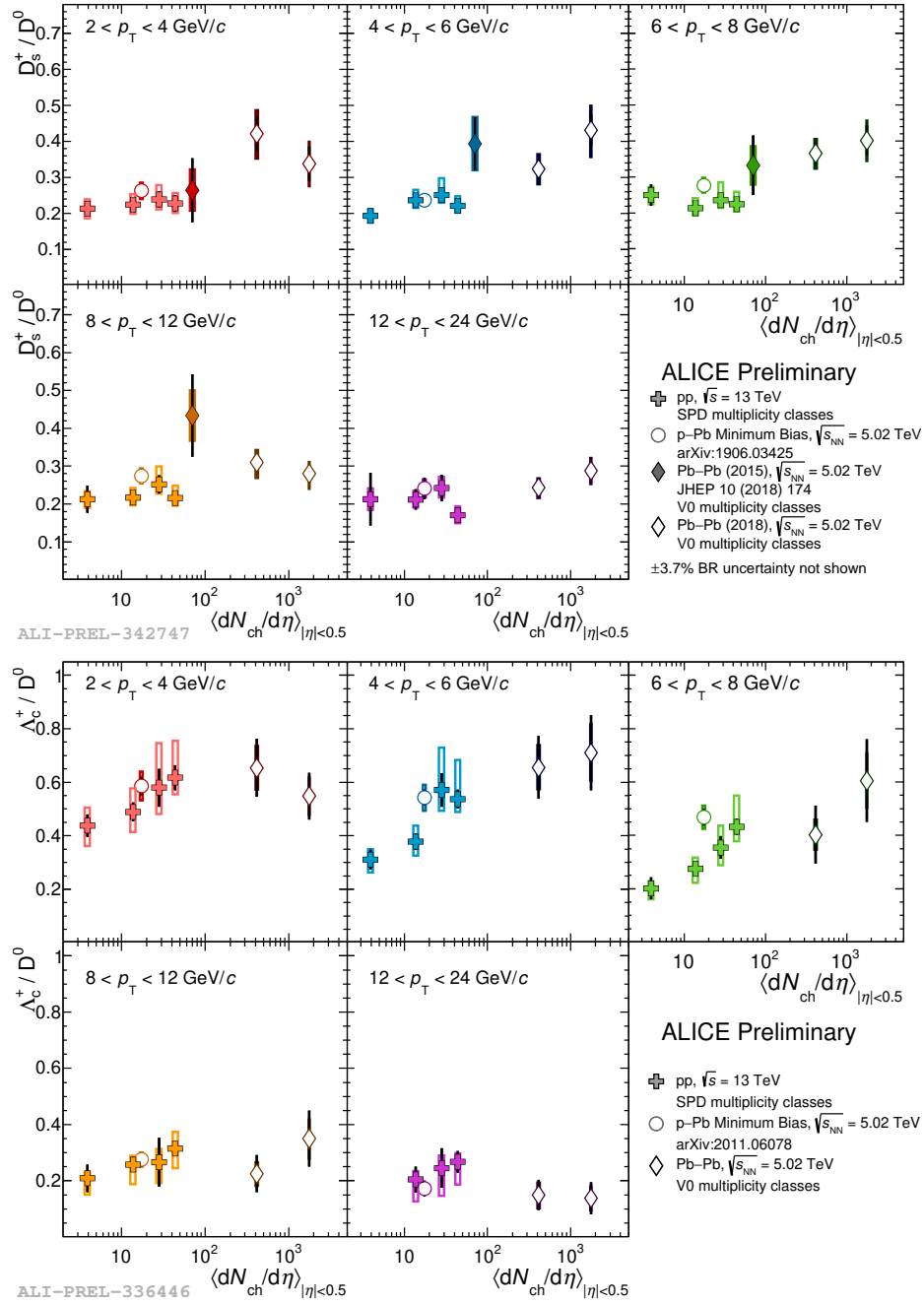
Figure 2-9: The fully reconstructed D_s^+/D^0 (top) and \Lambda_c^+/D^0 ratios (bottom) as a function of event multiplicity \langle dN_{ch}/d\eta \rangle within |\eta| < 0.5 in p_T from 2 - 4, 4 - 6, 6 - 8, 8 - 12, and 12 - 24 GeV/c in pp, pPb, and PbPb collisions measured by the ALICE experiment are shown above.
