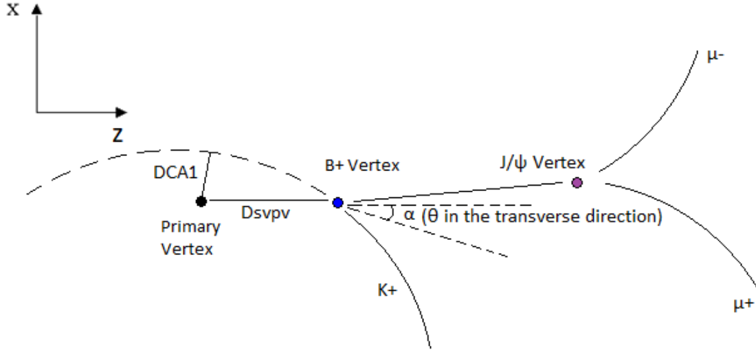
Figure 5-15: The definitions of topological variables in the decay of B^+ \rightarrow J/\psi K^+ \rightarrow \mu^+ \mu^- K^+ are schematically shown above.
