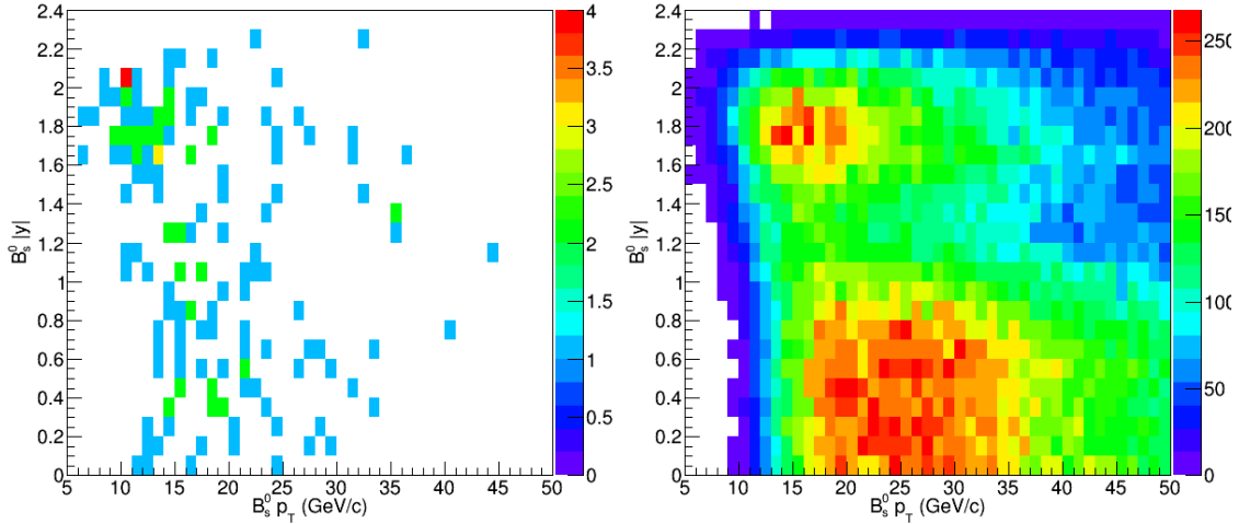
Figure 5-47: The finely binned 2D B-meson candidates distribution vs p_T and |y| for data (left) and MC (right) in centrality 0 - 90% are shown respectfully above.
