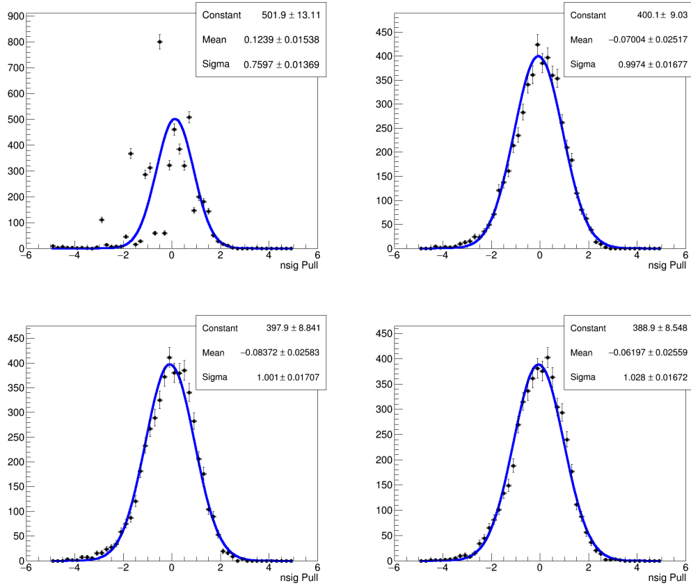
Figure 5-53: The B_s^0 pull distributions and the Gaussian fits for 0 - 90% from p_T 7 - 10, 10 - 15, 15 - 20, 20 - 50 GeV/c are shown respectfully above.
