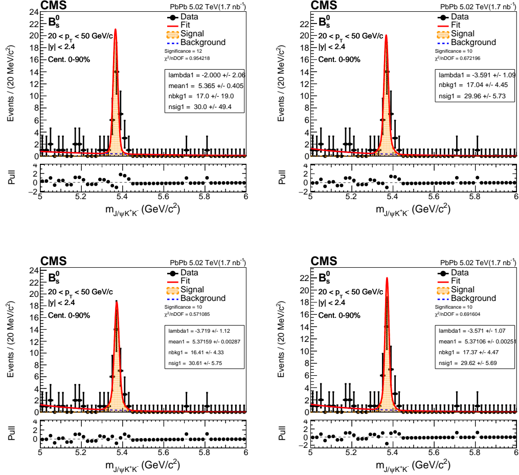
Figure 5-65: The fits of B_s^0 invariant mass distributions for p_T from 20 - 50 GeV/c and centrality from 0 - 90% are shown above. The signal PDFs are gaussian (with widths and relative proportions fixed from MC), double gaussian with all the parameters fixed (including the mean), increased width ( a=1.1 ), and decreased width ( a=0.9 ) from top left to bottom right.
