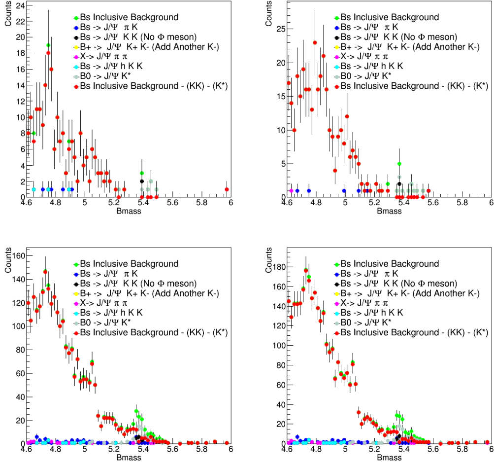
Figure 5-27: Individual NP background contributions with respect to the total background components from 10 to 15 GeV (top left), 15 to 20 GeV (top right), 20 to 50 GeV (bottom left), and 10 to 50 GeV (bottom right) in B_s^0 invariant mass distributions. The non-prompt background from all channels listed above is negligible compared to the inclusive background. Also, no peak near the B_s^0 resonance is observed when the B^0 \rightarrow J/\psi K^{*0} and B_s \rightarrow J/\psi K^+ K^- components subtract from inclusive background.
