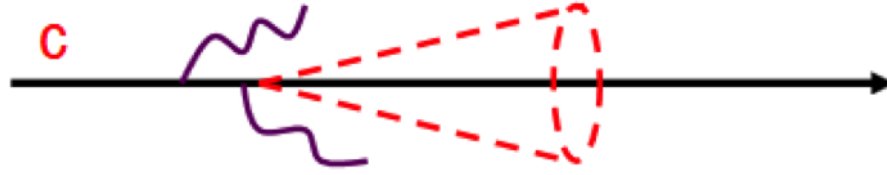
Figure 1-39: The schematic demonstration of a charm quark radiation is shown above. A suppression in small angles due to the dead cone effect in the QGP medium is highlighted.
