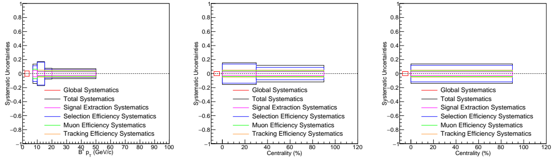
Figure 5-70: The summary of B^+ systematic uncertainties plotted as a function of p_T (left), centrality in 0 - 30% and 30 - 90% (middle), and the inclusive centrality bin 0 - 90% (right) are shown above.
