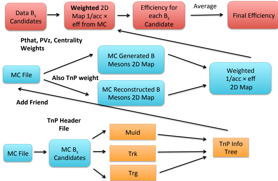
Figure 5-48: The workflow for the efficiency correction including the data-driven tag-&-probe approach in B-meson analysis is shown above.
