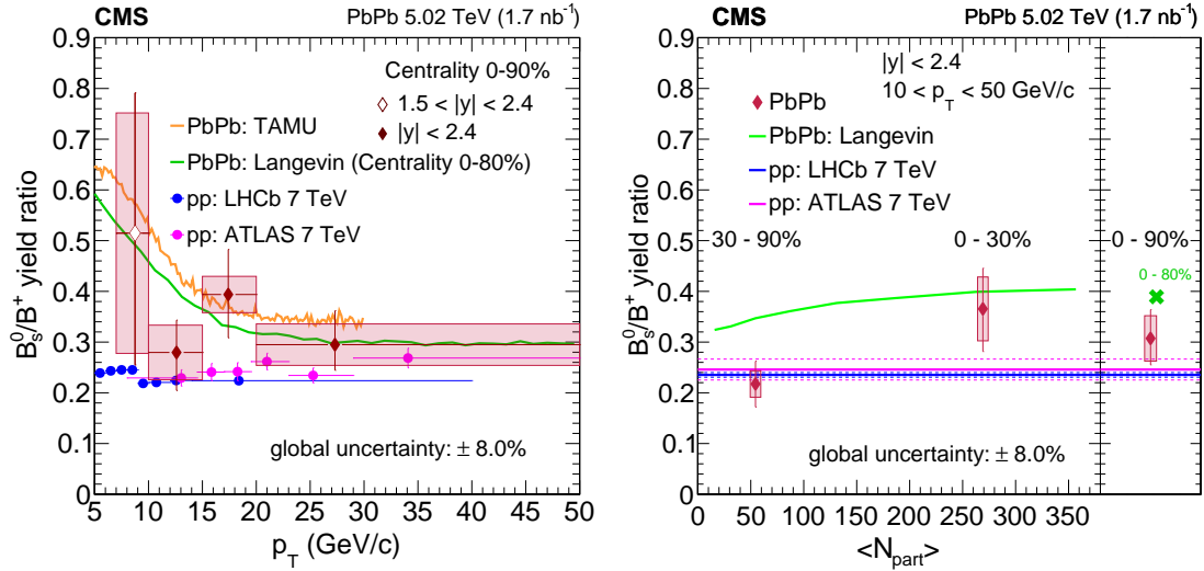
Figure 6-1: The fully reconstructed B_s^0/B^+ ratio (right) as a function of p_T (left) and PbPb event centrality (right) using the 2018 CMS dimuon PbPb dataset are shown above. Both plots include the ATLAS (magenta) and LHCb (blue) 7 TeV pp references. The TAMU model (orange) has only p_T dependent predictions shown on the left figure while the Cao, Sun, Ko model (green) has both p_T and centrality predictions plotted on both figures.
