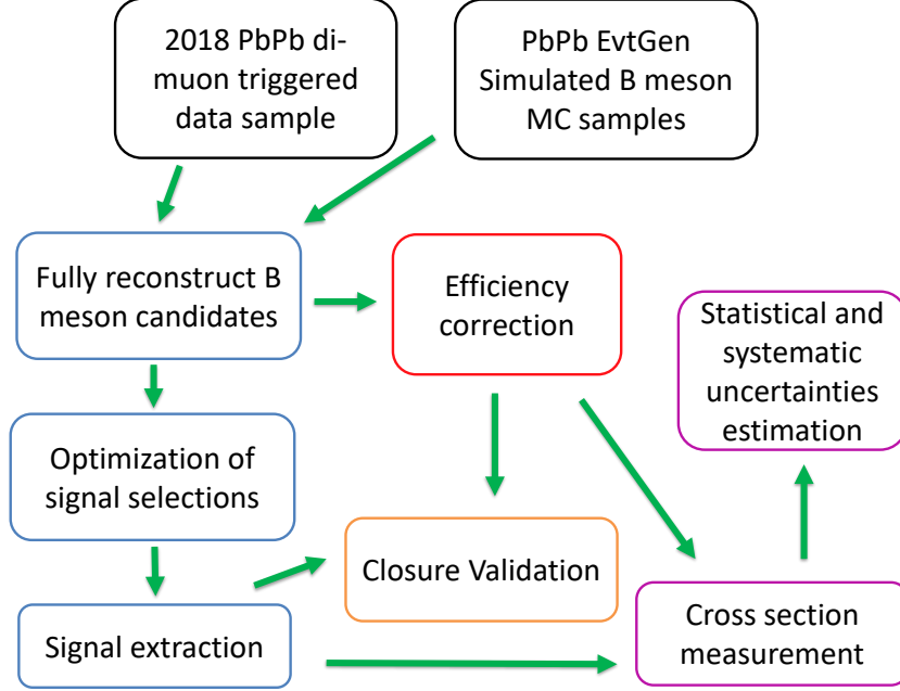
Figure 5-1: The block diagram of the workflow with major steps for B-meson cross section measurements is shown above.
