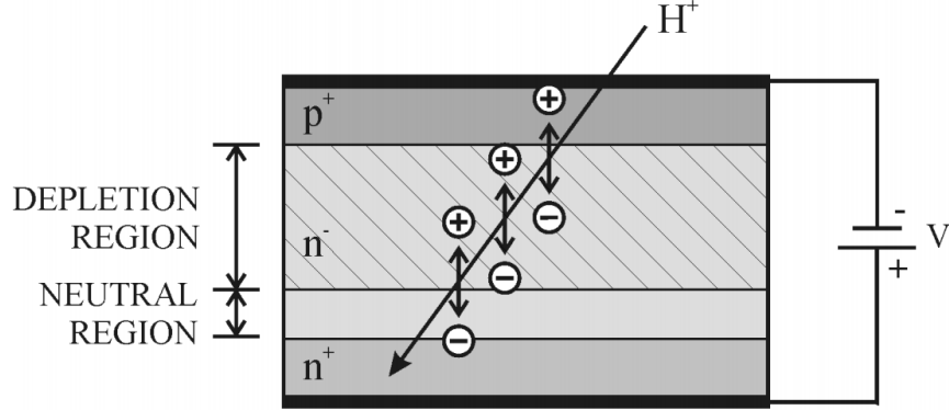
Figure 3-10: The schematic plot explaining how a silicon tracker detects charged particles is shown above.
