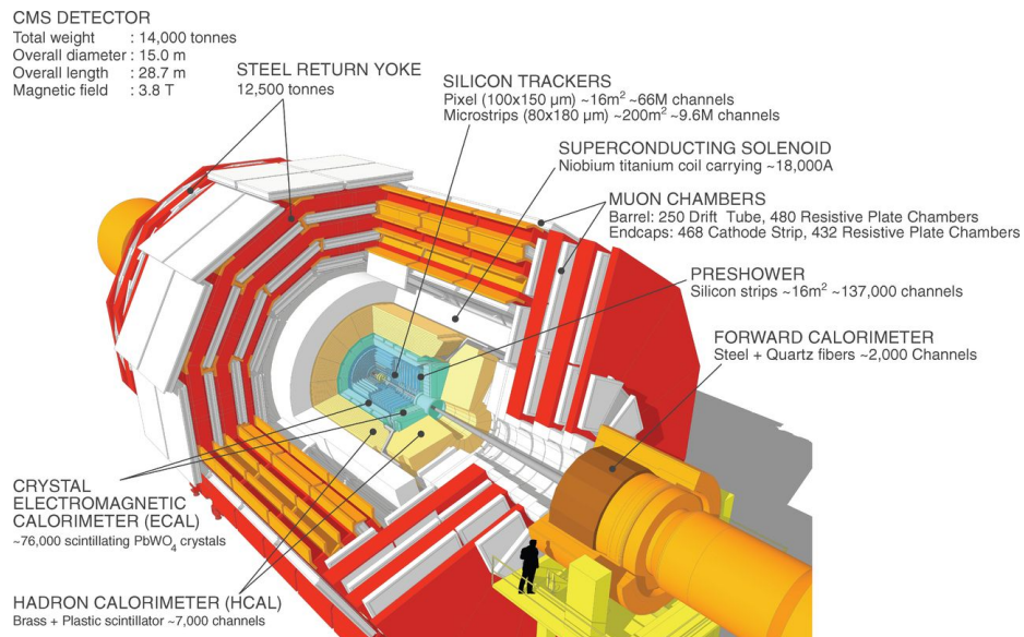
Figure 3-2: The schematic view of the CMS detector with brief descriptions of all its components is shown above. Image from [157]
