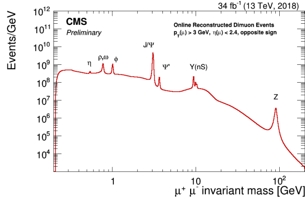
Figure 3-8: The dimuon invariant mass spectrum m_{\mu\mu} reconstructed by CMS HLT trigger in the 2018 pp dataset is shown above. We can identify the neutral vector boson resonances above.
