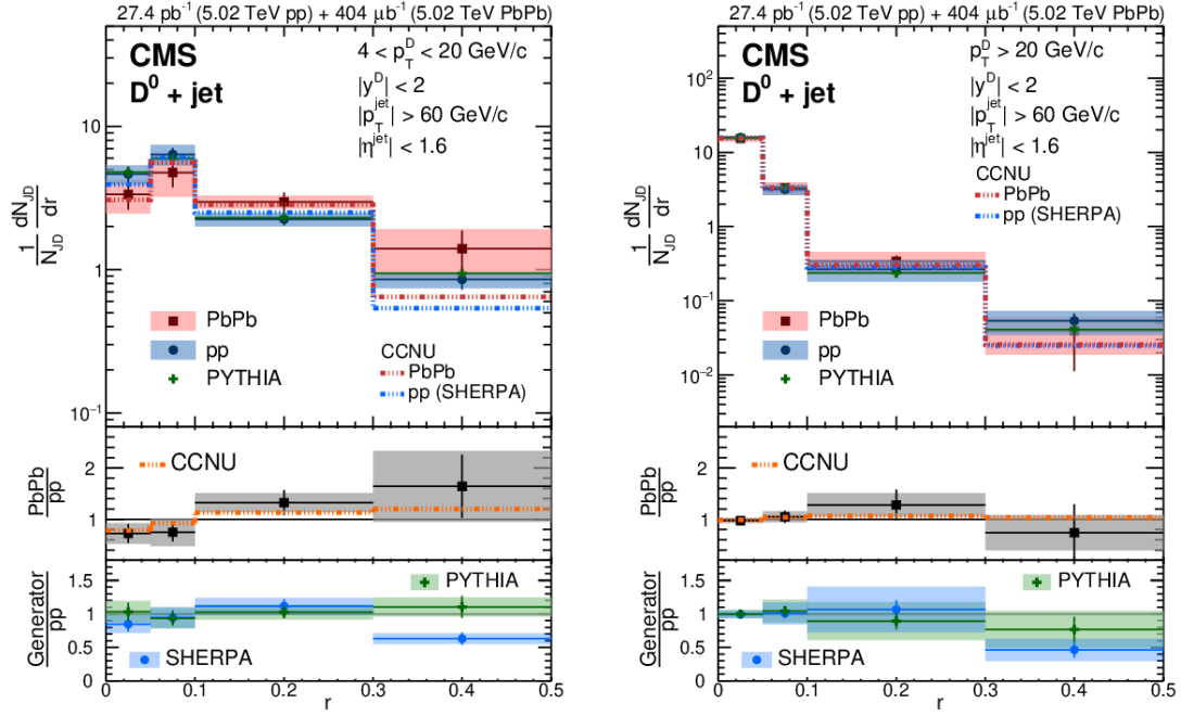
Figure 2-12: Distributions of fully reconstructed D^0 mesons in jets, as a function of the distance from the jet axis ( r ) for jets of p_T^{jet} > 60 GeV/c and |\eta^{jet}| < 1.6 measured in pp and PbPb collisions at \sqrt{s_{NN}} = 5.02 TeV, for 4 < p_T^D < 20 GeV/c and p_T^D > 20 GeV/c, are shown above. The jet radius is defined as r = \sqrt{(\Delta\phi_{jD})^2 + (\Delta\eta_{jD})^2} where \phi_{jD} and \eta_{jD} are the \eta and \phi of the D^0 meson with respect to the jet axis.
