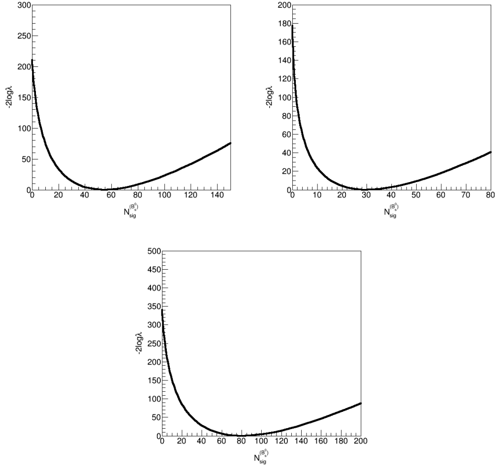
Figure 5-38: The significance vs signal yield for centrality bins in 0 - 30%, 30% - 90% 0 - 90% for p_T from 10 - 50 GeV/c are shown above
