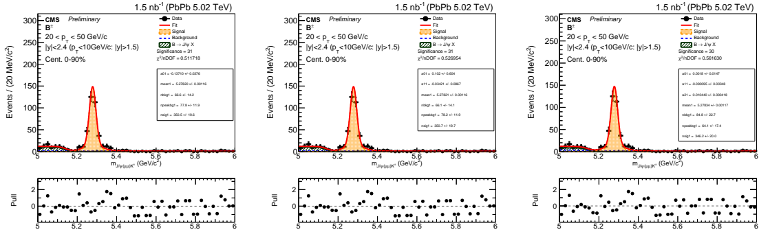
Figure 5-68: The Invariant mass fits to B^+ candidates for B^+ p_T from 20 - 50 GeV/c and centrality from 0 to 90% in 5.02 TeV PbPb. The background PDFs from left to right are first-, second-, and third-order polynomials.
