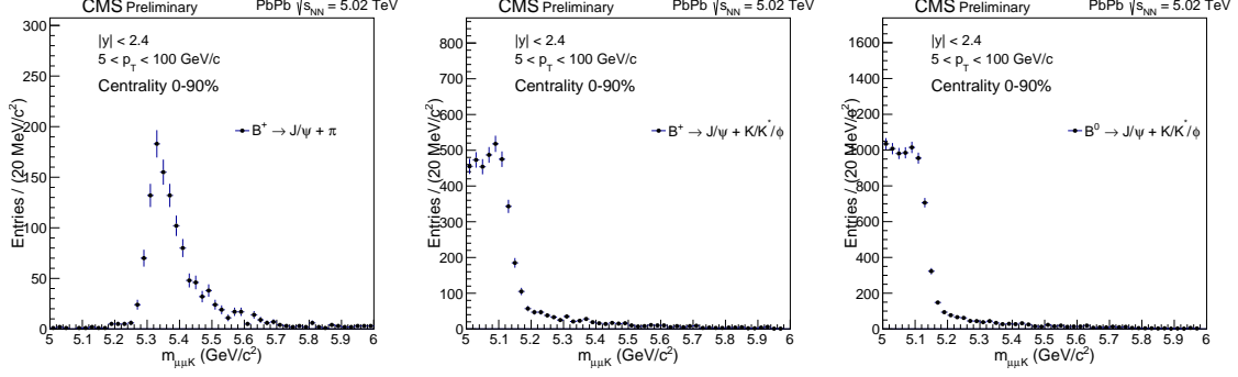
Figure 5-31: Peaking background contribution from B^+ \rightarrow J/\psi\pi and from K^{*0}(892) and K^{*+}(892) resonant decay channels of B^0 and B^+ are shown above.
