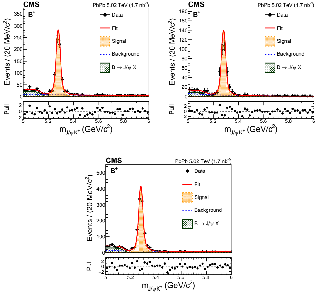
Figure 5-36: The B^+ invariant mass distributions as well as the fits to extract the signal raw yield N_S in centrality bins 0 - 30%, 30 - 90%, and 0 - 90% are shown above.
