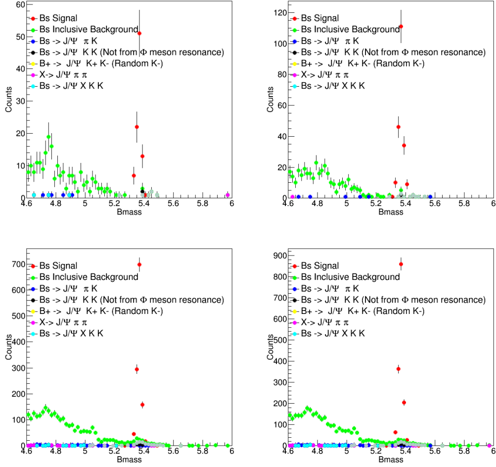
Figure 5-28: Individual Non-prompt background contributions with respect to the total background components and the signal channel from 10 to 15 GeV (top left), 15 to 20 GeV (top right), 20 to 50 GeV (bottom left), and 10 to 50 GeV (bottom right). We can see that the inclusive background is small compared to the signal in our studies.
