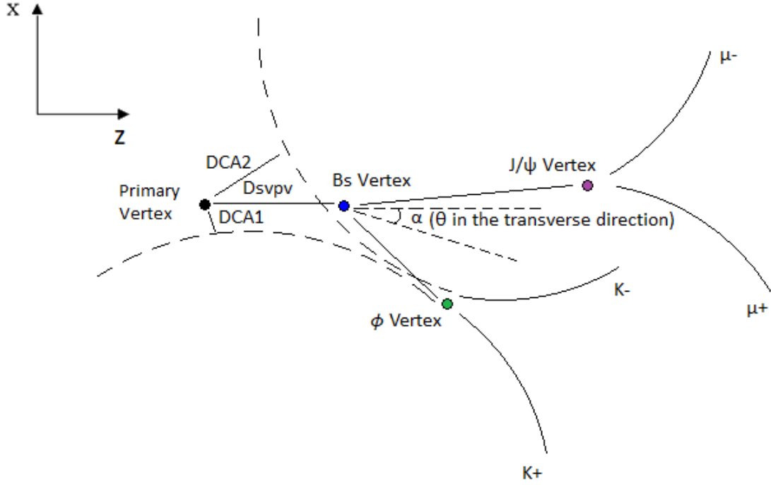
Figure 5-14: The definitions of topological variables in the decay of B_s^0 \rightarrow J/\psi \phi \rightarrow \mu^+ \mu^- K^+ K^- (left) are schematically shown above.
