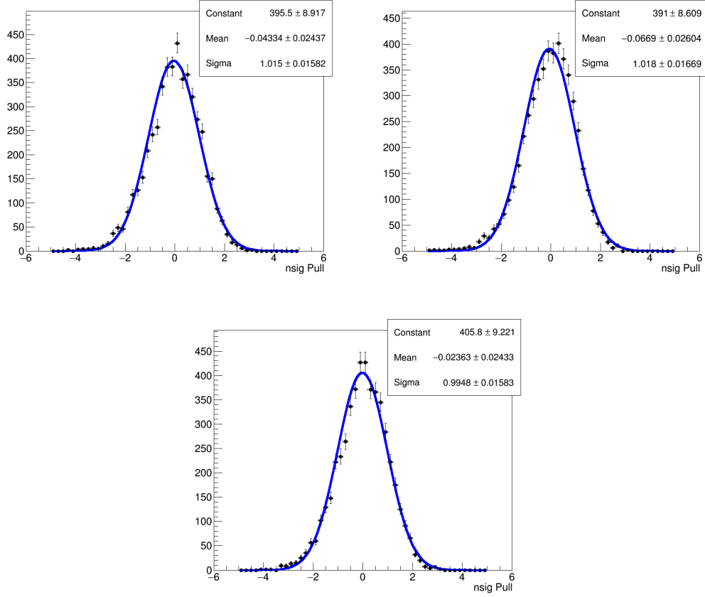
Figure 5-54: The B_s^0 pull distributions and the Gaussian fits in 0 - 30%, 30 - 90%, and 0 - 90% event centrality are shown respectfully above.
