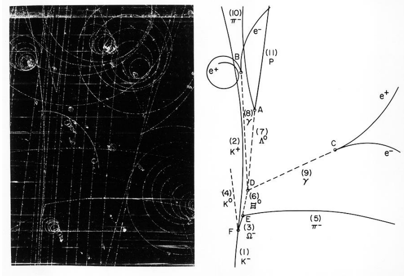
Figure 4-1: The photo of an \Omega^- baryon reconstructed from an event: K^-p \rightarrow K^0 K^+ \Omega^- \rightarrow \Xi^0 \pi^- \rightarrow \Lambda^0 \gamma \gamma \rightarrow \pi^- p taken from the bubble chamber of the group led by Nicholas Samios at BNL is shown above.
