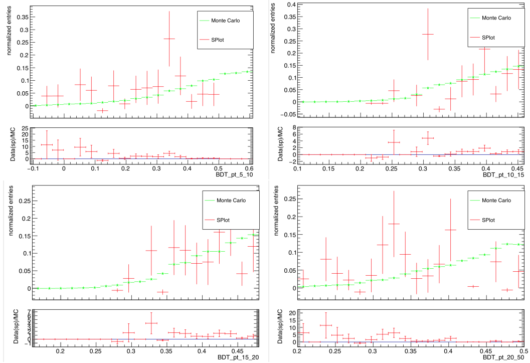
Figure 5-42: Comparison of B_s^0 BDT distributions in data (red) and MC (green) using the Splot method.
