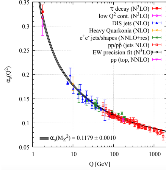
Figure 1-2: The running of the strong coupling constant \alpha_s in different experiments at different energy scales Q and the comparison with QCD calculations are shown above. Image from: [4]
