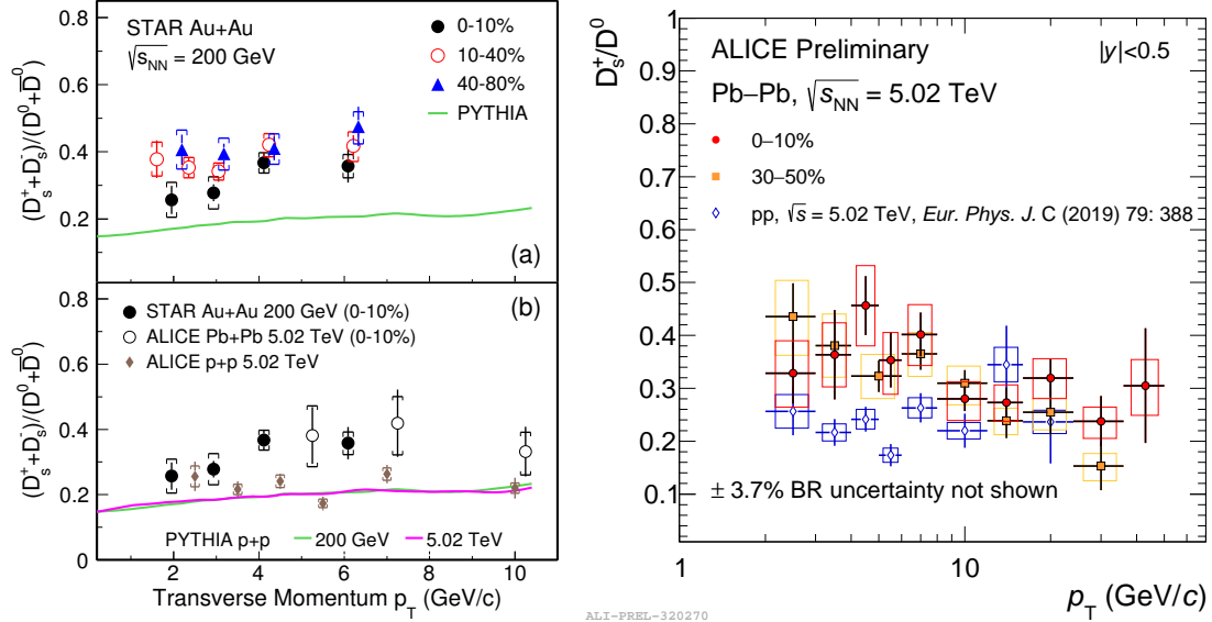
Figure 2-7: The fully reconstructed D_s^+/D^0 ratios in Au + Au measured by the STAR experiment at RHIC (left) and in PbPb the ALICE experiment at LHC (right) as functions of p_T are shown above.
