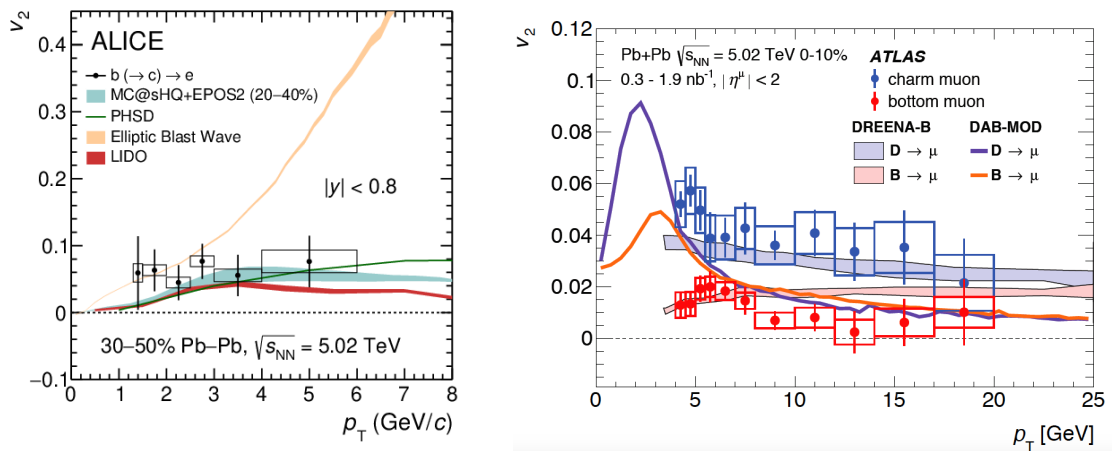
Figure 2-2: The v_2 of electrons from b-hadron decays as a function of electron p_T measured by the ALICE experiment (left) and the v_2 of muons from b-hadron decays as a function of muon p_T measured by the ATLAS experiment (right) are shown above.
