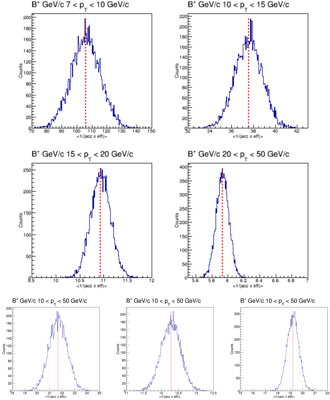
Figure 5-64: The distributions of B^+ \langle \frac{1}{\alpha \times \epsilon} \rangle for centrality in 0 - 90% in the p_T range of 7 - 10, 10 - 15, 15 - 20, and 20 - 50 GeV/c as well as 0 - 90%, 0 - 30%, and 30 - 90% in the p_T range of 10 - 50 GeV/c are shown above. The red dash lines are our nominal values for efficiency correction.
