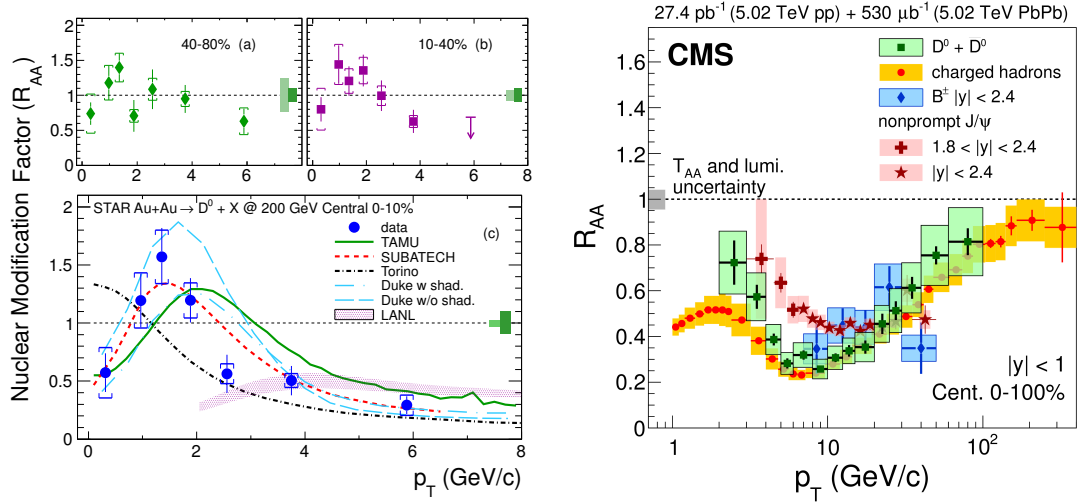
Figure 2-5: The fully reconstructed D^0 R_{AA} vs p_T with the STAR experiment in 0 - 10%, 10 - 40%, and 40 - 80% centrality at RHIC and D^0 , B^+ , non-prompt J/\psi , and charged hadrons R_{AA} vs p_T at 0 - 100% centrality with the CMS experiment at LHC are shown above.
