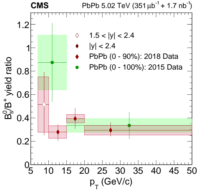
Figure 5-75: The comparison of B_s^0/B^+ as a function of p_T between the CMS 2018 PbPb datasets in centrality 0 - 90% (red) and the 2015 PbPb dataset in centrality 0 - 100% (green) is shown above.
