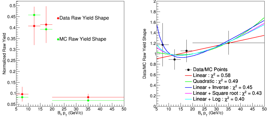
Figure 5-4: B_s^0 p_T normalized raw yields obtained in PbPb MC and Data are shown above on the top left panel. The data/MC ratio and different fitting functions: Linear (Red), Quadratic (Green), Linear + Inverse (Blue), Linear + Square Root (Purple), and Linear + Log (Cyan) and their \chi^2 are shown above on the top right panel. The bottom plots are the data/MC reweighed yields with different functions from the fit on the top right panel.
