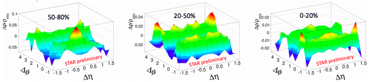
Figure 2-14: The 2D \Delta\eta \times \Delta\phi distributions of D^0 mesons and associated hadrons in Au + Au centrality 0 - 20%, 20 - 50%, and 50 - 80% at \sqrt{s_{NN}} = 200 GeV measured by the STAR experiment are shown above.
