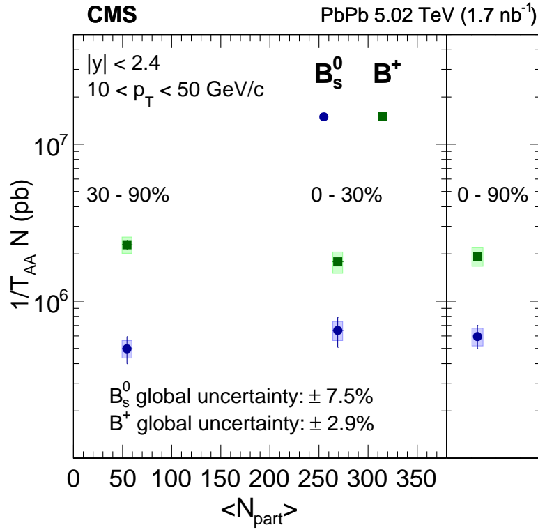
Figure 5-72: The measurement of B_s^0 and B^+ cross section \frac{1}{T_{AA}}N as a function of \langle N_{part} \rangle in different PbPb collision centralities within B-meson p_T from 10 - 50 GeV/c is shown above.
