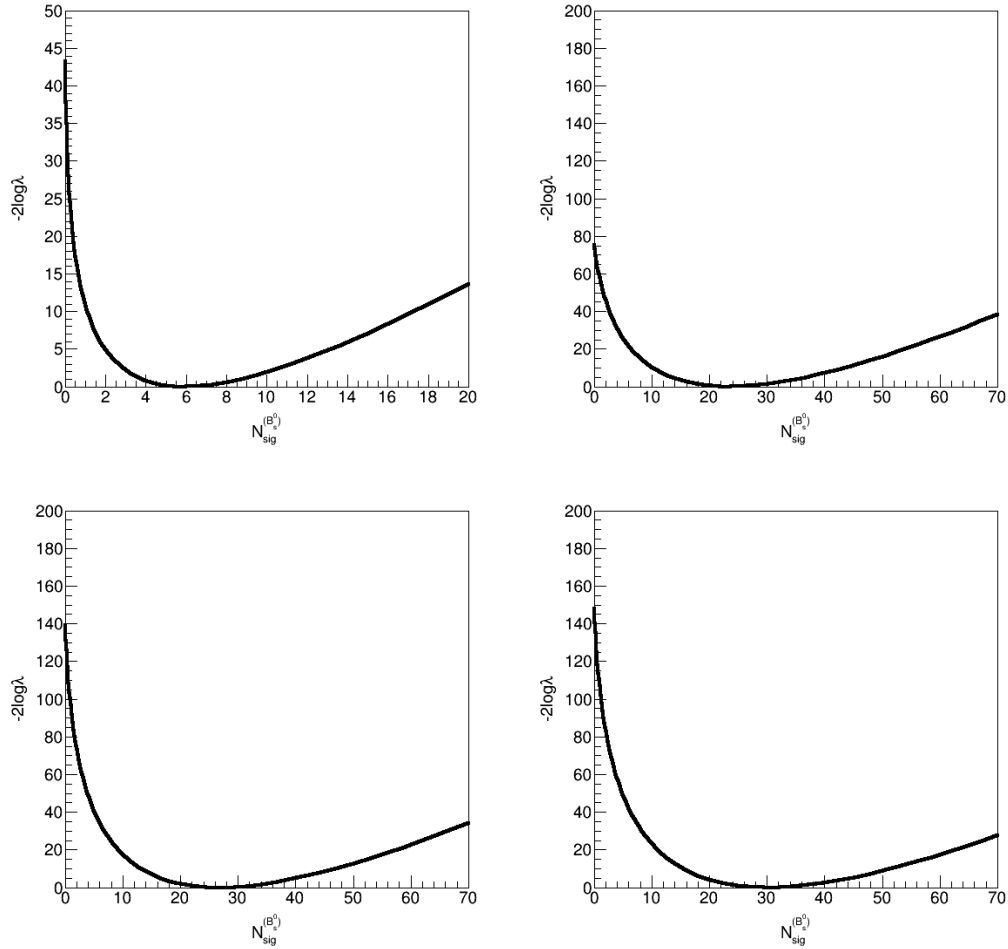
Figure 5-37: The significance vs signal yield for p_T bins from 7 – 10, 10 – 15, 15 – 20, and 20 – 50 GeV/c for 0 - 90% centrality are shown above
