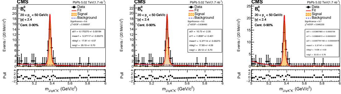
Figure 5-67: The Invariant mass fits to B_s^0 candidates for B_s^0 p_T from 20 - 50 GeV/c and centrality from 0 to 90% in 5.02 TeV PbPb. The background PDFs from left to right are first-, second-, and third-order polynomials.
