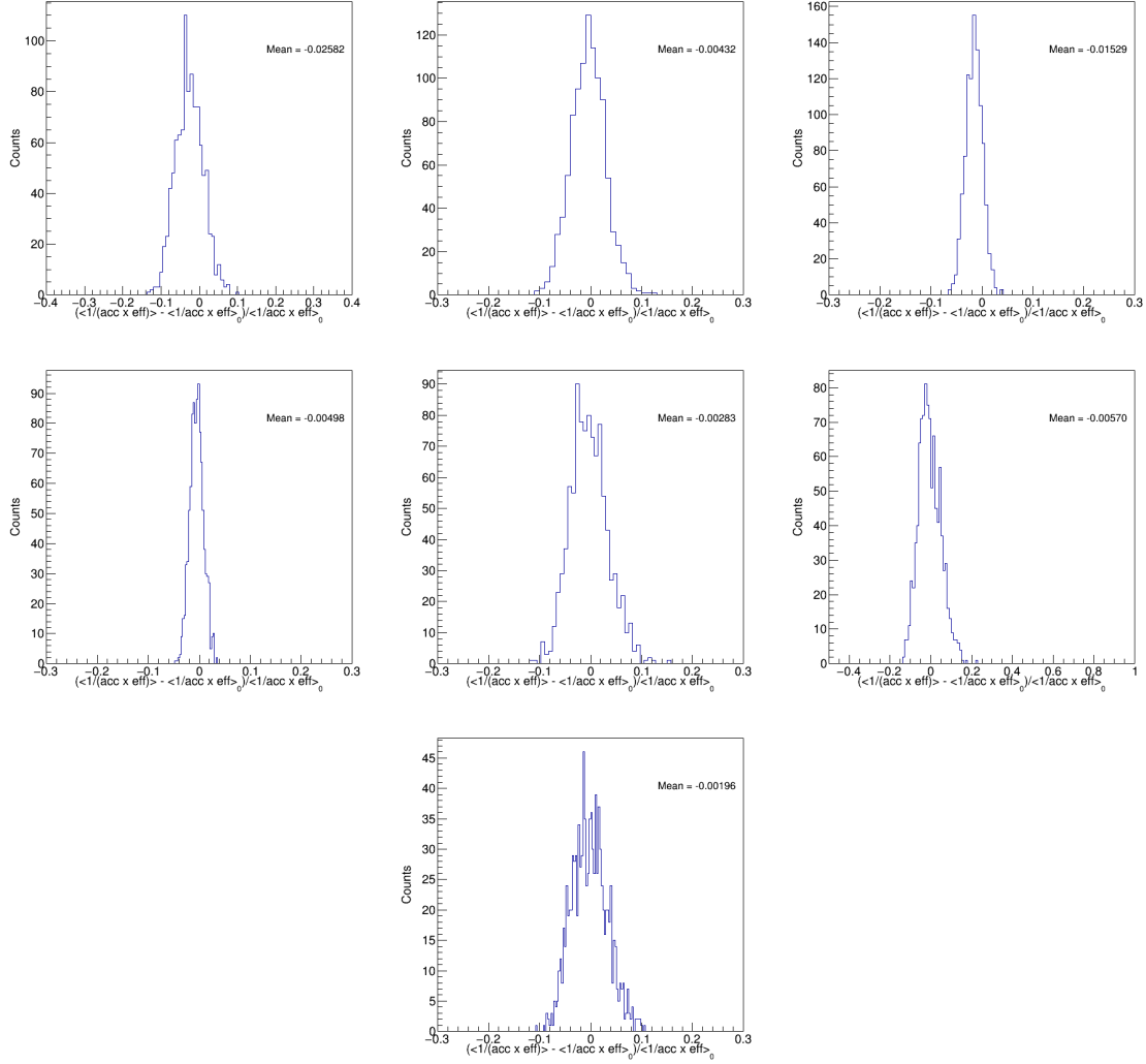
Figure 5-58: The percent deviation distributions of B^+ \langle \frac{1}{\alpha \times \epsilon} \rangle to RECO/GEN for the data-like randomly constructed MC samples in centrality 0 - 90% from 7 - 10, 10 - 15, 15 - 20, and 20 - 50 GeV/c as well as 0 - 90%, 0 - 30%, and 30 - 90% event centrality from 10 - 50 GeV/c are shown respectfully above.
