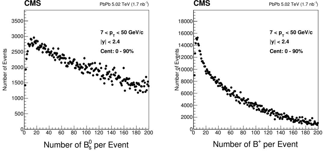
Figure 5-11: The number of reconstructed B-meson candidates per event distributions in the dimuon PbPb dataset for B_s^0 (left) and B^+ (right) are shown above. Multiple B-meson candidates are reconstructed in one event.
