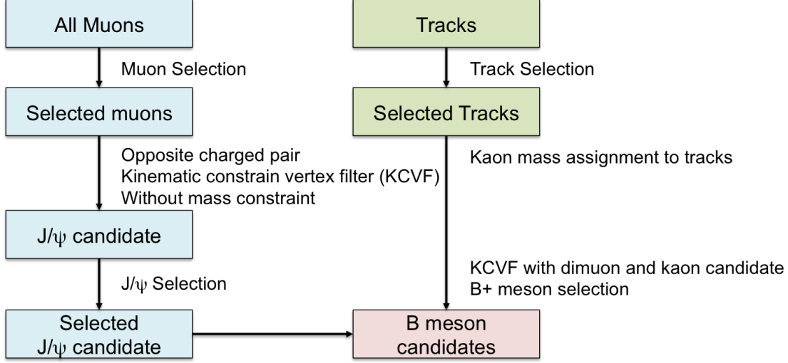
Figure 5-10: The schematic block diagram of the full reconstruction workflows for B^+ via the decay channel of B^+ \rightarrow J/\psi K^+ \rightarrow \mu^+ \mu^- K^+ in the Bfinder is shown above.
