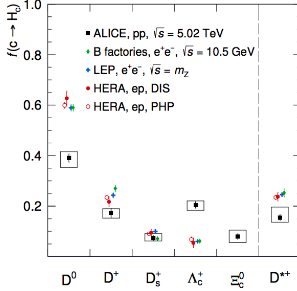
Figure 1-36: The charm quark fragmentation fraction to different charm hadrons species in e^+e^- , ep , and pp collisions are presented above. From the ALICE experiment, we can clearly see that the fragmentation fraction of D^0 has dropped by about 40% while the \Lambda_c^+ has enhanced by about a factor of 4. Therefore, the hadronization universality is clearly broken at the LHC energy in the charm sector.
