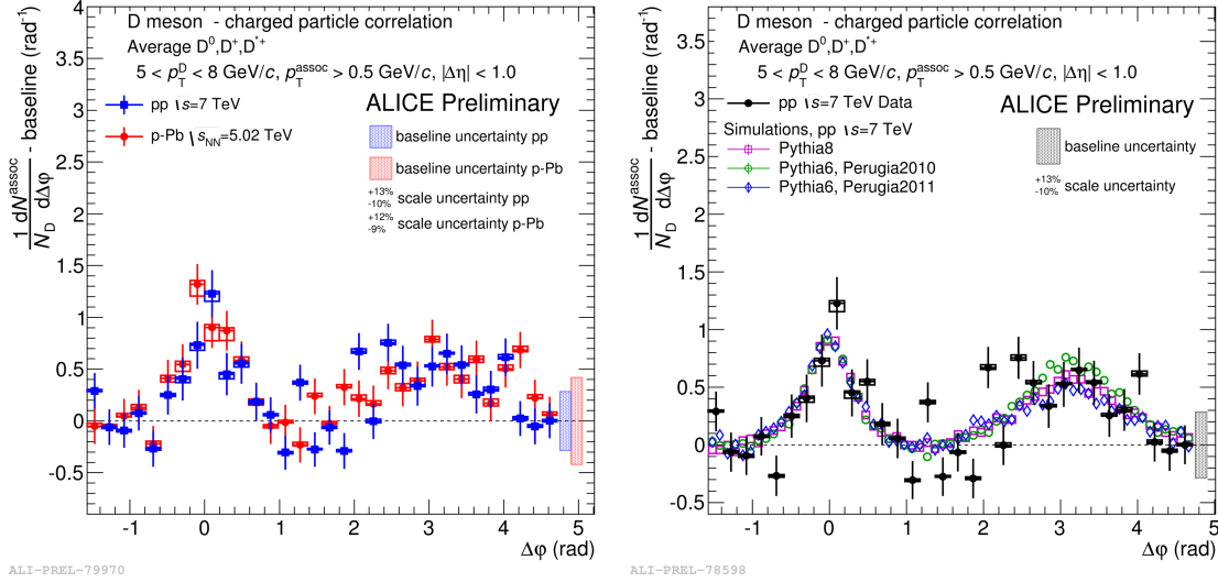
Figure 2-13: The ALICE D-hadron angular correlation in both pp (blue) and pPb (red) collision (left) and the comparison of pp data with PYTHIA calculations (right) are shown above.
