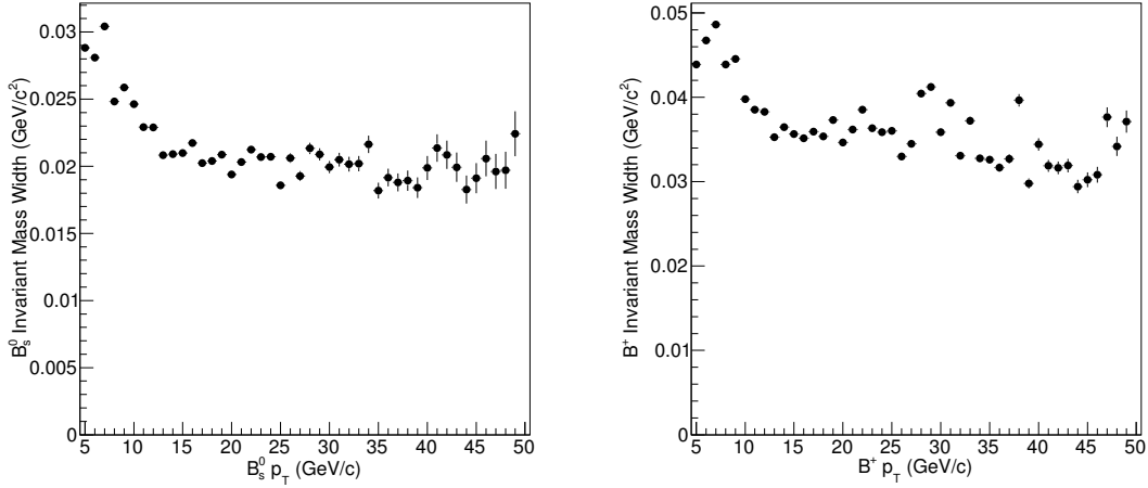
Figure 5-32: The signal B_s^0 (left) and B^+ (right) invariant mass widths as a function of p_T are shown above. We could see a rather large variation of the B-meson mass width from low to high p_T .
