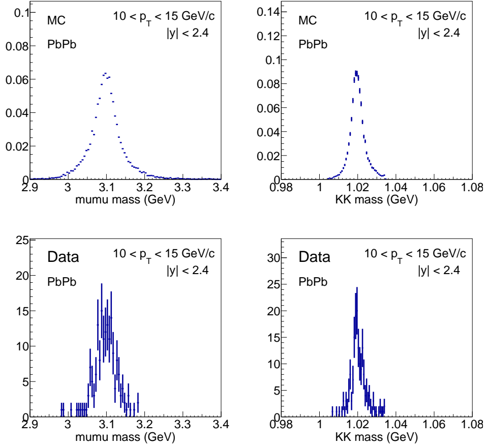
Figure 5-25: The J/\psi (left) and \phi (right) meson mass distributions after applying \text{BDT} > 0 for MC (top) and data (bottom) in B_s^0 analysis are shown above.
