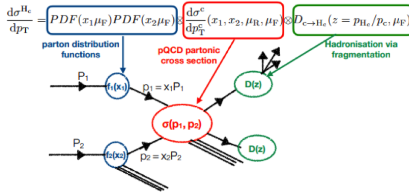
Figure 1-3: The QCD factorization theorem applied to study charm hadron production in a pp collision event involving soft and hard processes is shown schematically above.
