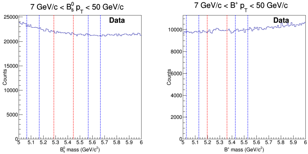
Figure 5-18: The definitions of signal (red band) and background region (blue band) in the fully reconstructed B-meson invariant mass distribution for B_s^0 (left) and B^+ (right) are shown above.
