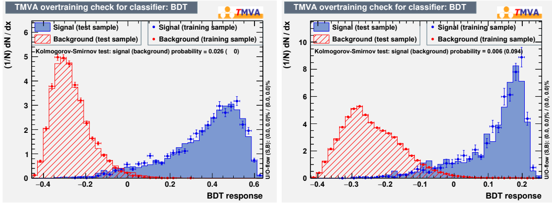
Figure 5-23: The Kolmogorov-Smirnov overtraining tests on the signal (blue) and background (red) in B_s^0 (left) and B^+ (right) at 10 < p_T < 15 \text{ GeV}/c are shown on the right. These plots suggest that they both pass the tests.
