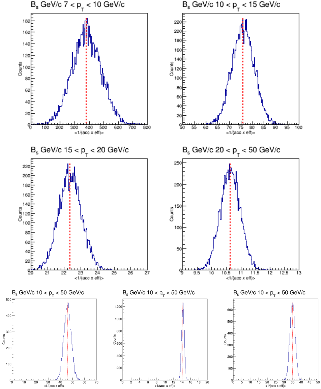
Figure 5-63: The distributions of B_s^0 \langle \frac{1}{\alpha \times \epsilon} \rangle for centrality in 0 - 90% in the p_T range of 7 - 10, 10 - 15, 15 - 20, and 20 - 50 GeV/c as well as 0 - 90%, 0 - 30%, and 30 - 90% in the p_T range of 10 - 50 GeV/c are shown above. The red dash lines are our nominal values for efficiency correction.
