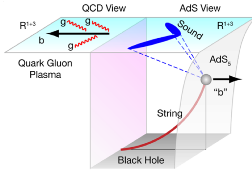
Figure 1-38: The schematic demonstration of ADS/CFT picture: a quark loses energy in the QGP medium holographically due AdS/CFT drag force.
