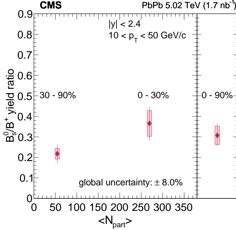
Figure 5-74: The measurement of B_s^0/B^+ as a function of p_T is shown above.
