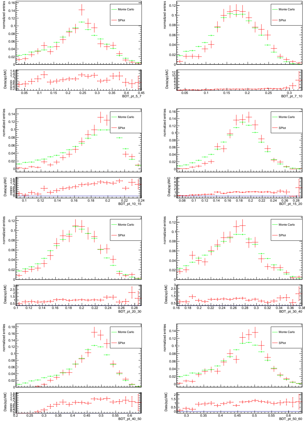
Figure 5-43: Comparison of B^+ BDT distributions in data (red) and MC (green) using the Splot method.
