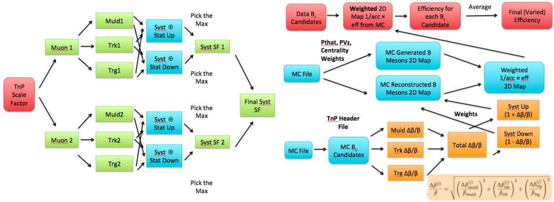
Figure 5-62: The schematic block diagrams demonstrating the calculations of the uncertainties on tag-&-probe scale factors (left) and the asymmetric systematic uncertainties due to muon efficiency on the efficiency correction factor (right) are shown above.
