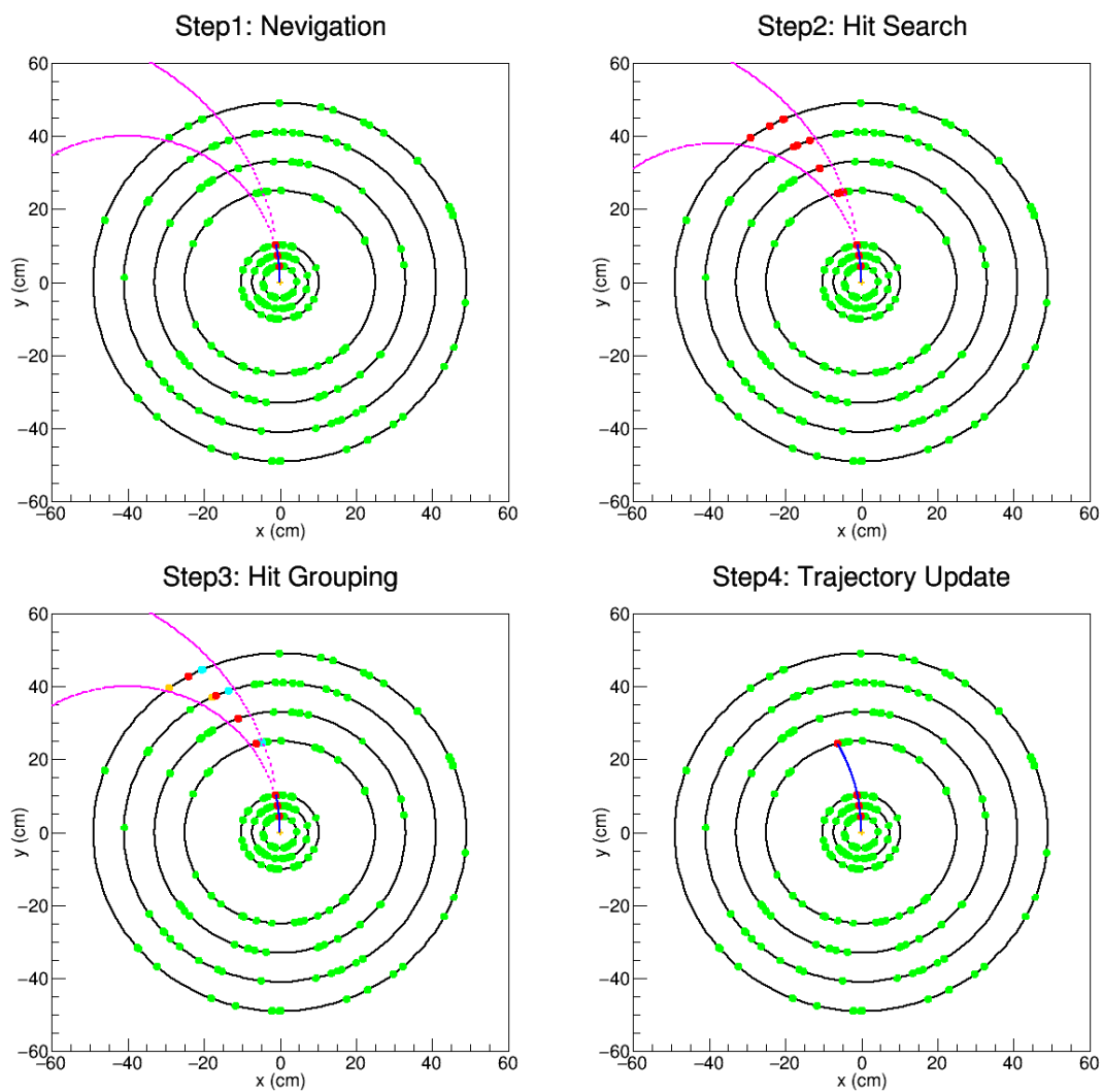
Figure 4-10: The four schematic plots demonstrating each of the four steps for track finding are shown respectfully above.
