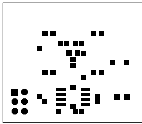
Figure 5: Top Soldermask Layer
