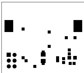
Figure 6: Bottom Soldermask Layer
