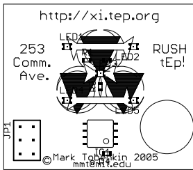
Figure 2: Bottom Copper Layer
