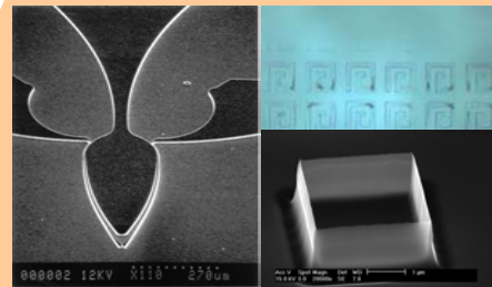
Microfabrication Nanofabrication Thermal Nanolithography
