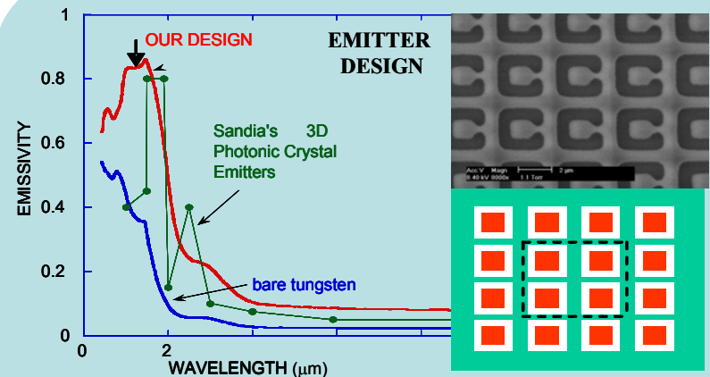
Emission Control, Efficient Light Bulbs Thermophotovoltaics Energy Conversion
