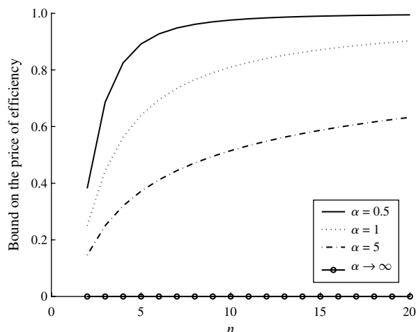
Figure 3 Bounds on the Price of Efficiency of \alpha -Fair Allocations for Different Values of the Inequality Aversion Parameter \alpha Implied by Theorem 2
