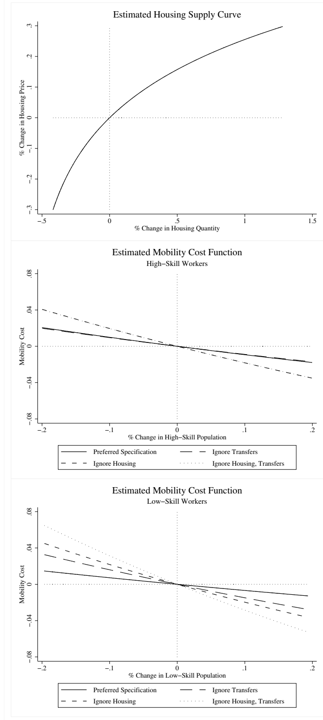
Figure 6: GMM Estimates
