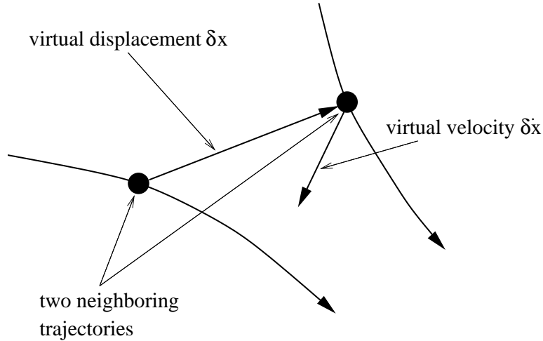
Fig. 1. Virtual dynamics of two neighboring trajectories
