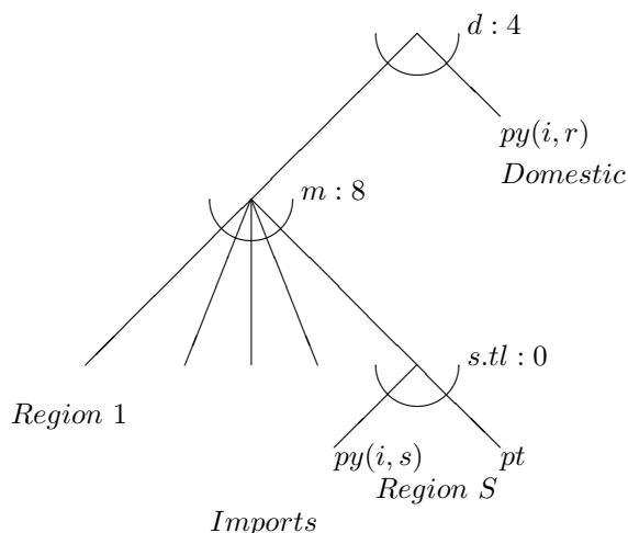
Fig. 6. Armington aggregation
