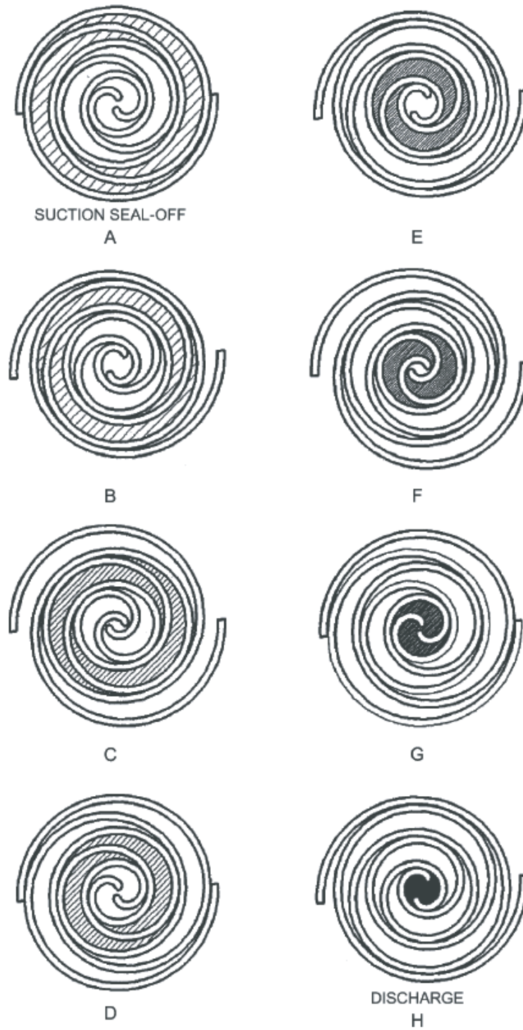
Figure 1-5: Compression cycle for a scroll compressor[26].
