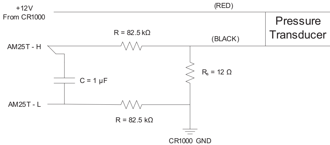
Figure 2-3: Typical pressure transducer circuit diagram.
