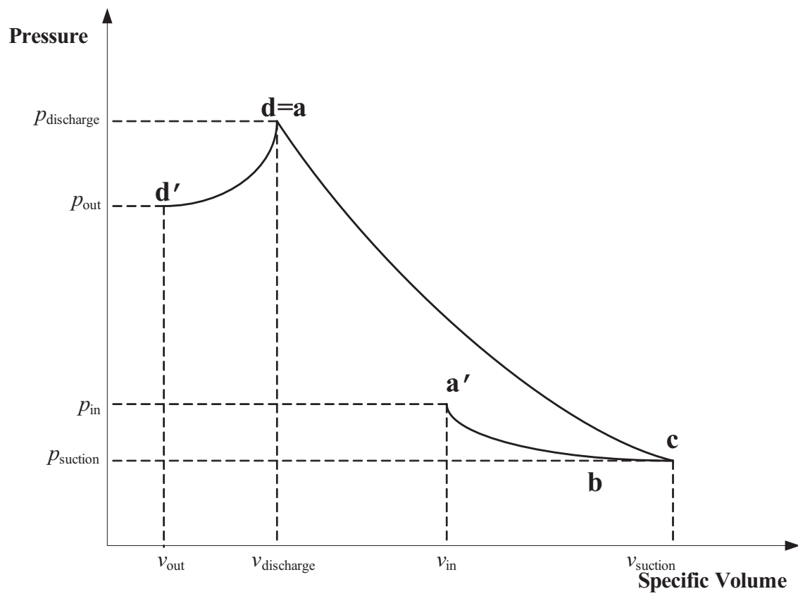
Figure 4-3: Pressure-specific volume for the compression cycle.
