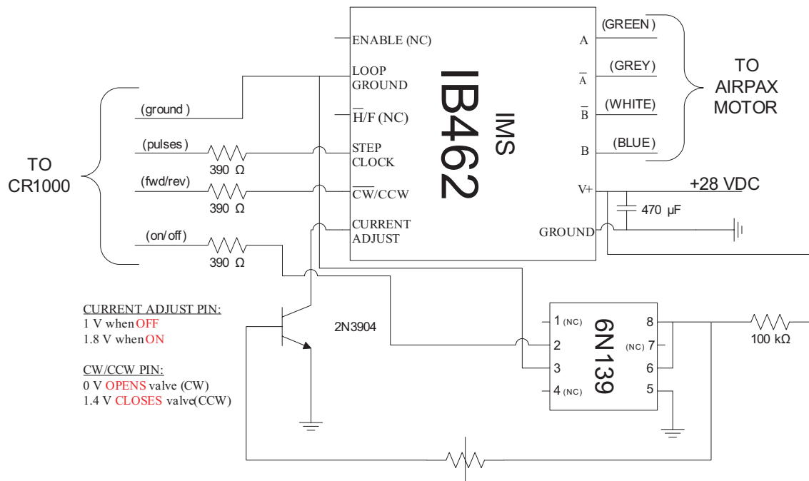
Figure 2-12: Control valve wiring; valve side ( typical of 3 ).
