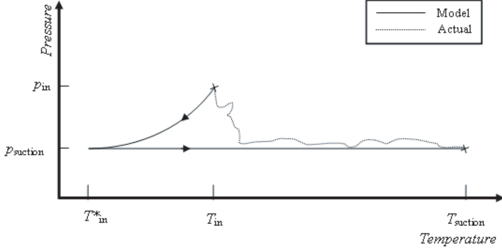
Figure 4-5: Pressure-temperature diagram of suction side pressure drop.
