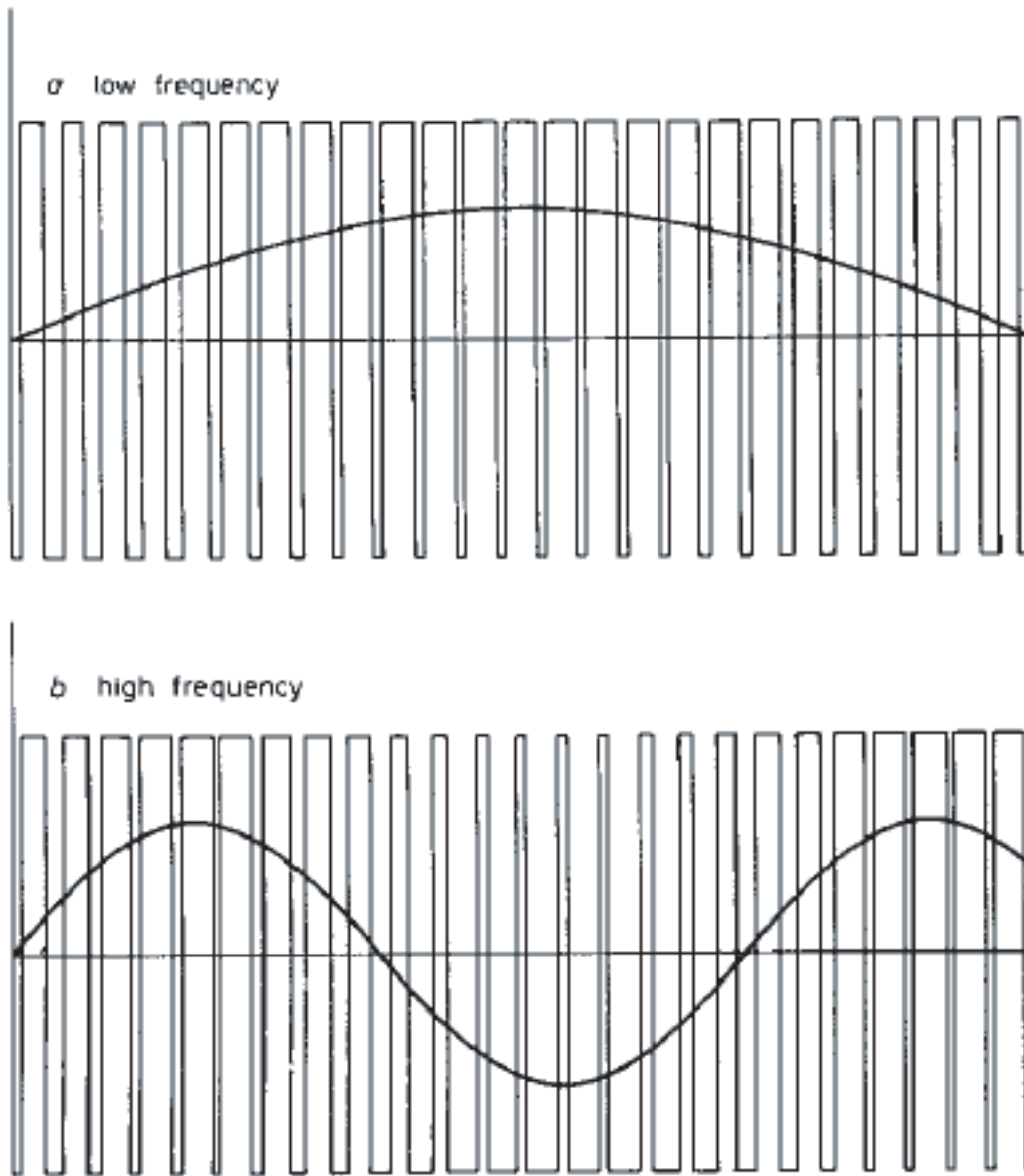
Figure 2-19: Frequency variation using PWM[11].
