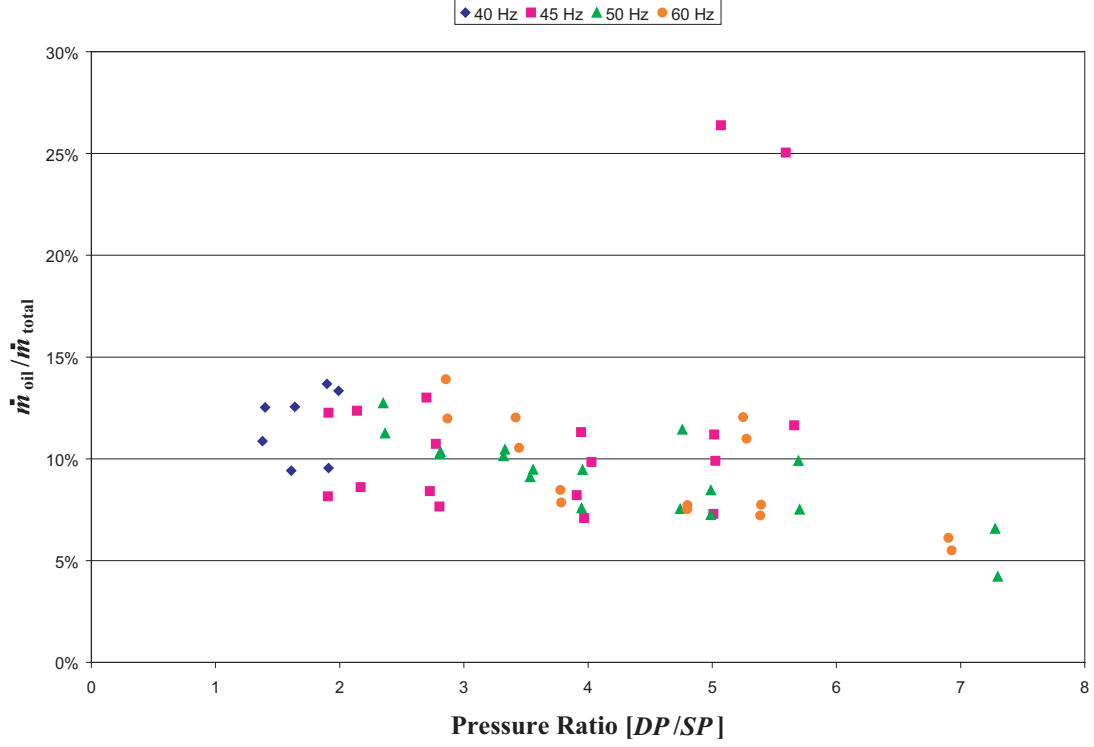
Figure 3-7: Inferred mass flow rate of oil as a percentage of total mass flow.
