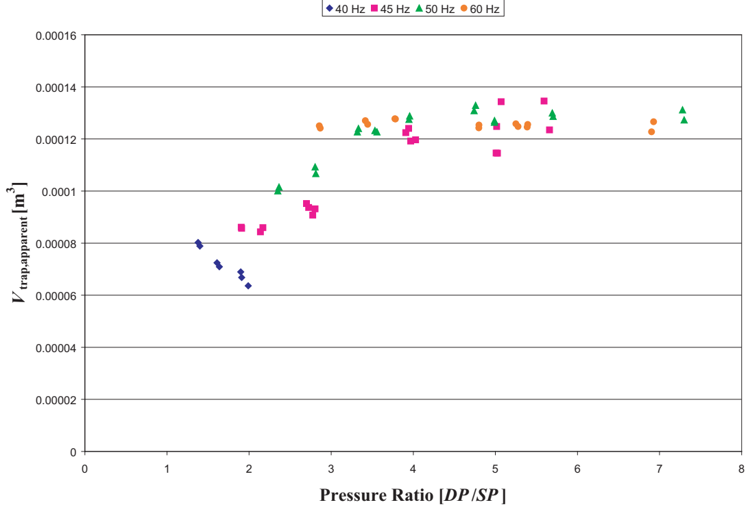
Figure 3-10: Volumetric efficiency for experimental data.
