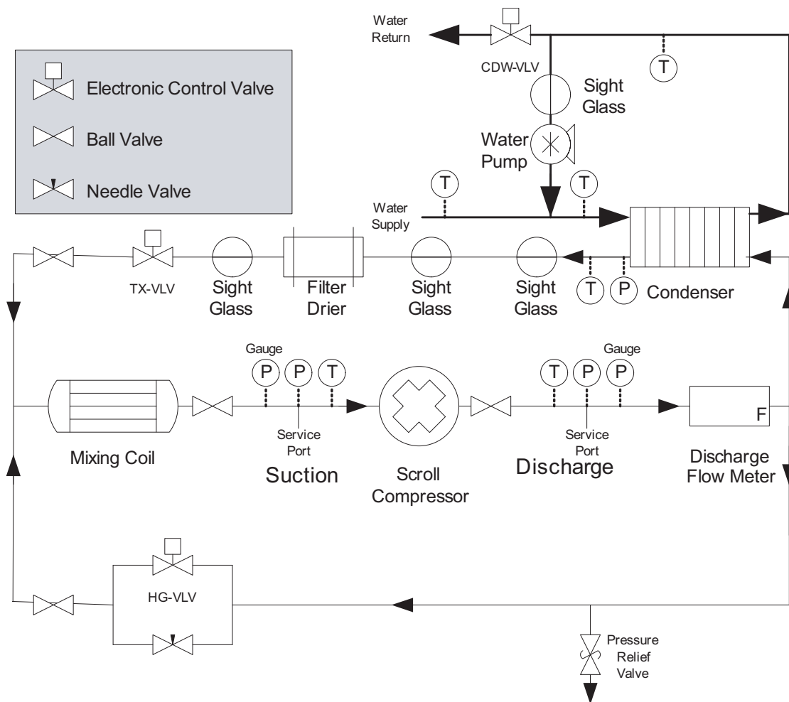
Figure 2-2: Flow diagram of the modified system.
