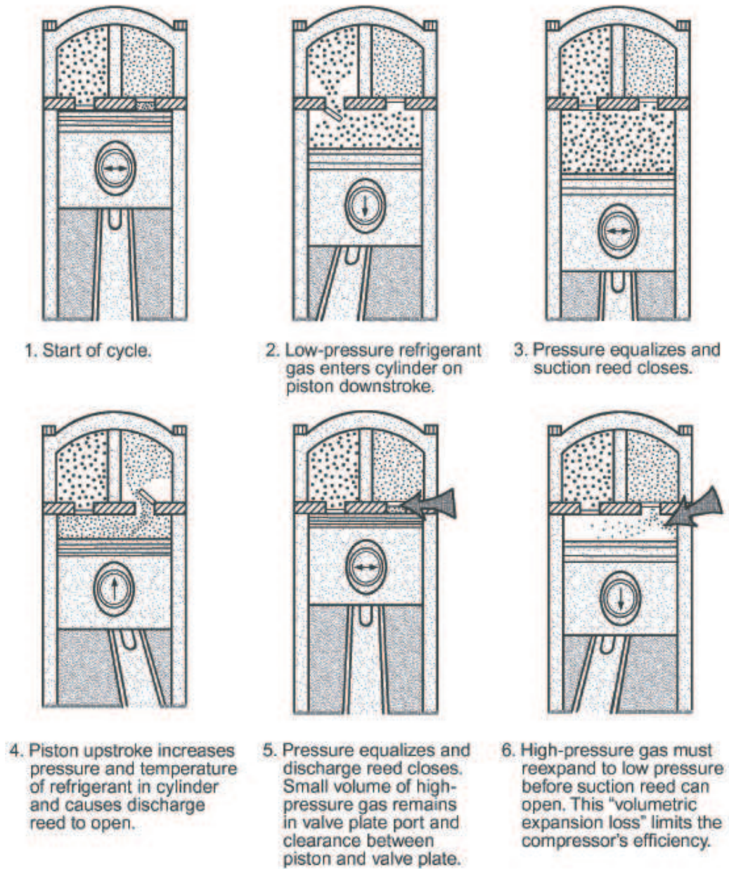
Figure 1-4: Compression cycle for a reciprocating compressor[2].
