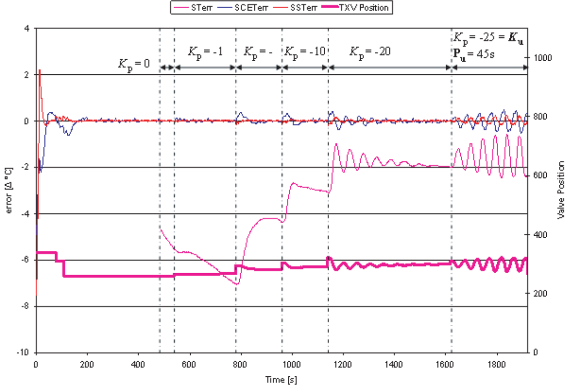
Figure 2-13: Ziegler-Nichols tuning of the thermal expansion valve.
