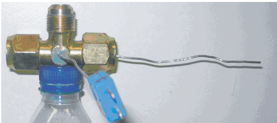
Figure 2-8: Condenser water outlet stream temperature probe.
