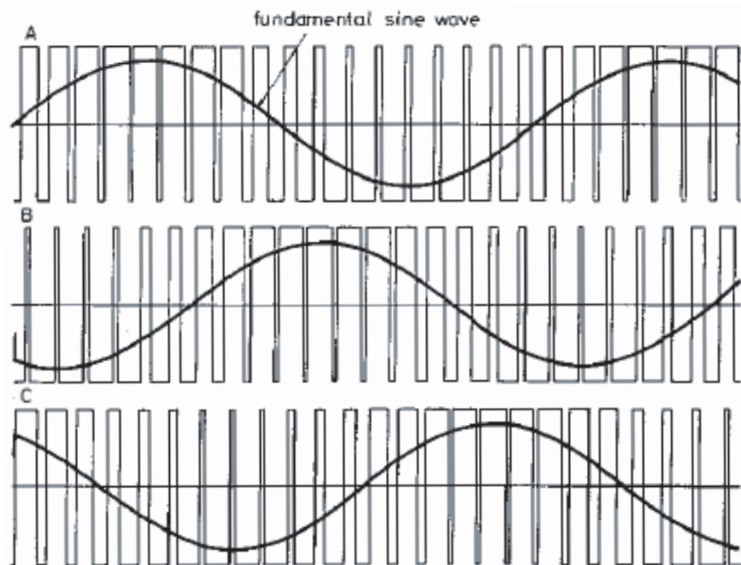
Figure 2-20: 3 Phase operation of PWM scheme[11].
