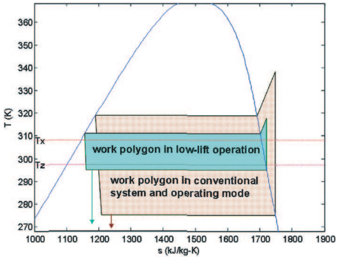
Figure 1-3: Typical work polygon for low-lift operation [4].
