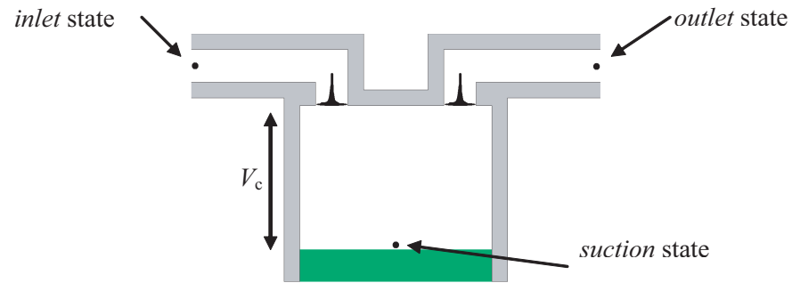
Figure 4-1: Reciprocating compressor cylinder just before compression.
