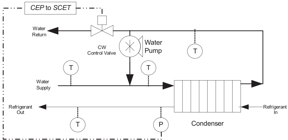
Figure 2-9: Condenser water control loop.
