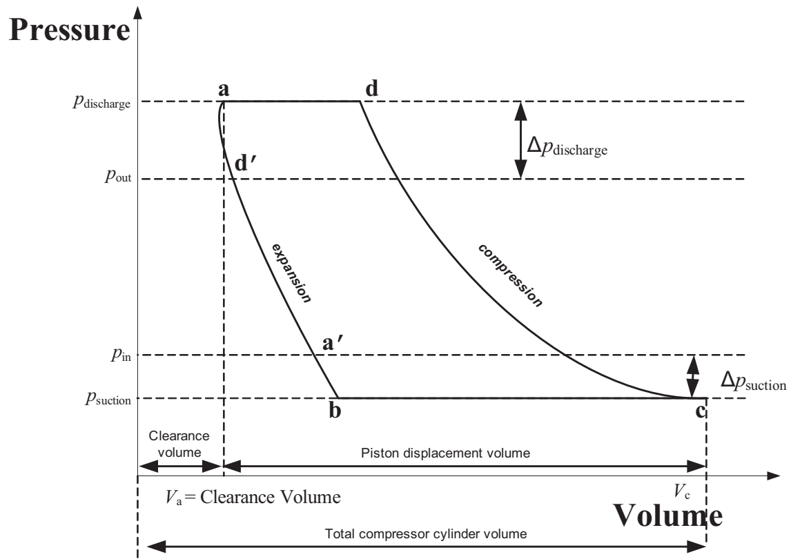
Figure 4-4: Pressure-volume diagram for the compression cycle.
