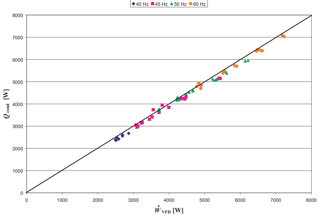
Figure 3-3: Compressor input power versus condenser heat rate.
