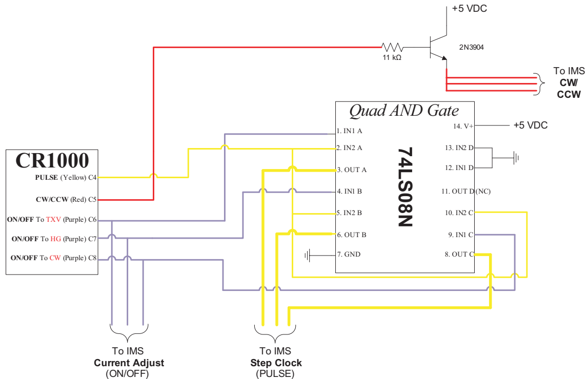
Figure 2-11: Control valve wiring diagram; CR1000 side.
