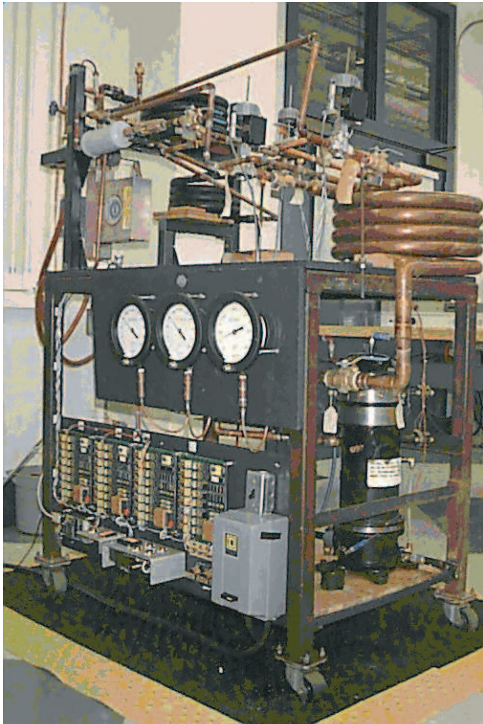
Figure 2-1: Otten/Wilson calorimeter [23].
