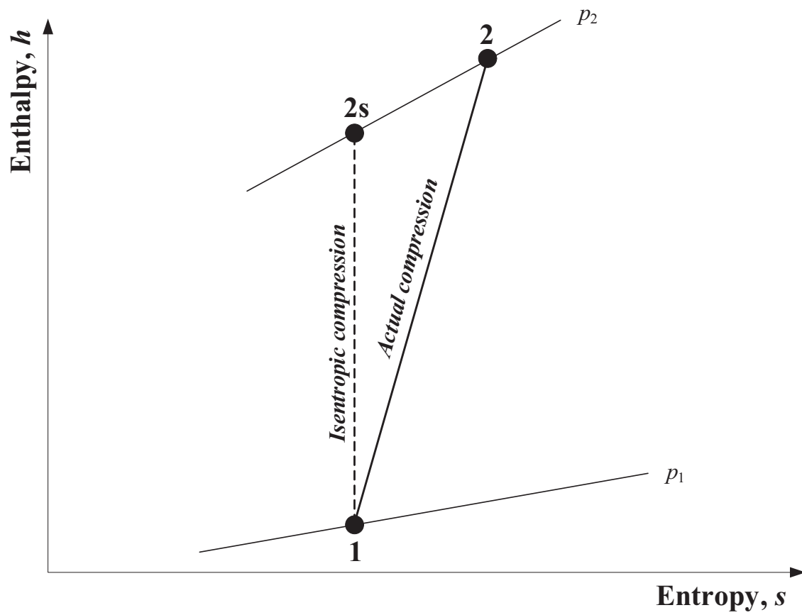
Figure 1-6: Isentropic compression versus actual compression.
