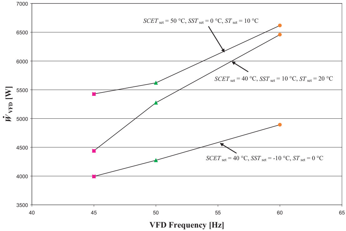
Figure 3-2: Compressor input power for three different conditions.
