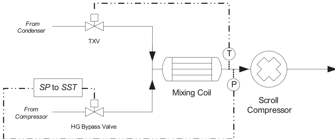
Figure 2-10: Hot gas bypass and thermal expansion valve control loop.
