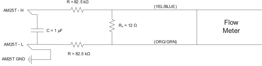
Figure 2-4: Mass flow meter wiring diagram.
