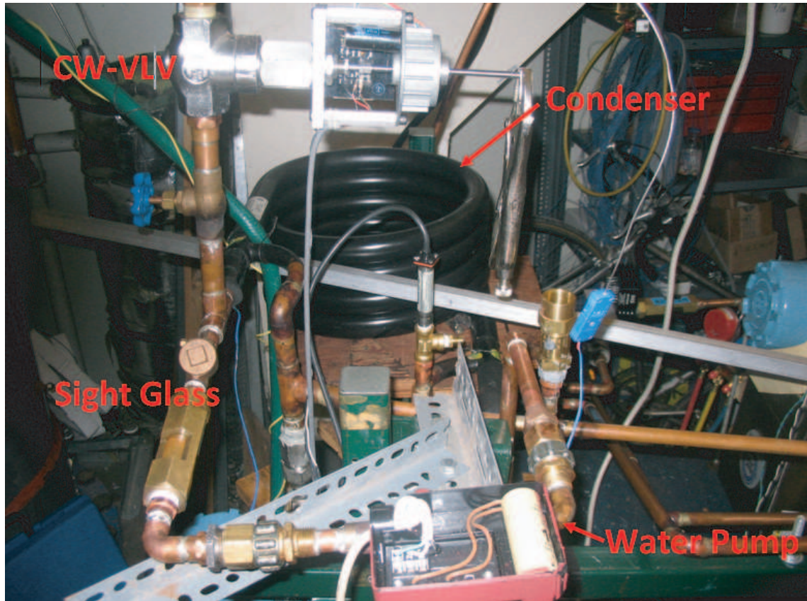
Figure 2-6: Condenser and water circulation pump.
