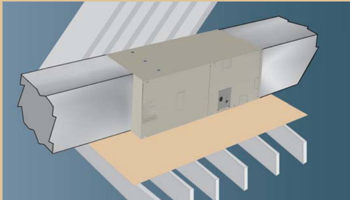
Horizontal Configuration for all multi-poise air handlers
