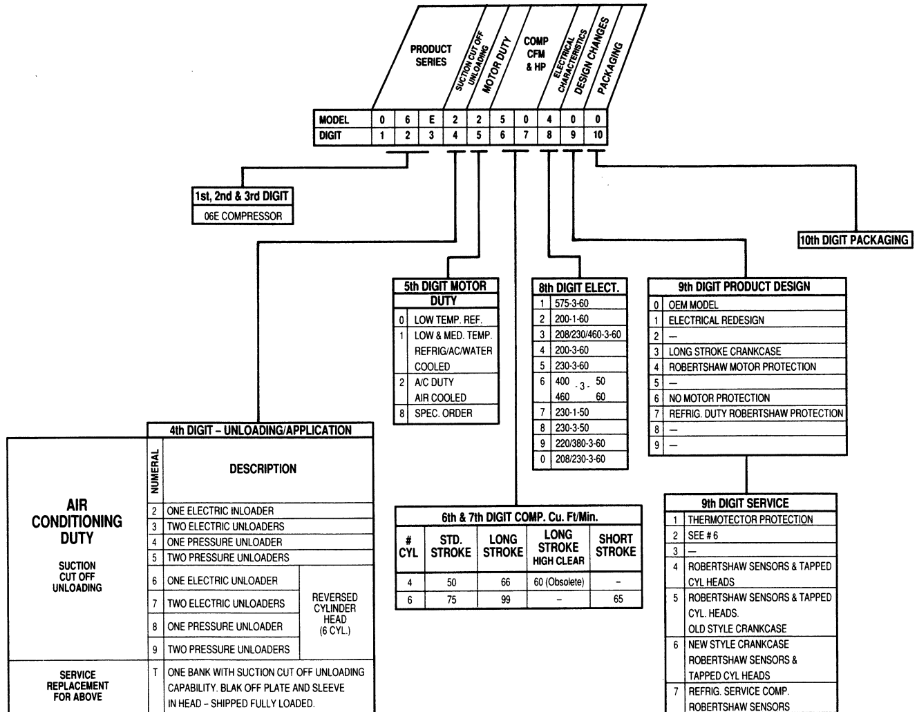
06E COMPRESSOR MODEL SIGNIFICANCE CHART 06ET W/SUCTION CUTOFF UNLOADING
