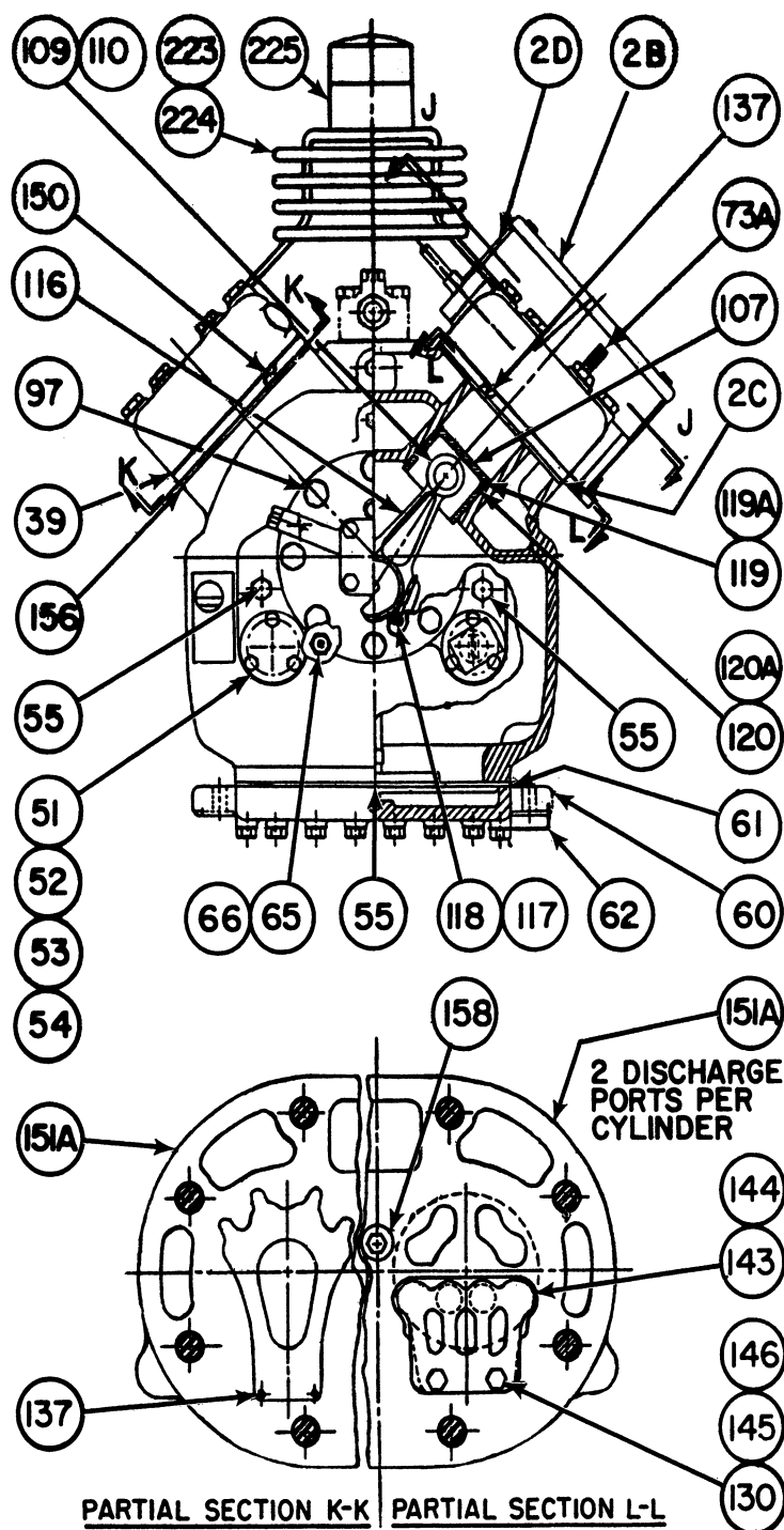
06ER/EY (4 CYLINDER)
