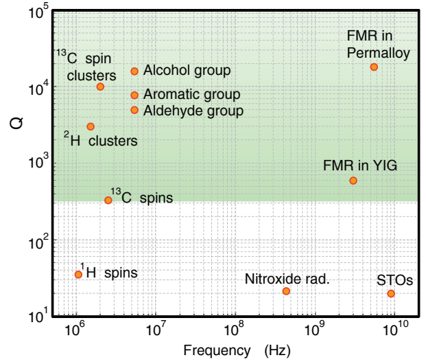
Fig. S15. Q-value vs f for different quantum metrology experiments. In this scatter plot we show representative examples the Q-values from different signal sources plotted against their native frequency f (see Table S1). Note that in our experiments, we could obtain gains in Q by about 10^4 via quantum interpolation, and this might open up the metrology of several signals (green shaded region) that were hitherto extremely challenging.
