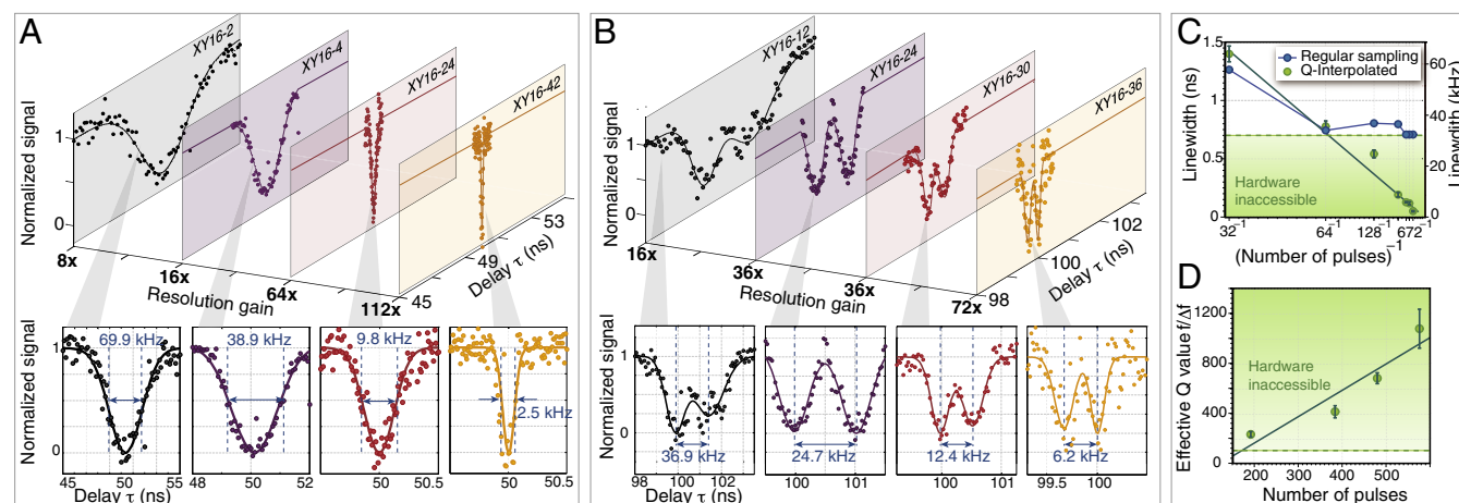
Fig. 2. High-resolution sensing and spectroscopy. (A) Detection of the spurious harmonic of an AC magnetic field via quantum-interpolated XY16 sequences. The incoherent external magnetic field is generated by an AC current at f_{AC} = 2.5 MHz through a 20\text{-}\mu\text{m} wire located in the vicinity of the NV center. Our hardware limitation ( \Delta\tau = 1 ns) translates in a frequency resolution of \Delta f_{AC} = 35.3 kHz, and would cause a severe suppression of the detected signal as its linewidth decreases linearly with the number of \pi -pulses. In the rightmost image, quantum interpolation enables supersampling at 8.9 ps (an effective boost of 112), which still permits to resolve clearly a linewidth of 2.5 kHz. (B) Detection of incoherent AC magnetic fields with two distinct frequencies. Quantum interpolation with a maximum of 672 \pi -pulses allows for a resolution gain of a factor 72 and faithfully reconstructs the AC fields, even if the two frequencies are not resolved by regular XY16 sequences with our timing resolution. (C) Linewidth of the detected AC magnetometry signal (from A) with regular sampling (blue) and supersampling (green). The error bars are residuals to a Gaussian fit. (D) Sensing quality factor Q = f/\Delta f extracted from B. Conventional dynamical decoupling sequences can only achieve Q \leq 100 . This limit can be surpassed with quantum interpolation, scaling linearly with number of pulses, to reach Q \approx 1,000 .
