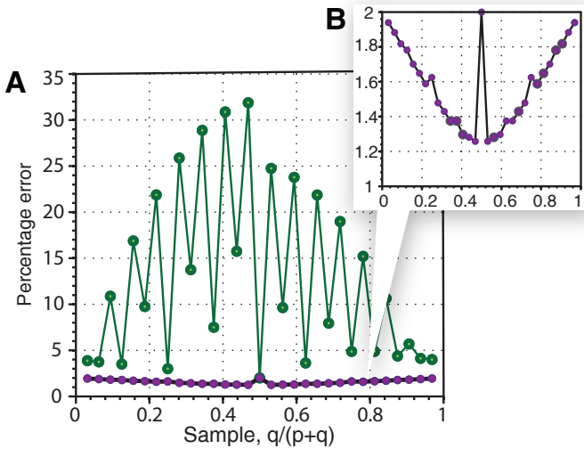
Fig. S12. Performance of optimal quantum interpolation. We represent the percentage errors (specified in units of \Delta\tau/4\tau ) of the construction of a supersample [q/(p+q)]\Delta\tau via quantum interpolation using two hardware defined unitaries \mathcal{U}(\tau_k) and \mathcal{U}(\tau_{k+1}) , and an time resolution of \Delta\tau . Here we consider N = 16 cycles of the CPMG sensing sequence, giving a total of 32 possible supersamples. The error is calculated from the effective area under the time domain error function \epsilon following Fig. S7. (A) The green points denote the naive construction \mathcal{U}(\tau_k)^p \mathcal{U}(\tau_{k+1})^q , where the errors accumulate very quickly. The purple line and points instead denote the case of the optimal construction following Fig. S9, where the error of all samples is less than the half-way-sample (zoomed in the inset (B)). Hence the optimal construction can reliably produce different supersamples with low effective error (see also Fig. S13).
