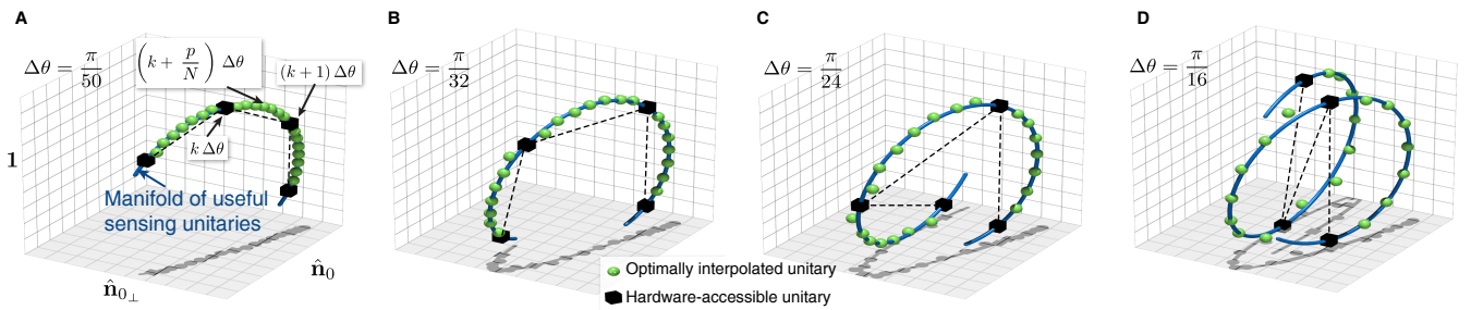
Fig. S5. Geometric picture of Quantum interpolation. We represent unitaries as points in the 3D space spanned by the operators \{1, \hat{\mathbf{n}}_0, \hat{\mathbf{n}}_{0\perp}\} . The projection of the missing dimension, (\hat{\mathbf{n}}_0 \times \hat{\mathbf{n}}_{0\perp}) is small and only causes the norm of the vector to be smaller than one. The blue line indicates the ideal manifold of sensing unitaries, while the black squares represent the hardware accessible unitaries. Without quantum interpolation, the signal obtained by classical interpolation corresponds to the dashed black line. The green circles are the unitaries resulting from quantum interpolation following the optimal construction, where one seeks to construct the ideal unitaries \mathcal{U}_{|0\rangle}^N(\pi - \delta_0 + k\Delta\theta) , with \delta_0 \in \{-\Delta\theta, 0, \Delta\theta, 2\Delta\theta\} . Here N = 8 leading to 8 supersamples in each \Delta\theta interval, and we set \alpha_j = 0.1 rad. The success of quantum interpolation is evident as the interpolated unitaries closely matches the target unitaries over the entire manifold, even for increasing values of \Delta\theta (left to right panels).
