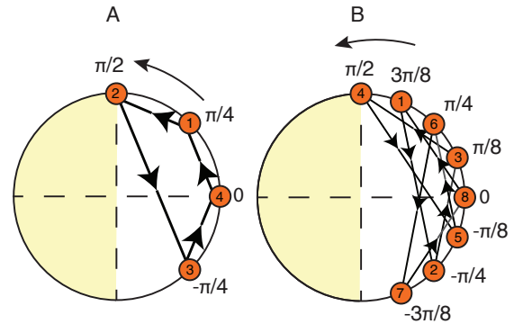
Fig. S9. Geometric representation of the optimal construction, for two particular sampling times (A) \Delta\tau/4 and (B) 3\Delta\tau/8 . We represent the desired sample as phasor at angle \pi \times \text{sample} on a circle (orange circles). The left half plane (LHP) of the circle (shaded) is considered forbidden. Starting with an initial loop counter m = 0 , we propagate the algorithm by forming the phasor m \rightarrow m + \text{sample} (arrows); and so long as we don't pass into the LHP we assign to this the operator \mathcal{U}(\tau_k) . In the opposite case, we assign \mathcal{U}(\tau_{k+1}) , and reflect the phasor about the origin. The algorithm ends when we finally return to the starting position. The numbers in the orange circles indicate the progression of the algorithm. This geometric representation also allows an intuitive understanding of why the error of all samples is almost the same (see Fig. S12).
