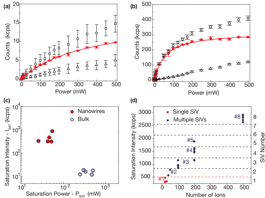
Fig. 4. Single SiV - fluorescence rates in bulk diamond and nanowires. Measured fluorescence rates as a function of laser excitation power for single SiV - centers in (a) bulk diamond and (b) a nanowire. Open black squares are raw counts; hollow black triangles are background; and filled red circles are normalized SiV - counts. Backgrounds were measured, respectively, in an empty zone of the bulk with no SiV - , and in a nanowire not implanted with silicon ions. (c) Single SiV - optical properties ( P_{sat} and I_{sat} ) for several nanowires in the array (red circles) compared to example single SiV - centers in the bulk (blue open circles). (d) Estimated number of SiV - defects created per nanowire, determined from measured values of I_{sat} . Red circles indicate single SiV - centers.
