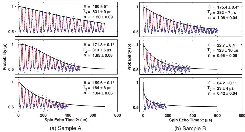
FIG. 2. (Color online) Example Hahn-echo measurements of ensemble NV electronic spin decoherence and dependence on static magnetic field orientation: (a) sample A with NV density \approx 3 \times 10^{13} \text{ cm}^{-3} and N density \approx 10^{15} \text{ cm}^{-3} ; and (b) sample B with NV density \approx 1 \times 10^{14} \text{ cm}^{-3} and N density \approx 5 \times 10^{15} \text{ cm}^{-3} . Clearly seen in this data is a sharp decrease in the ensemble NV coherence lifetime T_2 as the B_0 field is misaligned from the NV electronic spin axis and as the paramagnetic impurity level increases. For each data plot, the left vertical axis indicates the measured probability for NVs in the ensemble to be in the m_s=0 state at the end of a Hahn-echo experiment, as a function of the echo time \tau , the black line is a fit to \exp[-(\tau/T_2)^n] to the overall Hahn-echo-signal envelope, where the exponent n is a fit parameter and the long term baseline is taken to be 0.5 (the mixed spin state); and the errors in \theta , T_2 , and n are given by one-standard-deviation confidence intervals of the fit. The red line is a fit to the observed echo-signal modulations, which are collapses and revivals of NV spin coherence induced by precession of the natural abundance ^{13}\text{C} nuclear-spin bath in applied, hyperfine and dipolar magnetic fields.
