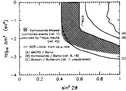
Fig. 3. The 90% confidence level contour for MACRO data for exclusion of large mixing parameters. No lower limit for parameters is shown since the data are consistent with no mixing at the 90% confidence level. Also shown in the plot are previous limits which are calculated under similar assumptions to those used for the MACRO limit along with the region allowed for parameters based on the Kamiokande analysis for contained events. (Note that the limit reported by Baksan using the Butkevich flux assumes the systematic error on the flux is \pm 10\% . A limit also exists for IMB data but using different assumptions on the flux [10].)
