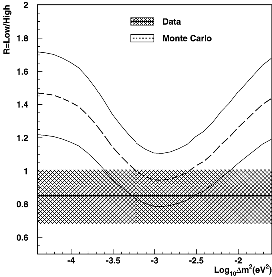
Fig. 6. Low energy events over high energy events as a function of \Delta m^2 : the area between the solid lines includes a 17% systematic (the error is not Gaussian, see text). The hatched band represents the real data.
