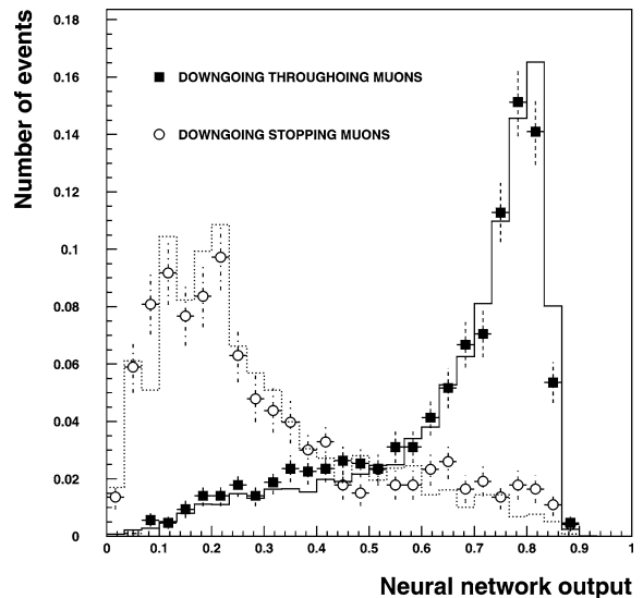
Fig. 2. Neural network (NN) output for down-throughgoing muons: real data (black squares) and Monte Carlo expectations (continuous line). NN output for downward going stopping muons: real data (empty circle) and Monte Carlo expectations (dotted line).
