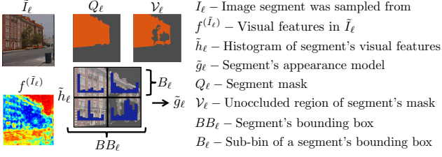
Figure 4: Notation for our likelihood model. Here we depict our model for the visual appearance of a building segment.
