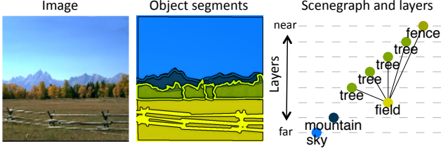
Figure 2: We model a scene as a layer-world collage of objects. Object support relationships are represented in a “scenegrph”. For example, the scenegrph above indicates that the trees are supported by the field.
