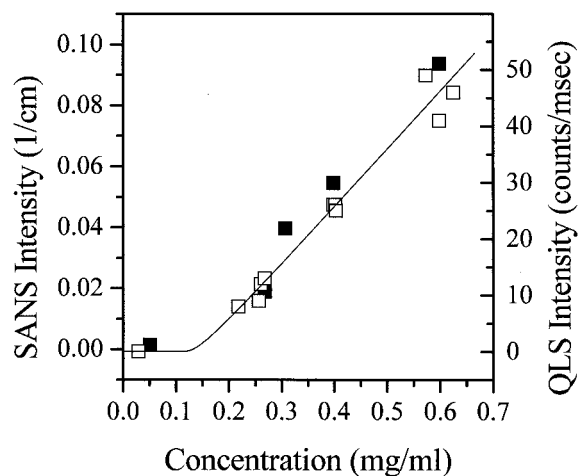
Fig. 4. SANS and QLS scattering intensities as functions of concentration at 4^\circ\text{C} . ( \blacksquare , SANS forward cross section I_0^b ; \square , QLS intensity normalized so as to overlay with SANS data. The solid line represents the theoretical prediction for c^* = 0.15 mg/ml and m_0 = 29 ).
