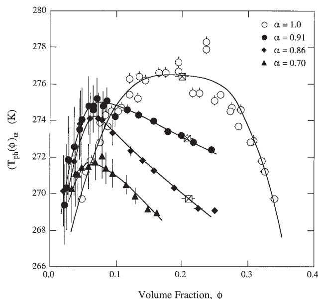
FIG. 4. The constant \alpha sections (cloud-point curves) of the coexistence surface of \gamma_{II} , \gamma_s , and water ternary solutions at fixed compositions \alpha . The solution conditions were (pH 7.1) 100 mM phosphate buffer, ionic strength of 240 mM, in the presence of 20 mM DTT. The data for \alpha = 1.0 ( \gamma_{II} ) were taken from Broide et al. (7) [modified from Thomson et al. (5)] and shifted by -2 K to account for the effect of 20 mM DTT. \square , Experimentally measured critical points. The solid curves are eye guides to show trends in the data.
