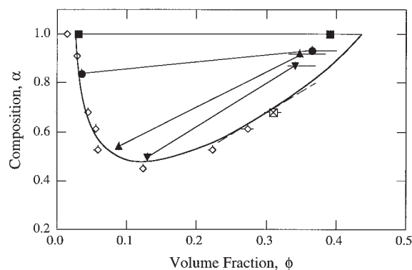
FIG. 3. Pairs of points (solid symbols) connected by straight lines (i.e., tie-lines) represent the two coexisting phases at T = 293.2 K for aqueous ternary solutions of \gamma_{\text{IVa}} and \gamma_s at various initial solution volume fractions and compositions ( \phi^0, \alpha^0 ) = (0.15, 0.57) ( \nabla ), (0.12, 0.68) ( \blacktriangle ), (0.06, 0.91) ( \bullet ), and (0.12, 1.0) ( \blacksquare ). The critical point ( \boxtimes ) and the equilibrium data points ( \diamond ) are deduced from the cloud-point curve data in Fig. 2. The solid curve is an eye guide for the binodal curve. The slope of the tie-line (dashed line) at the critical point is drawn as discussed in the text.
