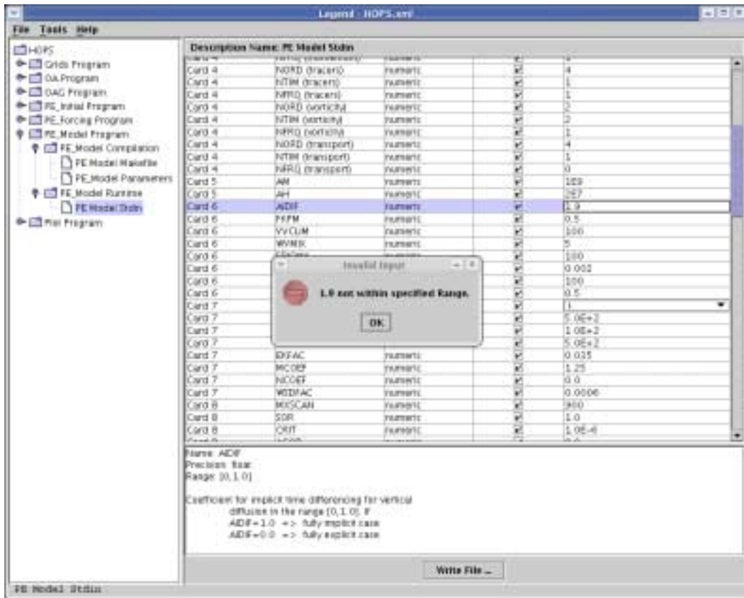
Fig. 16. Screen capture of GUI validating user input
