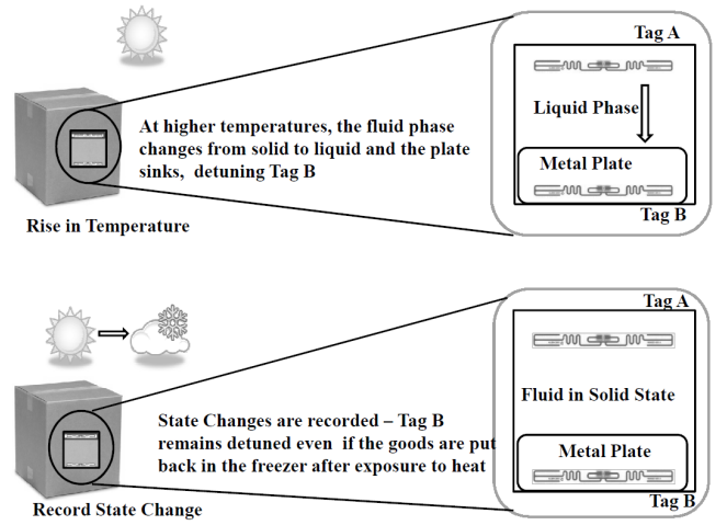
Fig. 4. Functional States of the temperature sensor
