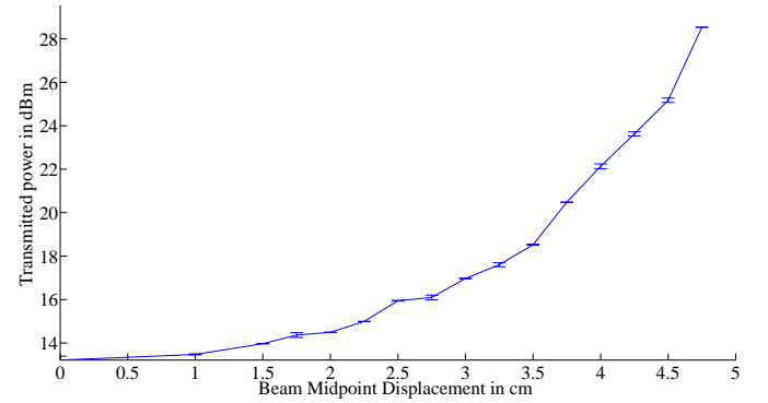
Fig. 7. Displacement vs. Threshold TX Power
