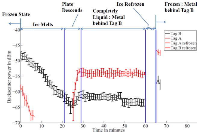
Fig. 5. Change in tag response with threshold violation for a reader-tag separation of 0.5 m
