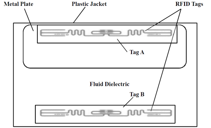
Fig. 3. Design of the temperature threshold sensor
