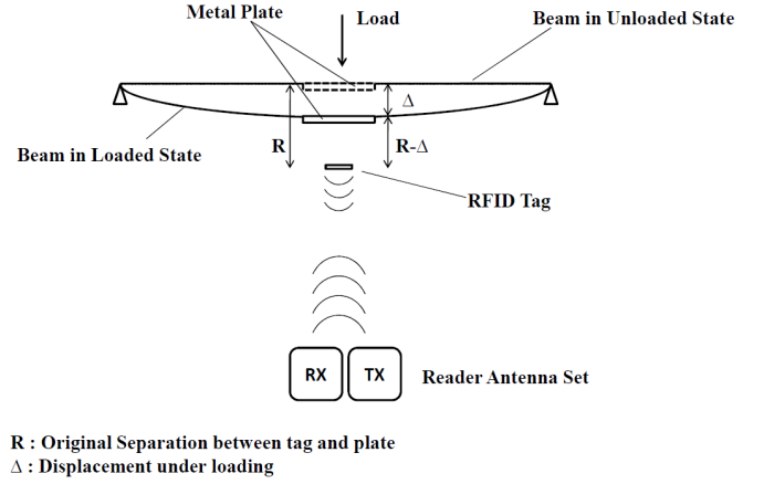
Fig. 6. Displacement Sensor Design
