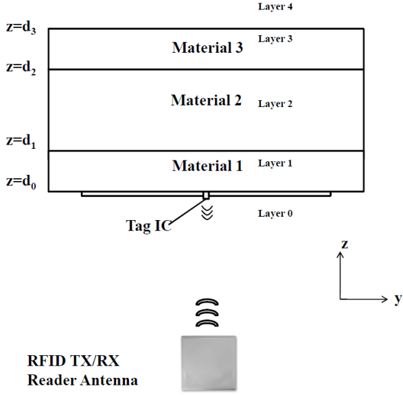
Fig. 2. RFID antenna on a 3-layer dielectric medium
