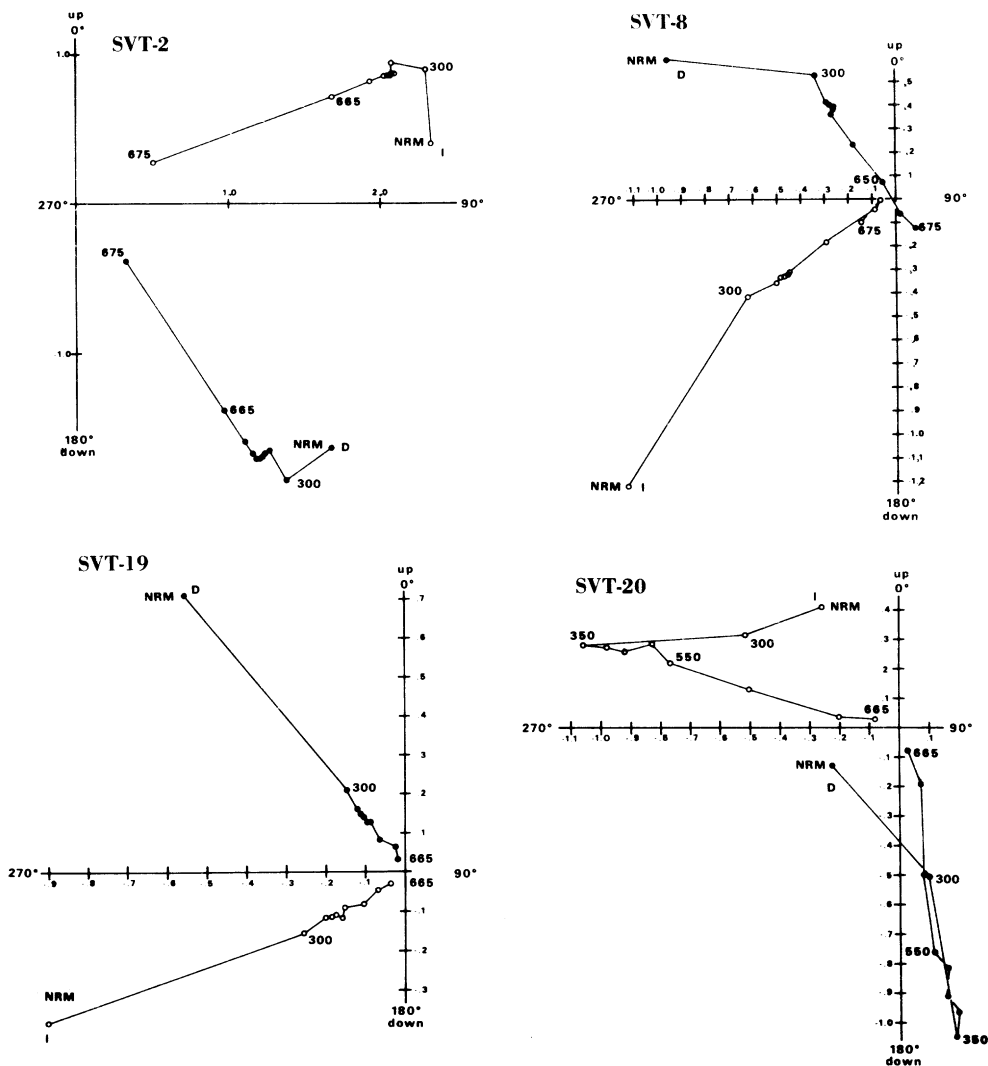
Figure 6. Vector demagnetization diagrams. Numbers along the axes refer to the magnetic intensity in units of 10^{-6} \text{ emu g}^{-1} (or \text{A m}^2 \text{ kg}^{-1} ). Paths labelled D (declination) show the horizontal projection into the bedding plane of the demagnetization path, and those labelled I (inclination) plot the vertical component against the horizontal. Although it is not strictly an orthogonal projection, an inclination curve plotted in this fashion directly shows the inclination and intensity of the remanence vector at each demagnetization point. Occasionally, a line will plot on this curve as part of a hyperbola. The sampling locality, Tiout, is at 30.35^\circ \text{ N} , 8.67^\circ \text{ W} .
