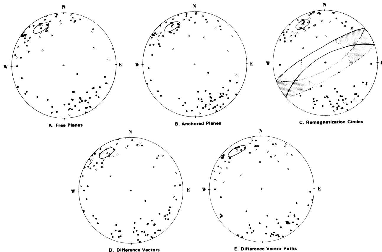
Figure 4. Comparison of pole directions for coplanar demagnetization data obtained with each of the five methods outlined on Fig. 2. Original magnetic data come from 96 Siberian samples collected at Zerinsky Mys. Open symbols indicate directions on the upper hemisphere (negative inclination). Open squares show the direction of the principal eigenvectors from the restricted data set ( MAD < 15^\circ ) along with their ovals of 95 per cent confidence. (C) also gives the 95 per cent boundaries along a girdle distribution in which both the primary and secondary magnetic directions lie; the shaded portion of the girdle corresponds to palaeoinclinations below 30^\circ north or south.
