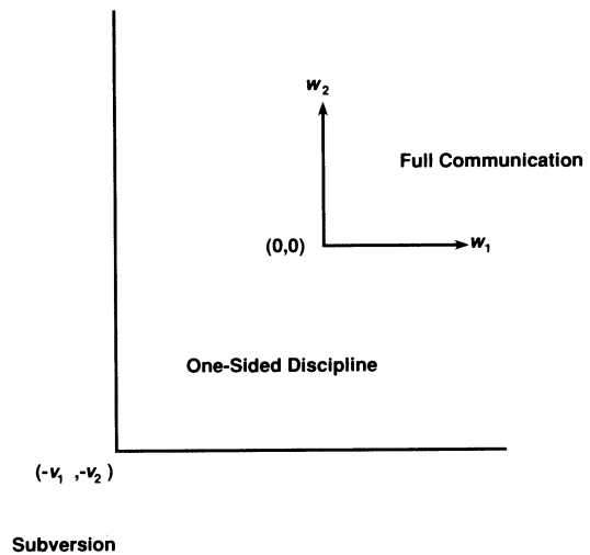
FIGURE 1. THE CASE v_1 > 0, v_2 > 0
