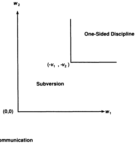
FIGURE 3. THE CASE v_1 < 0, v_2 < 0
