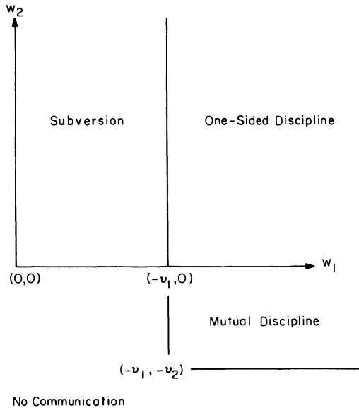
FIGURE 2. THE CASE v_1 < 0, v_2 > 0
