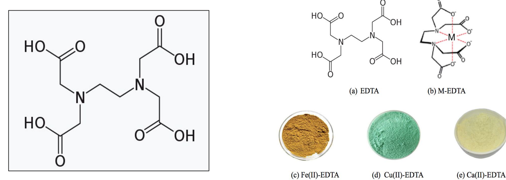
(a) EDTA in its natural form. (b) A metal particle inside a chelate. (c), (d), and (e): metal-EDTAs are extensively used as a chelating agent due to its ability to "sequester" metal ions.
