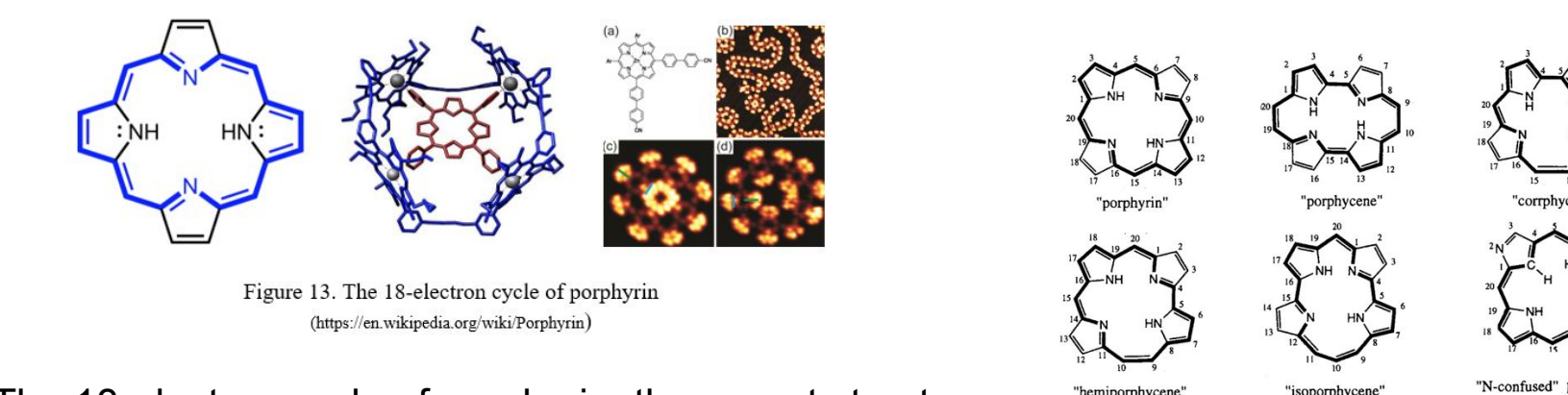
Figure 11. The 18-electron cycle of porphyrin (http://www.kjchem.com/porphyrin)
