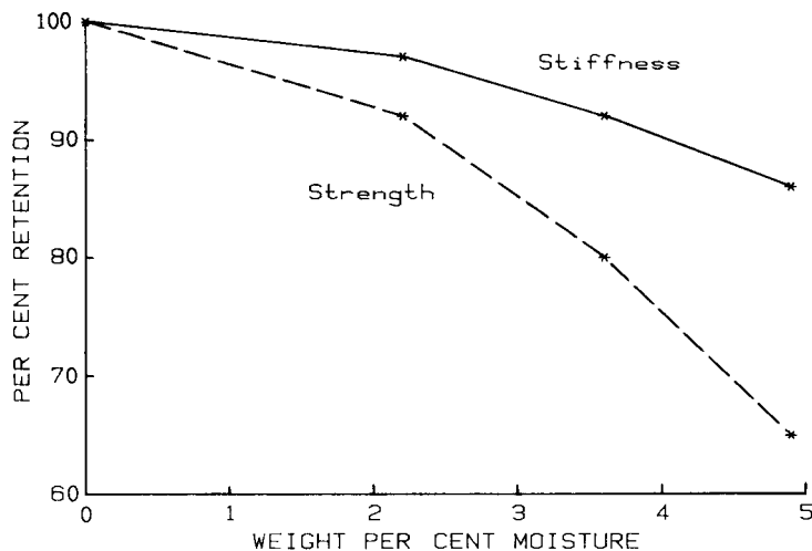
Figure 1 Transverse strength and stiffness retention of Kevlar 49/934 as a function of equilibrium moisture content at 25° C.
