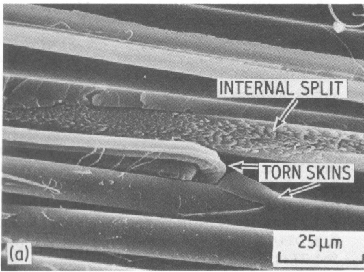
Figure 4 Transverse fracture with 5.3% moisture showing split filaments and skin-core failure.
