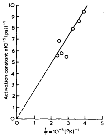
Fig. 7. Activation constant versus reciprocal temperature for drawn Nylon 6 fibers. Samples predesiccated and tested in dry N_2 atmosphere.
