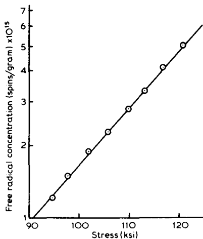
Fig. 6. Steady state free radical (spin) concentration versus stress for drawn Nylon 6 fibers. Samples predesiccated and tested in dry N_2 atmosphere at 60^\circ C .
