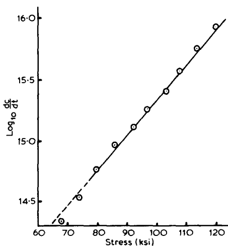
Fig. 4. Bond breakage rate versus stress during a constant-load-rate test. Sample predesiccated and tested in dry N_2 atmosphere at 80^\circ C .
