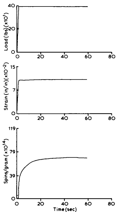
Fig. 2. Free radical production during a constant-load test of drawn Nylon 6 fibers. Samples predesiccated and tested in dry N_2 atmosphere at 25^\circ C .
