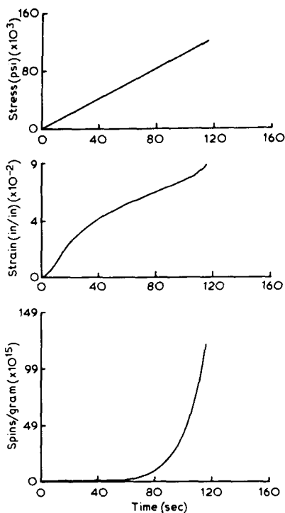
Fig. 3. Free radical production during a constant-load-rate test of drawn Nylon 6 fibers. Sample predesiccated and tested in dry N_2 atmosphere at 80^\circ C .
