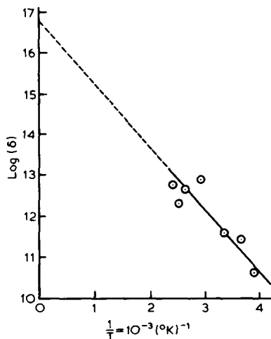
Fig. 8. Logarithm of pre-exponential factor \delta versus reciprocal temperature for drawn Nylon 6 fibers. Samples predesiccated and tested in dry N_2 atmosphere.
